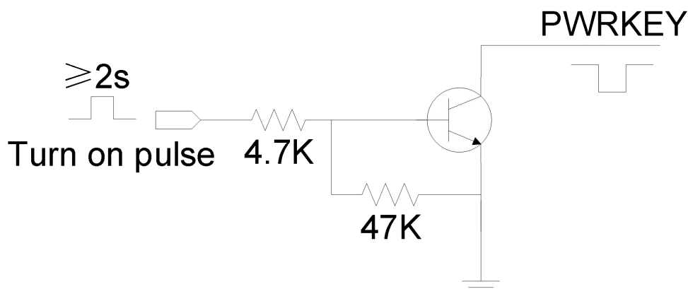
FIG. 6 Open set drive reference boot circuit
