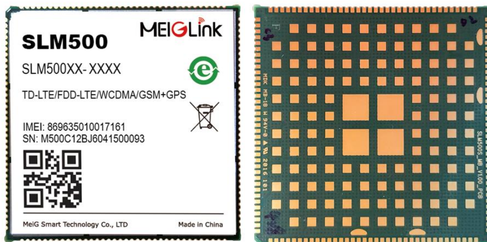
Fig6.1: Top and bottom views of modules
