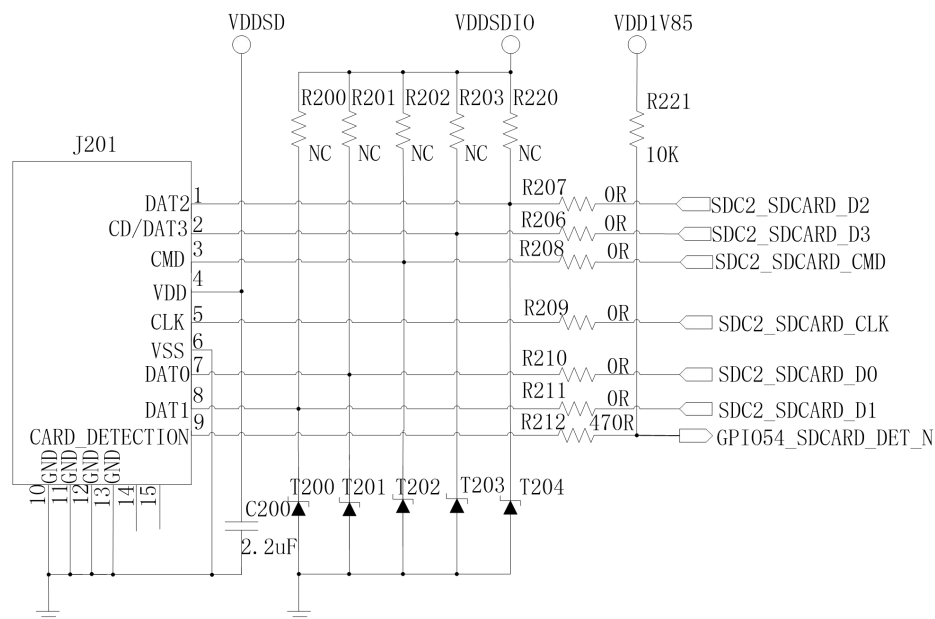
Fig4.30: SD interface circuit
