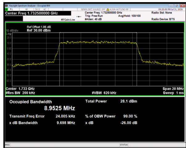
Band4 16QAM BW=10MHz Channel=20175 RB Size=50 Position=#0
