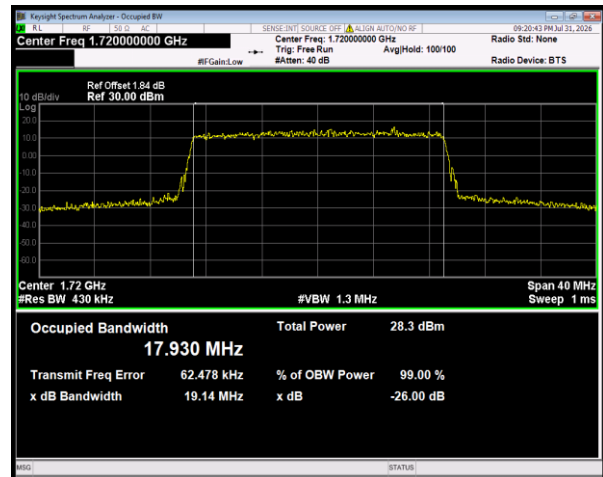
Band4 16QAM BW=20MHz Channel=20050 RB Size=100 Position=#0
