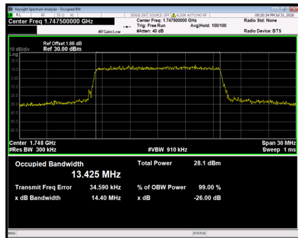
Band4 16QAM BW=15MHz Channel=20325 RB Size=75 Position=#0
