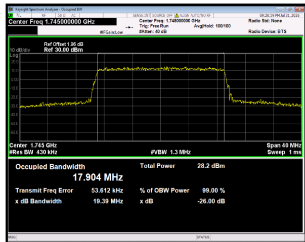
Band4 16QAM BW=20MHz Channel=20300 RB Size=100 Position=#0
