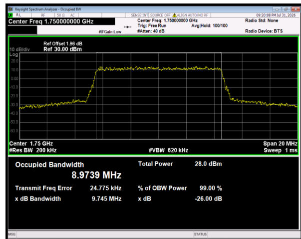
Band4 16QAM BW=10MHz Channel=20350 RB Size=50 Position=#0
