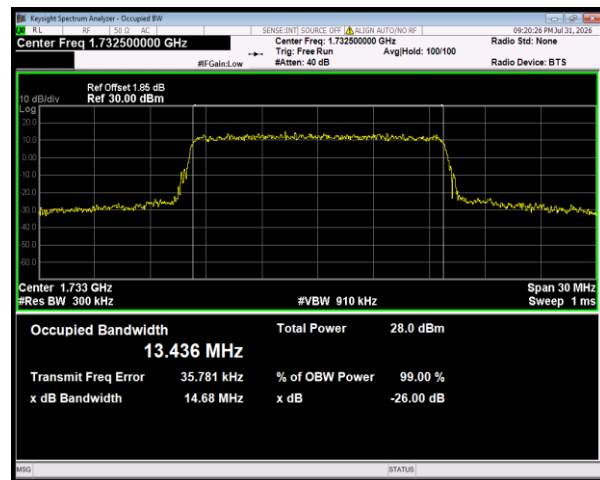
Band4 16QAM BW=15MHz Channel=20175 RB Size=75 Position=#0
