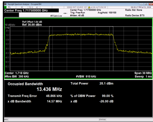
Band4 16QAM BW=15MHz Channel=20025 RB Size=75 Position=#0
