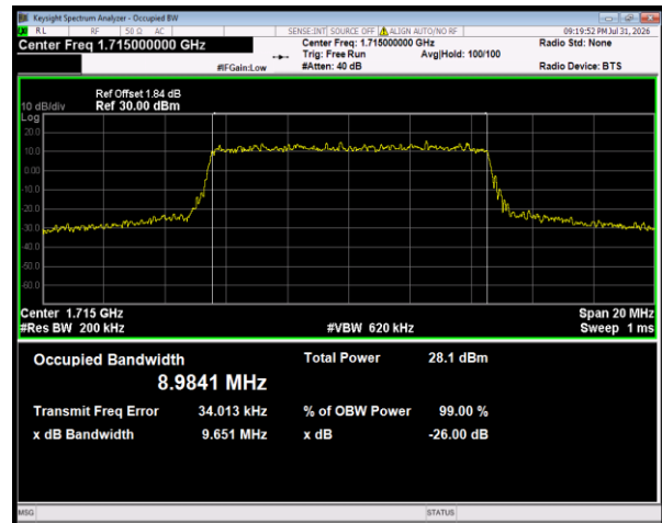
Band4 16QAM BW=10MHz Channel=20000 RB Size=50 Position=#0
