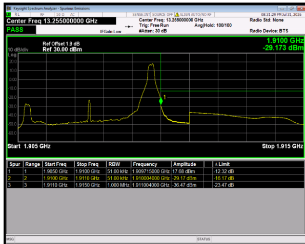
Band2 QPSK BW=5MHz HighChannel=19175 RB Size=1 Position=#Max
