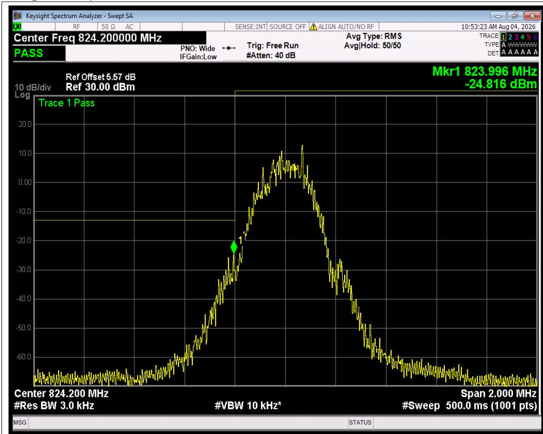
GSM850 Channel=128
