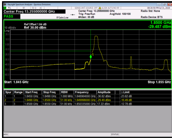
Band2 QPSK BW=5MHz LowChannel=18625 RB Size=1 Position=#0
