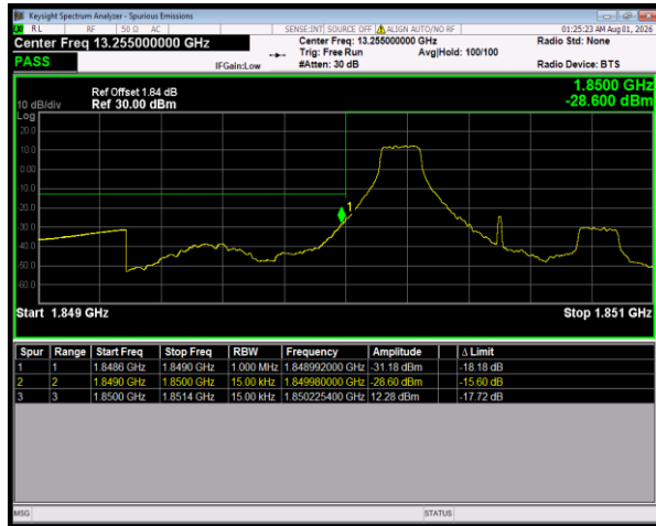
Band25 QPSK BW=1.4MHz LowChannel=26047 RB Size=1 Position=#0
