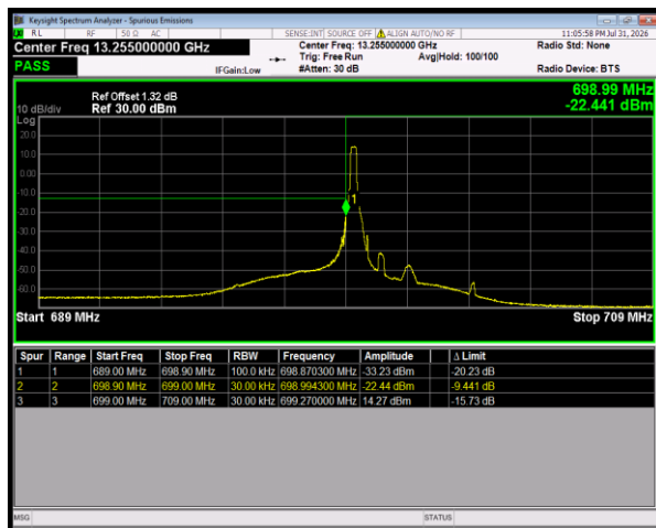
Band12 QPSK BW=1.4MHz LowChannel=23017 RB Size=1 Position=#0
