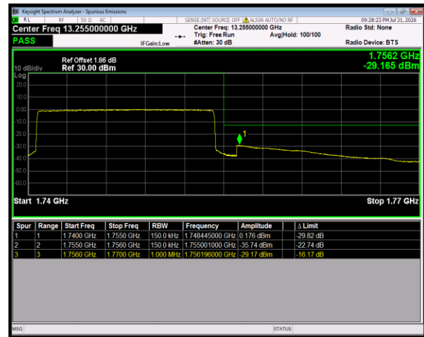
Band4 QPSK BW=15MHz HighChannel=20325 RB Size=75 Position=#0
