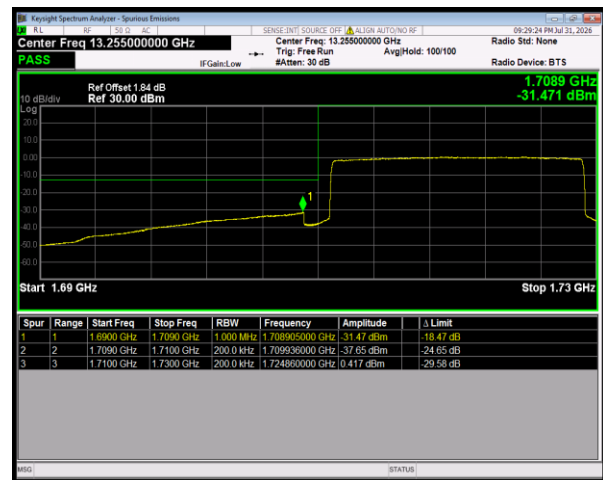
Band4 QPSK BW=20MHz LowChannel=20050 RB Size=100 Position=#0
