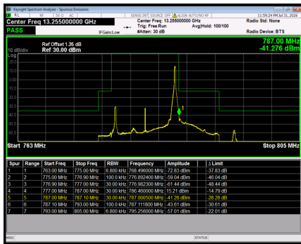
Band13 QPSK BW=10MHz HighChannel=23230 RB Size=1 Position=#Max
