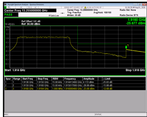
Band25 QPSK BW=1.4MHz HighChannel=26683 RB Size=6 Position=#0
