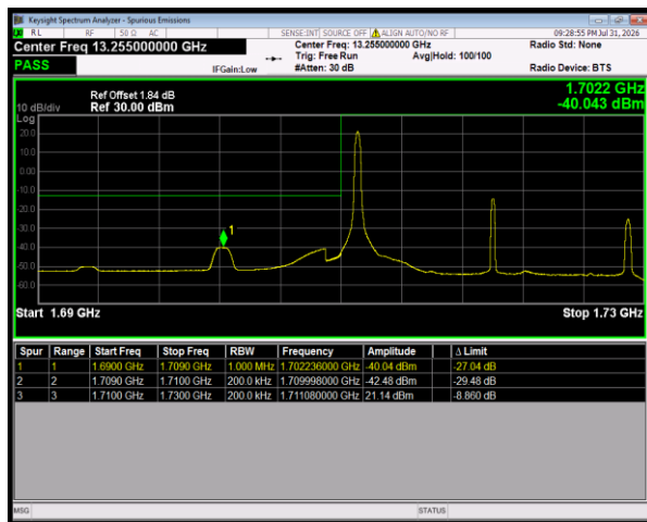
Band4 QPSK BW=20MHz LowChannel=20050 RB Size=1 Position=#0
