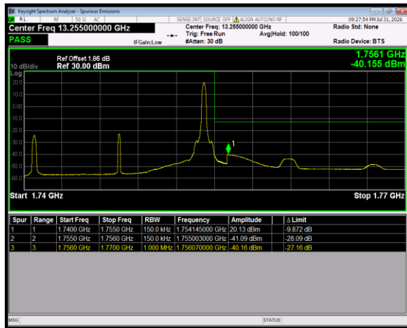
Band4 QPSK BW=15MHz HighChannel=20325 RB Size=1 Position=#Max
