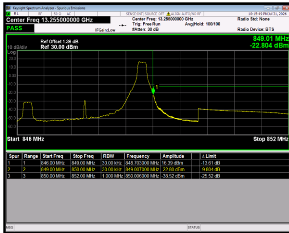
Band5 QPSK BW=3MHz HighChannel=20635 RB Size=1 Position=#Max
