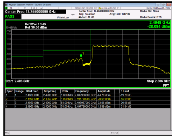
Band41 QPSK BW=5MHz LowChannel=39675 RB Size=25 Position=#0
