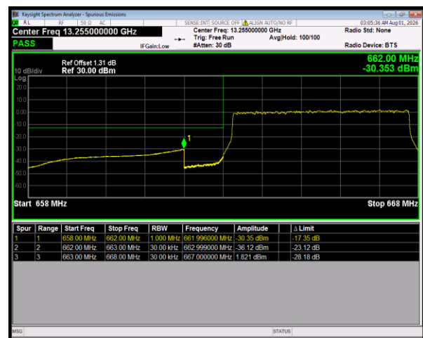
Band71 QPSK BW=5MHz LowChannel=133147 RB Size=25 Position=#0
