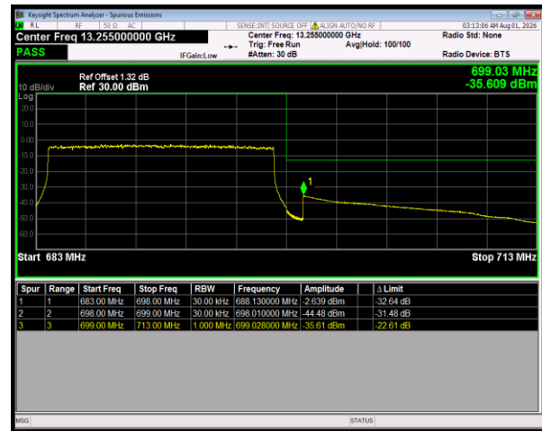
Band71 QPSK BW=15MHz HighChannel=133397 RB Size=75 Position=#0
