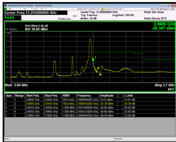
Band41 QPSK BW=5MHz HighChannel=41565 RB Size=1 Position=#Max
