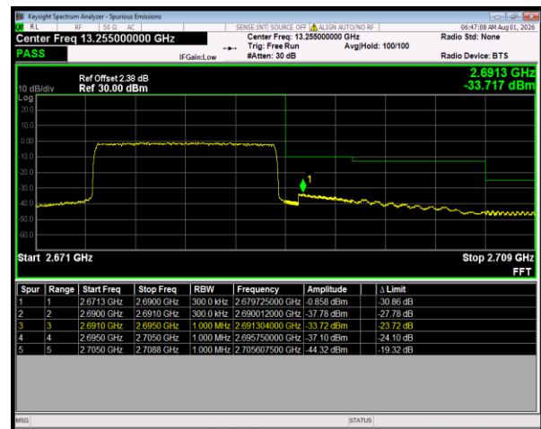
Band41 QPSK BW=15MHz HighChannel=41515 RB Size=75 Position=#0
