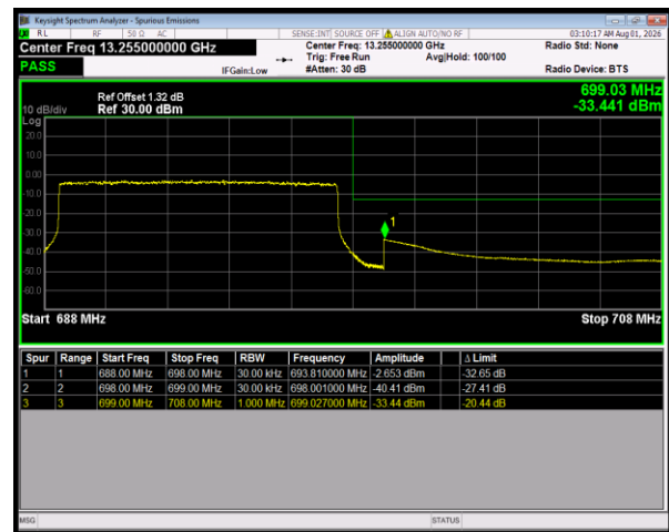
Band71 QPSK BW=10MHz HighChannel=133422 RB Size=50 Position=#0
