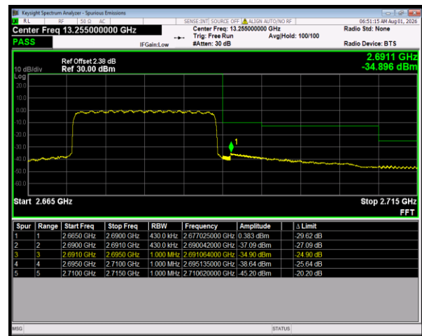
Band41 QPSK BW=20MHz HighChannel=41490 RB Size=100 Position=#0
