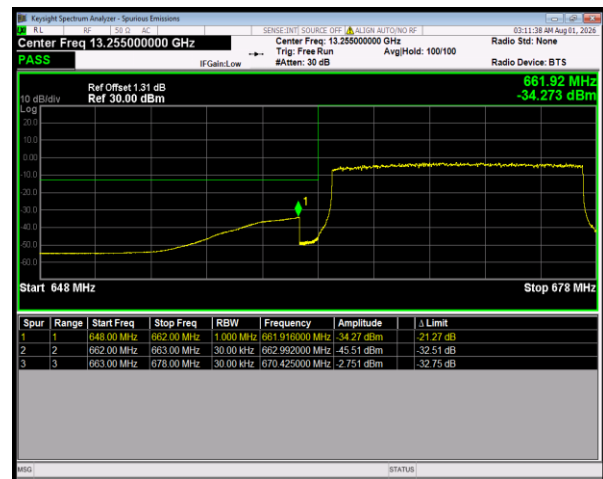
Band71 QPSK BW=15MHz LowChannel=133197 RB Size=75 Position=#0
