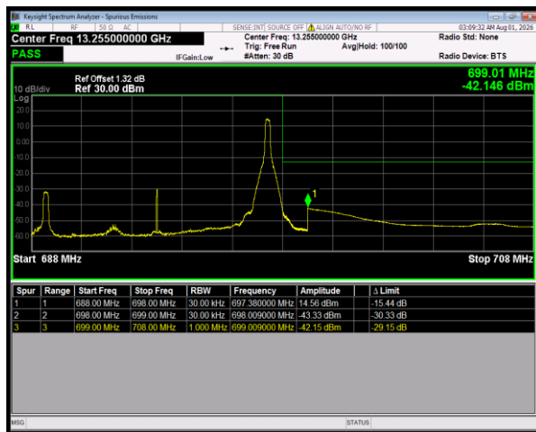
Band71 QPSK BW=10MHz HighChannel=133422 RB Size=1 Position=#Max
