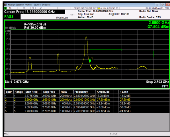
Band41 QPSK BW=10MHz HighChannel=41540 RB Size=1 Position=#Max
