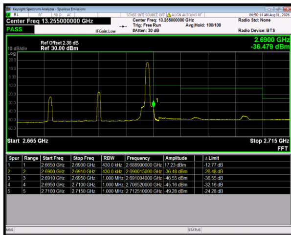
Band41 QPSK BW=20MHz HighChannel=41490 RB Size=1 Position=#Max
