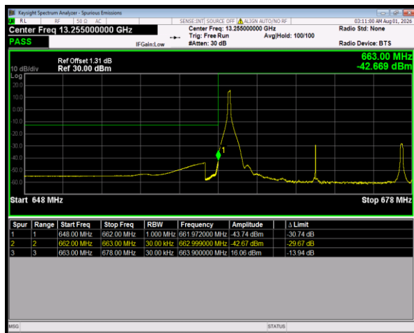
Band71 QPSK BW=15MHz LowChannel=133197 RB Size=1 Position=#0
