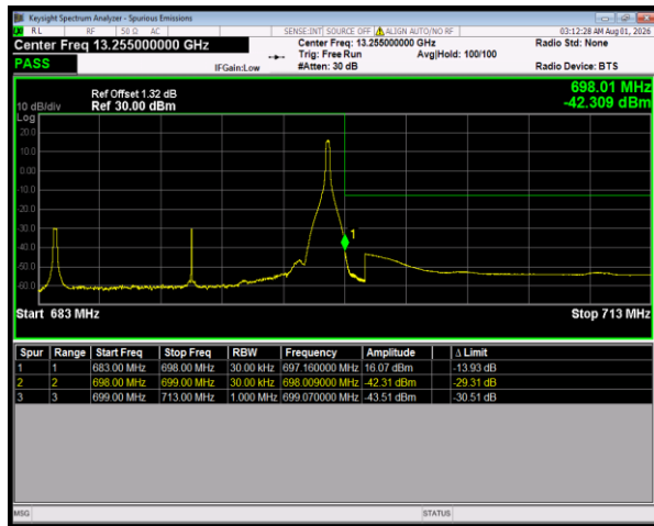
Band71 QPSK BW=15MHz HighChannel=133397 RB Size=1 Position=#Max
