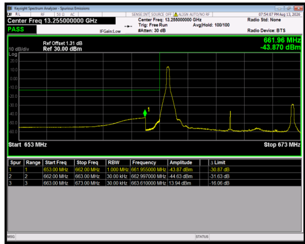
Band71 QPSK BW=10MHz LowChannel=133172 RB Size=1 Position=#0
