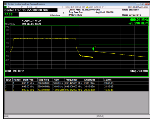
Band71 QPSK BW=5MHz HighChannel=133447 RB Size=25 Position=#0
