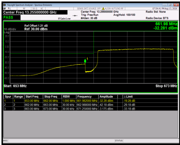
Band71 QPSK BW=10MHz LowChannel=133172 RB Size=50 Position=#0
