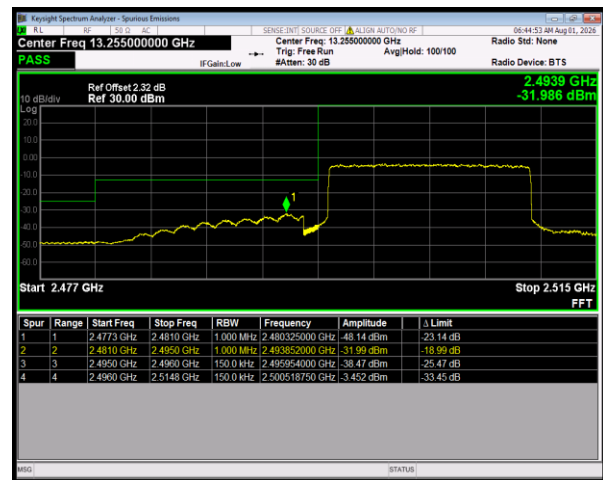
Band41 QPSK BW=15MHz LowChannel=39725 RB Size=75 Position=#0
