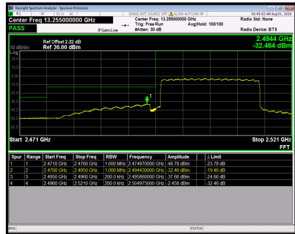
Band41 QPSK BW=20MHz LowChannel=39750 RB Size=100 Position=#0
