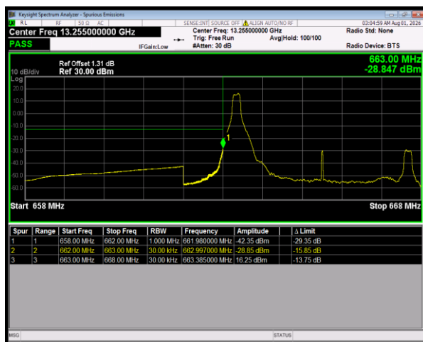
Band71 QPSK BW=5MHz LowChannel=133147 RB Size=1 Position=#0
