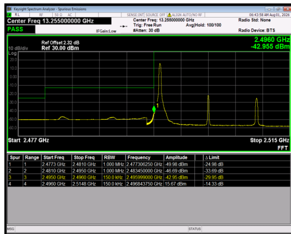
Band41 QPSK BW=15MHz LowChannel=39725 RB Size=1 Position=#0
