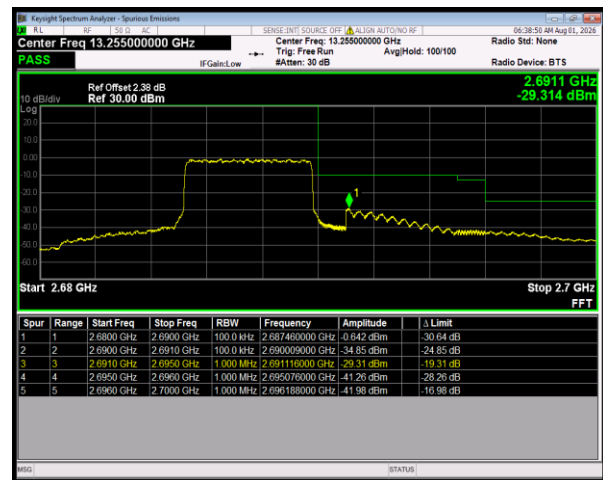
Band41 QPSK BW=5MHz HighChannel=41565 RB Size=25 Position=#0
