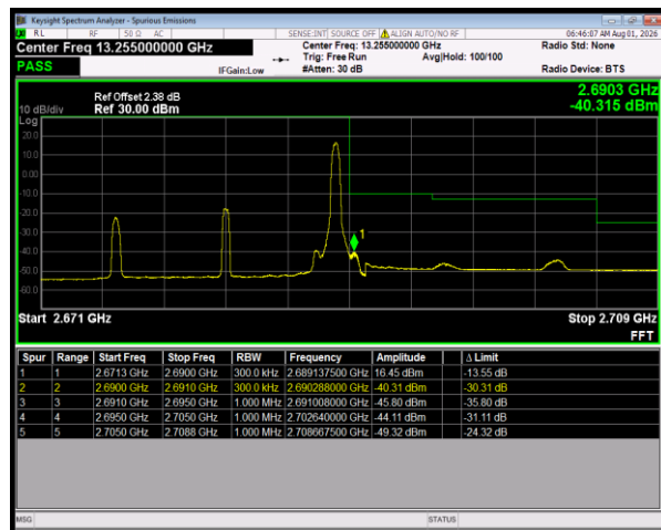
Band41 QPSK BW=15MHz HighChannel=41515 RB Size=1 Position=#Max
