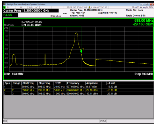
Band71 QPSK BW=5MHz HighChannel=133447 RB Size=1 Position=#Max
