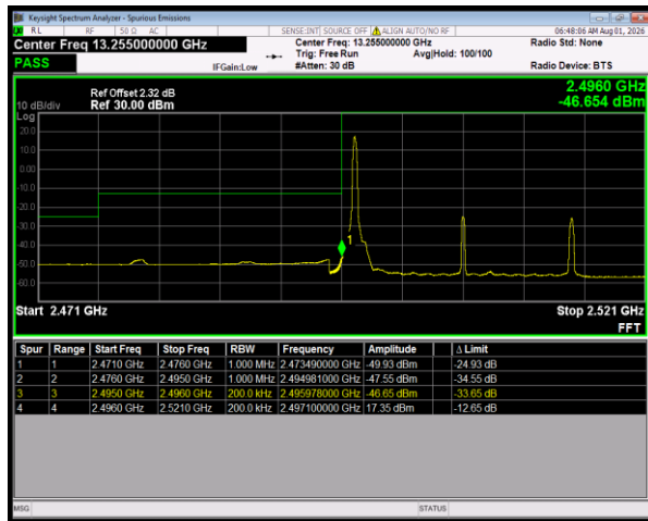
Band41 QPSK BW=20MHz LowChannel=39750 RB Size=1 Position=#0
