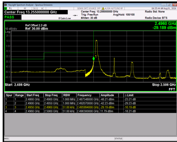
Band41 QPSK BW=5MHz LowChannel=39675 RB Size=1 Position=#0
