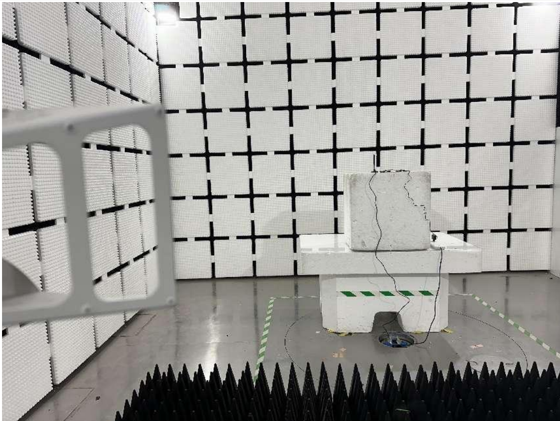
Above 1GHz-RF
