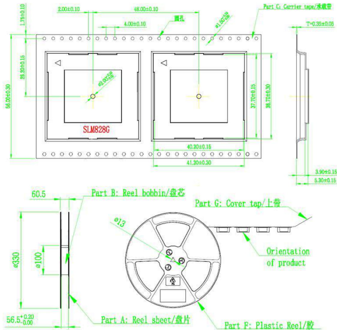
Figure 36 Package diagram
