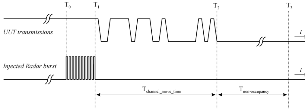
Figure 9: Channel Closing Transmission Time, Channel Move Time and Non-Occupancy Period
