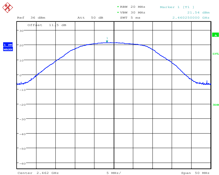
Fig.30 Peak Conducted Output Power CH11, 11g, Rate9
