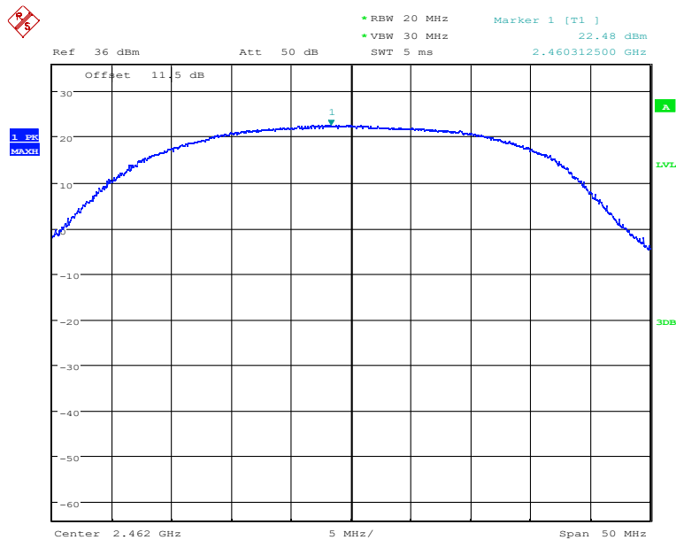
Fig.54 Peak Conducted Output Power CH11, 11n, MCS1
