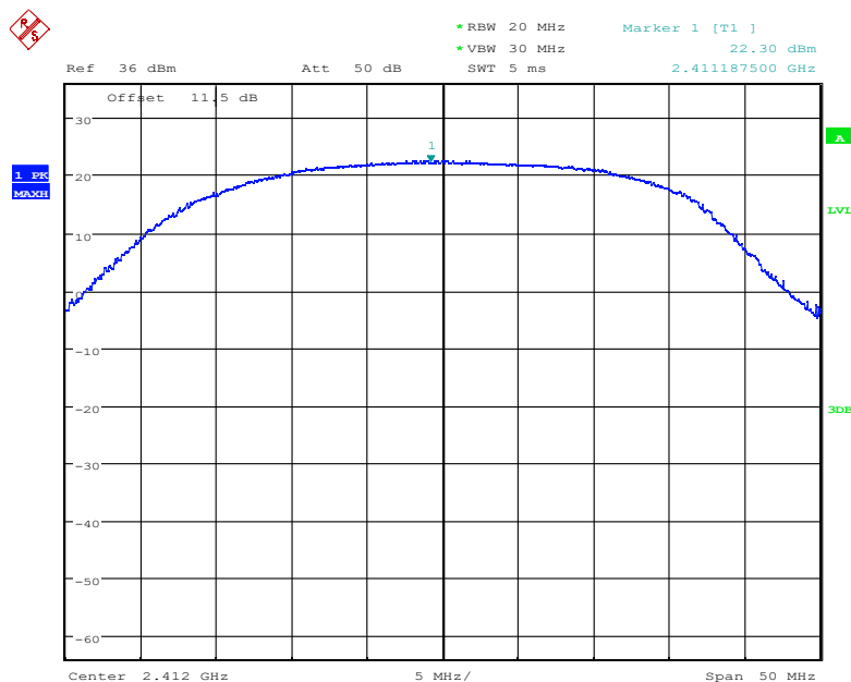
Fig.14 Peak Conducted Output Power CH1, 11g, Rate9
