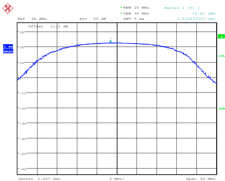
Fig.48 Peak Conducted Output Power CH6, 11n, MCS3
