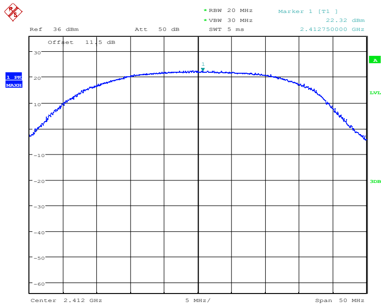
Fig.38 Peak Conducted Output Power CH1, 11n, MCS1
