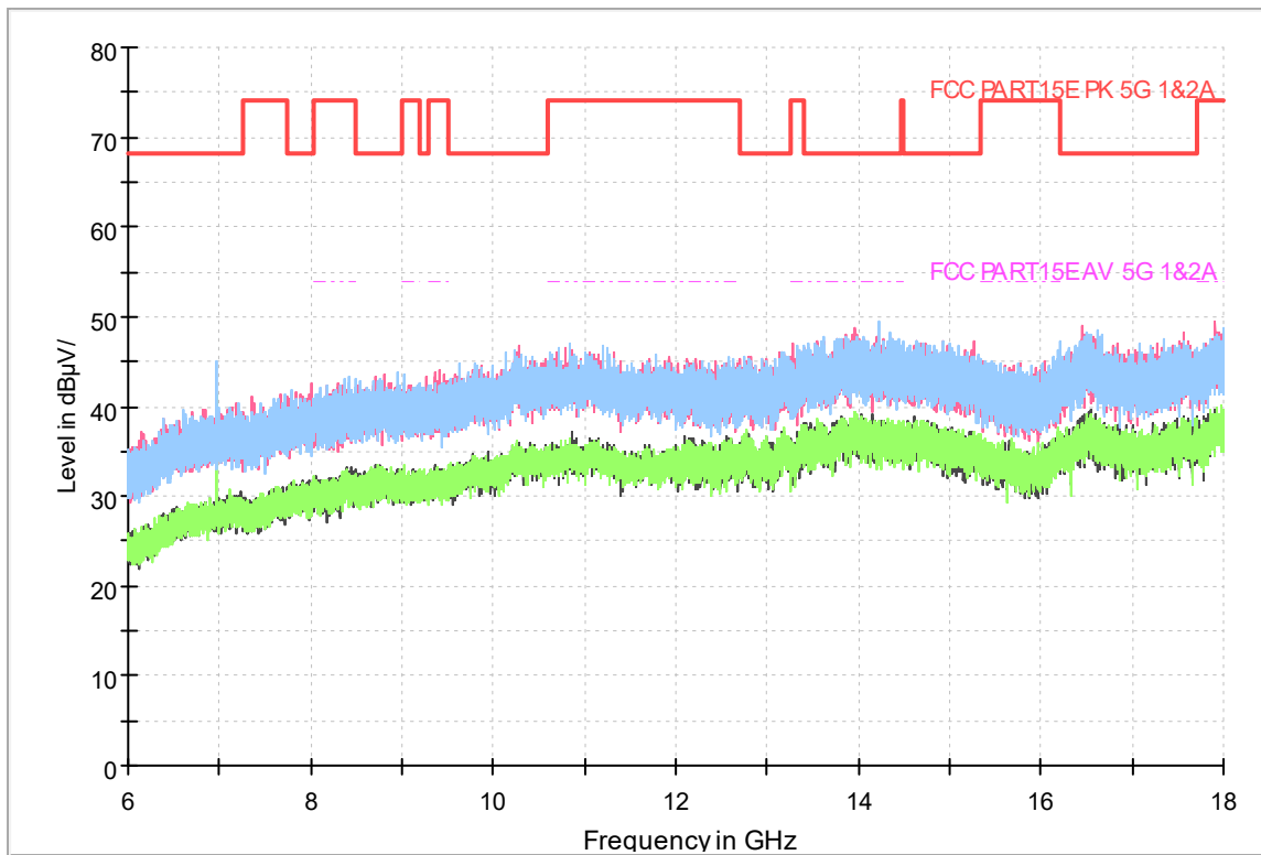
Fig.351 Radiated emission: 802.11ac(20M),CH40, 6GHz-18GHz
