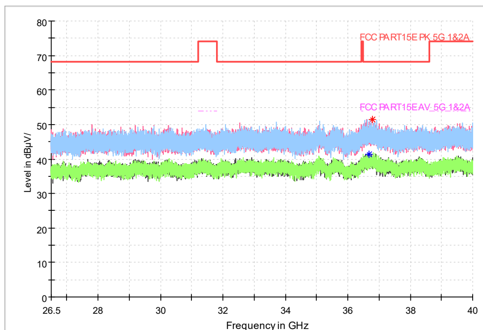
Fig.403 Radiated emission: 802.11ac(40M),CH162, 26.5 GHz – 40GHz
