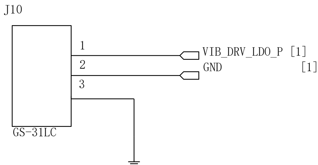
Figure 4.29: motor interface circuit
