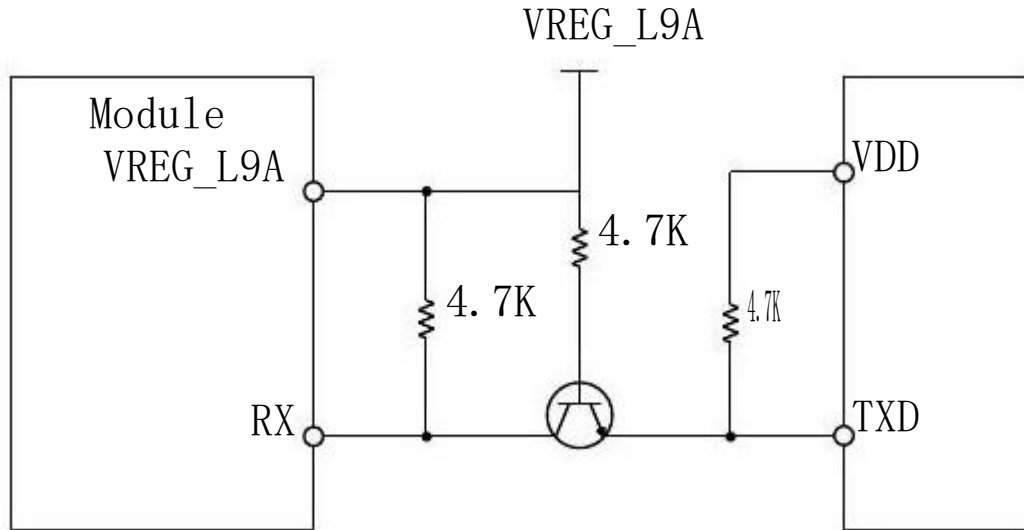
Figure 4.14 : RX Connection Diagram
