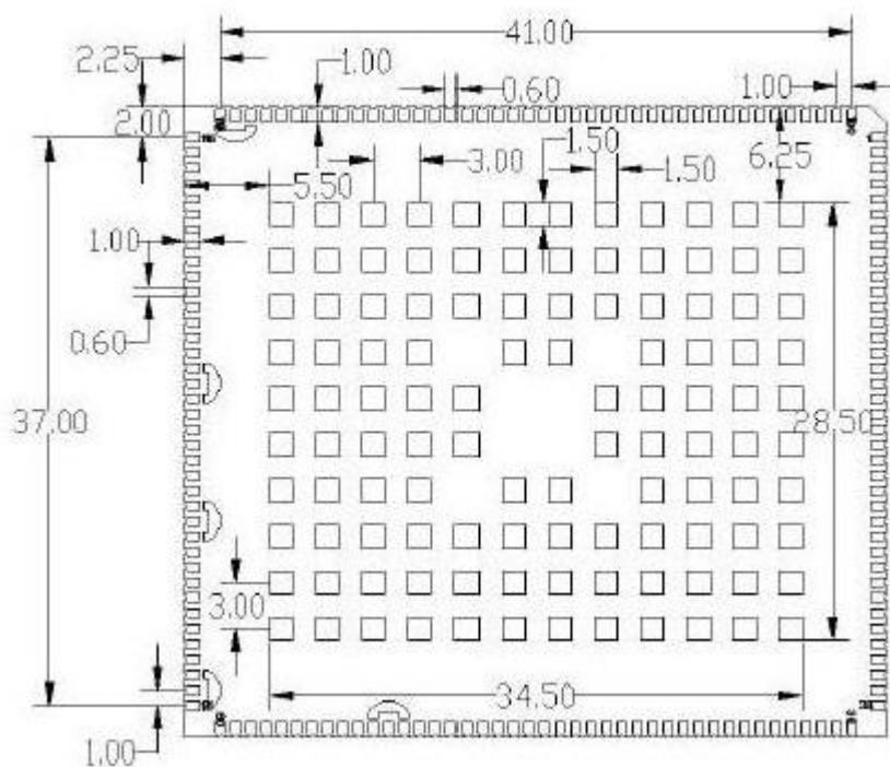
Figure 3.2 : Module 3D Dimensions (Unit: mm)
