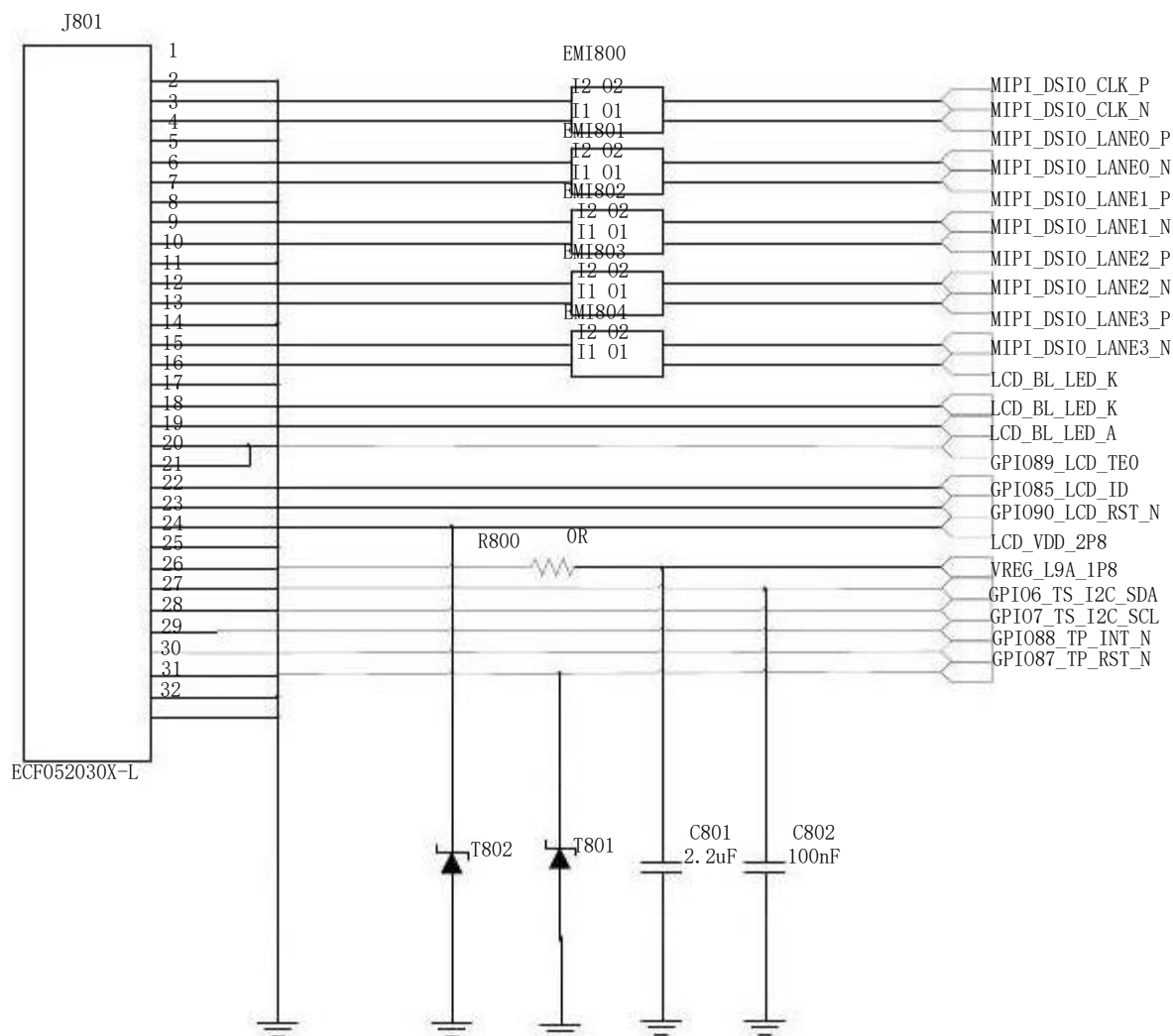
Figure 4.15 : LCD Interface Circuit
