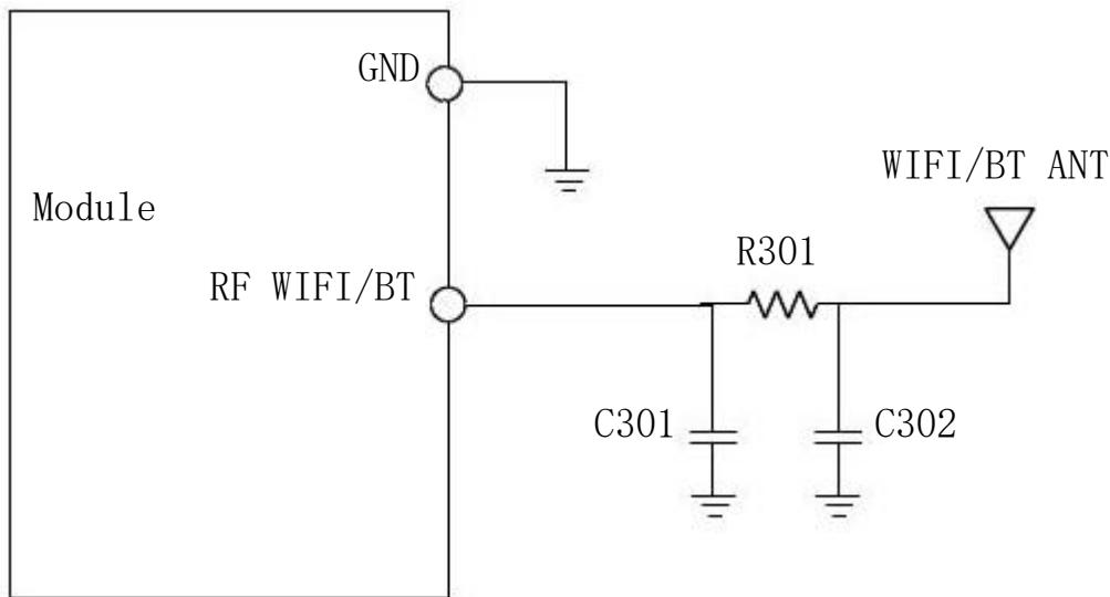
Figure 4.36 : WIFI_BT antenna interface simplified connection circuit
