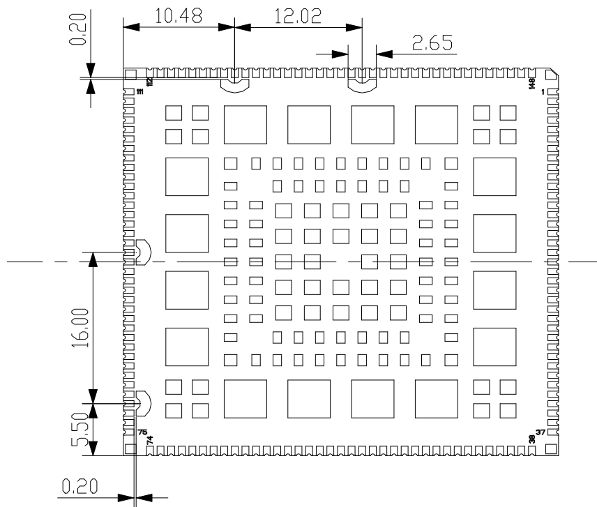
Figure 3.2: Three-dimensional dimensions of the module (unit: mm)
