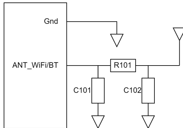
Figure 4.32: WIFI_BT antenna interface simplified connection
