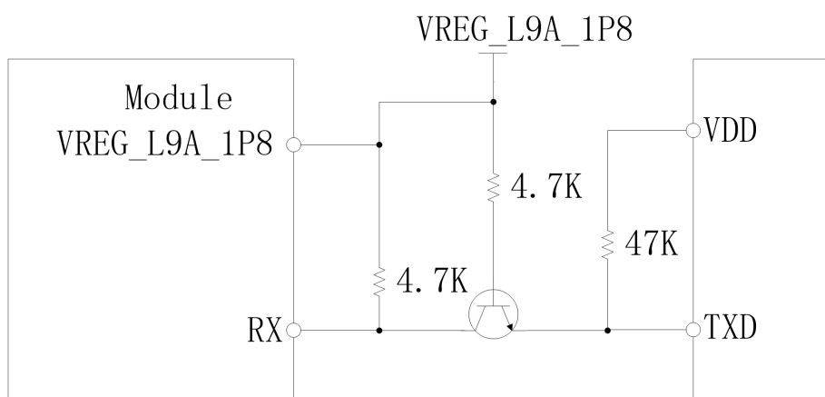
Figure 4.13: Schematic diagram of RX level conversion
