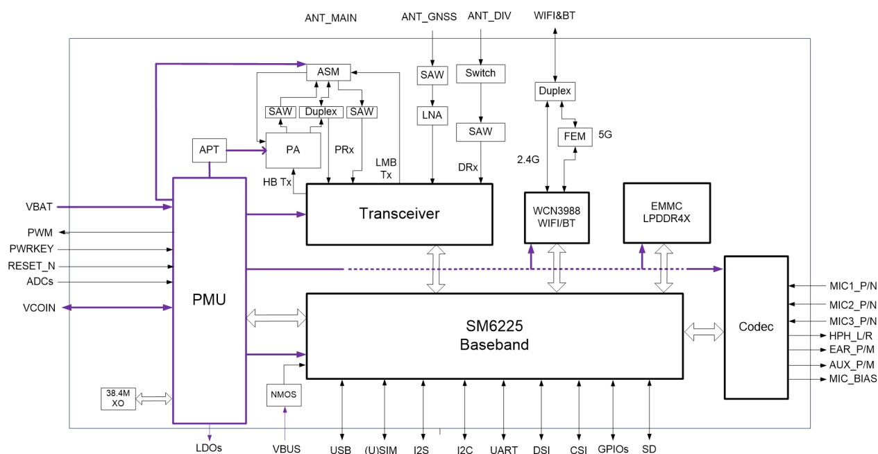
Figure 2.1: Block diagram of module functions
