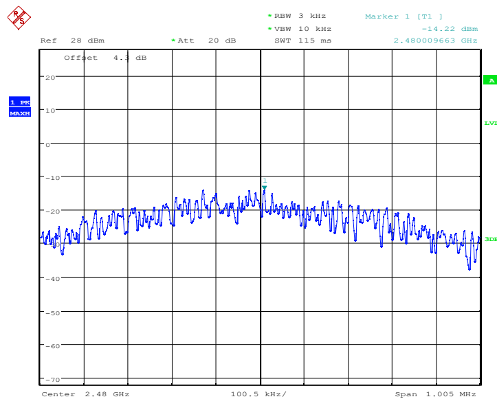
Fig.2 Power spectral density: 1M CH19 PSD/3KHz
