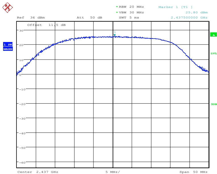
Fig.24 Peak Conducted Output Power CH6, 11g, Rate18
