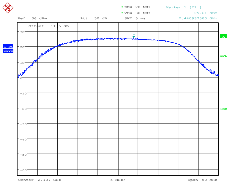
Fig.26 Peak Conducted Output Power CH6, 11g, Rate36
