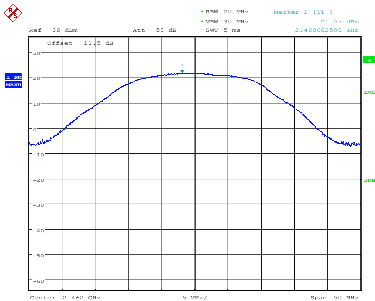
Fig.32 Peak Conducted Output Power CH11, 11g, Rate18
