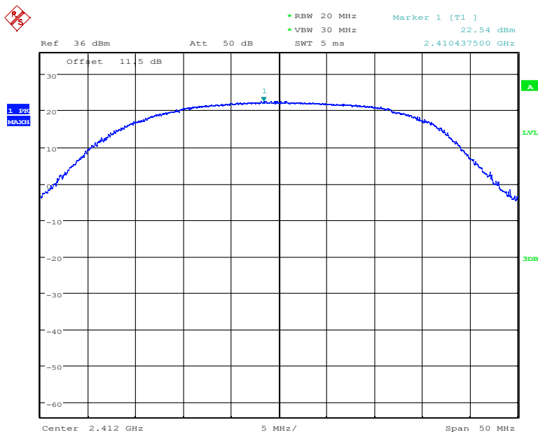
Fig.18 Peak Conducted Output Power CH1, 11g, Rate36
