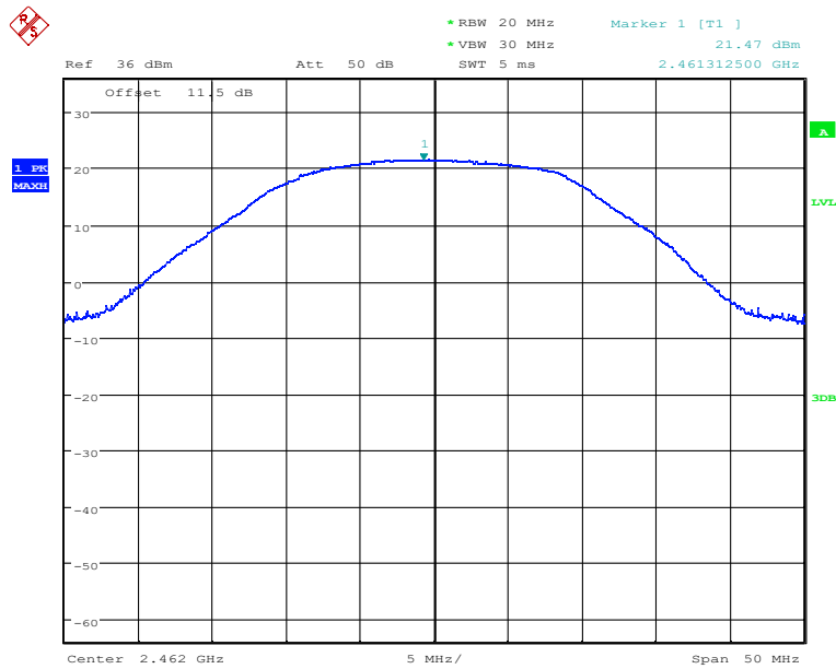
Fig.34 Peak Conducted Output Power CH11, 11g, Rate36
