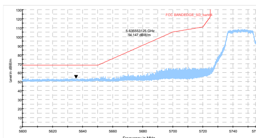
802.11ac VHT20-Channel 149: Peak
