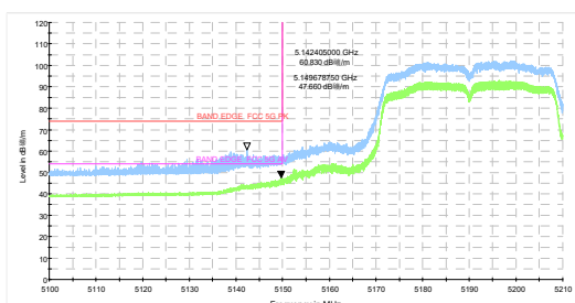
802.11ac VHT40-Channel 38: Peak + Average
