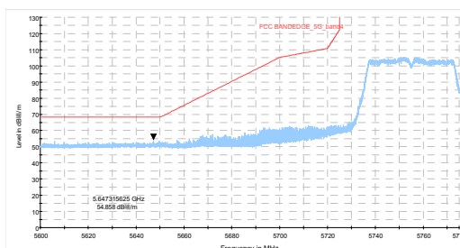
802.11ac VHT40-Channel 151: Peak
