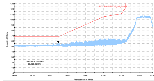
802.11a-Channel 149: Peak
