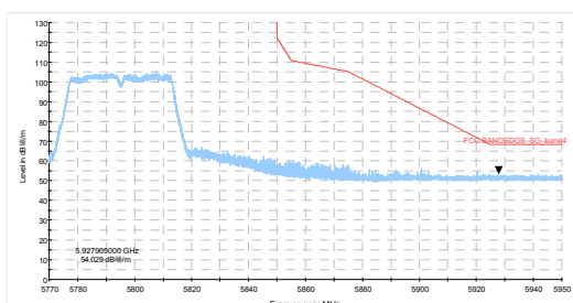
802.11ac VHT40-Channel 159: Peak
