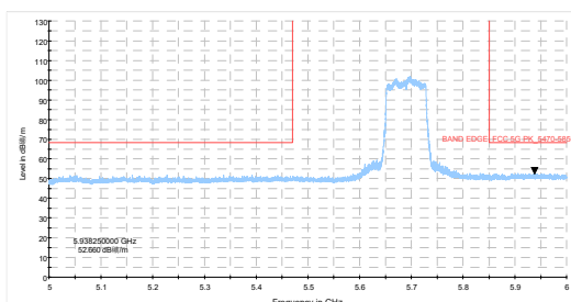
802.11ac VHT80- Channel 138: Peak
