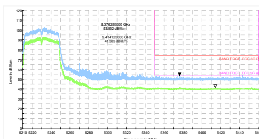
802.11ac VHT40-Channel 46: Peak + Average
