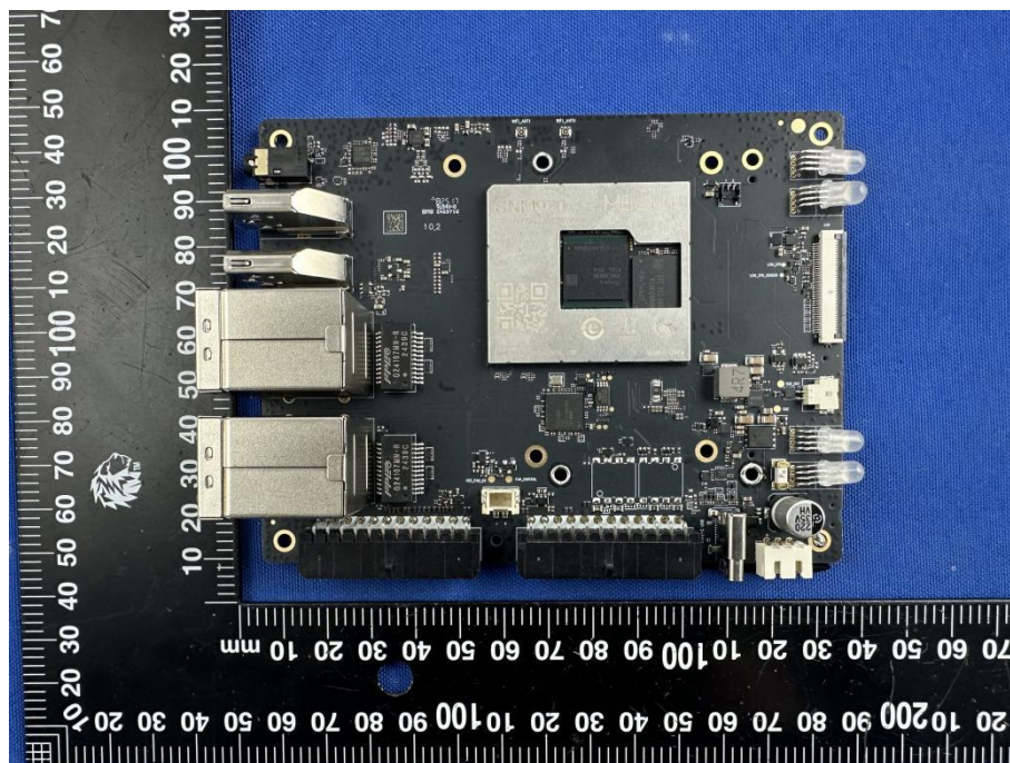
Host Board
