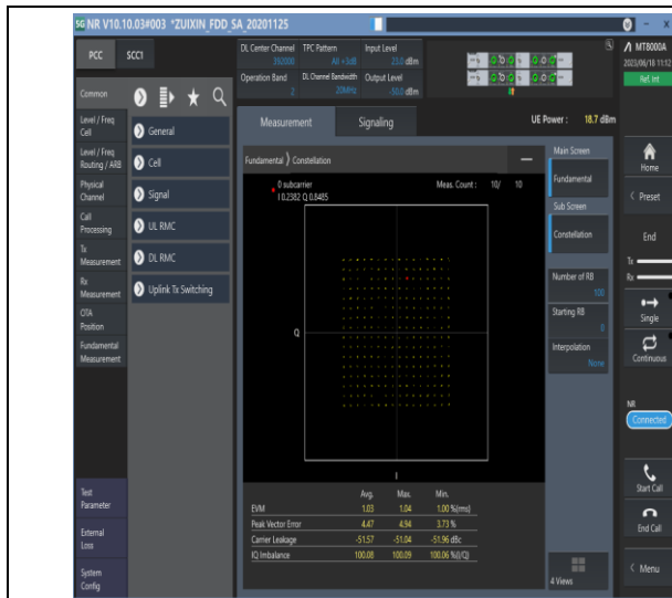
1-N2-PC3-15-20-M-5-DFT-256QAM-Outer_Full-100 @0-Ant3-see graph-PASS
