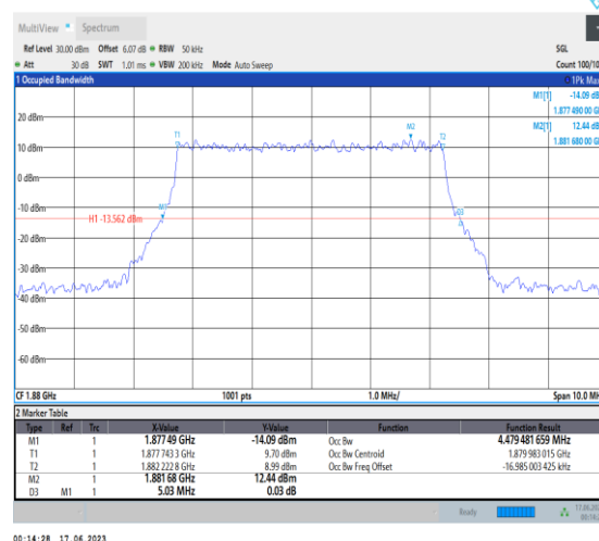
1-N2-PC3-15-5-M-3-DFT-16QAM-Outer_Full-25@0-A Ant3-4.479-5.030-≤5-PASS
