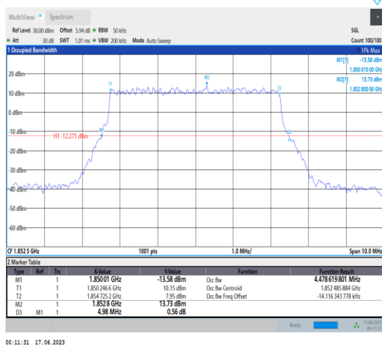
1-N2-PC3-15-5-L-1-DFT-QPSK-Outter_Full-25@0-An t3-4.479-4.980-≤5-PASS
