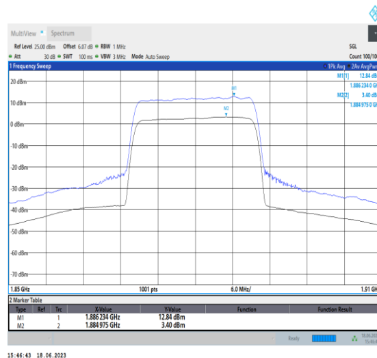
1-N2-PC3-15-20-M-2-CP-256QAM-Outer_Full-106 @0-Ant3-9.44-100%-0.00-9.44-PASS-≤13
