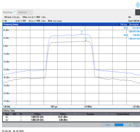
1-N2-PC3-15-20-M-1-DFT-256QAM-Outer_Full-100 @0-Ant3-8.53-100%-0.00-8.53-PASS-≤13
