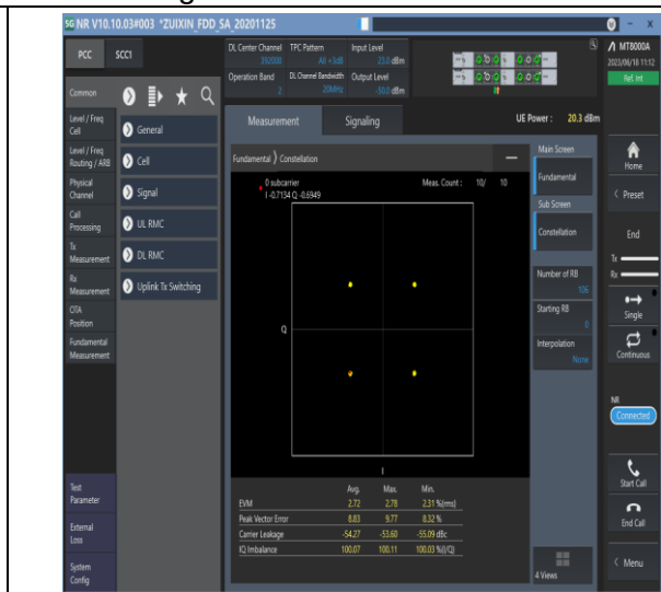
1-N2-PC3-15-20-M-6-CP-QPSK-Outer_Full-106@0- Ant3-see graph-PASS
