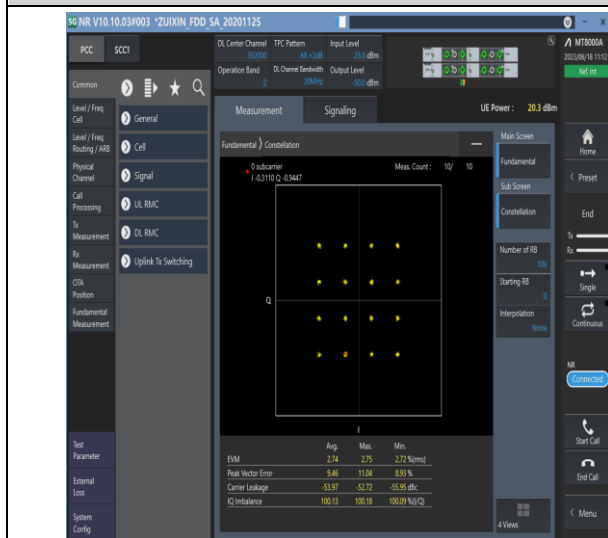
1-N2-PC3-15-20-M-7-CP-16QAM-Outer_Full-106@0- Ant3-see graph-PASS
