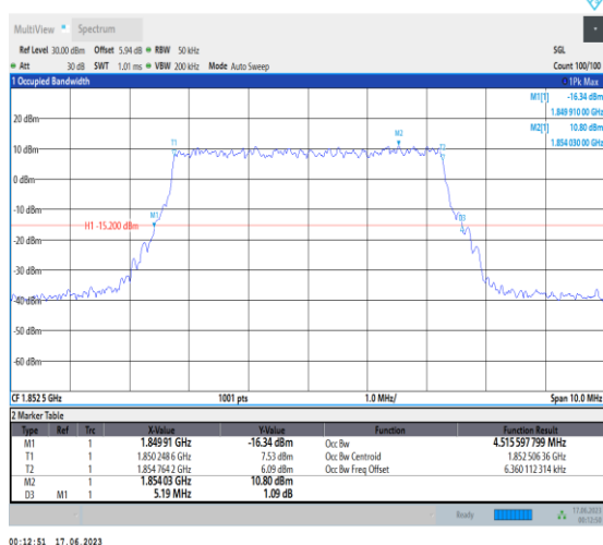
1-N2-PC3-15-5-L-7-CP-16QAM-Outer_Full-25@0-Ant3-4.516-5.190-≤5-PASS
