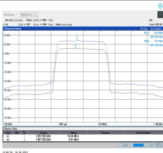
1-N2-PC3-15-20-L-1-DFT-256QAM-Outer_Full-100@ 0-Ant3-8.83-100%-0.00-8.83-PASS-≤13
