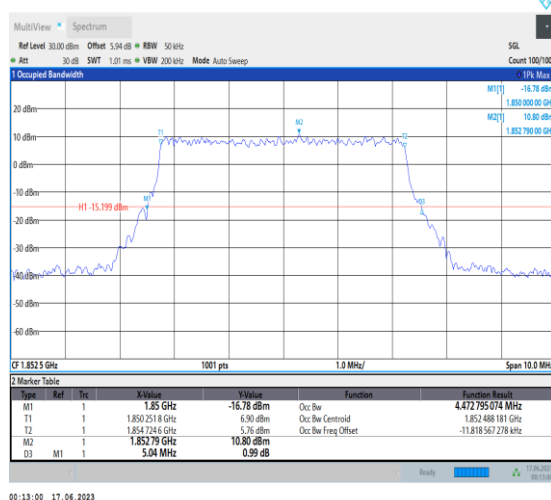
1-N2-PC3-15-5-L-8-CP-64QAM-Outer_Full-25@0-Ant3-4.473-5.040-≤5-PASS
