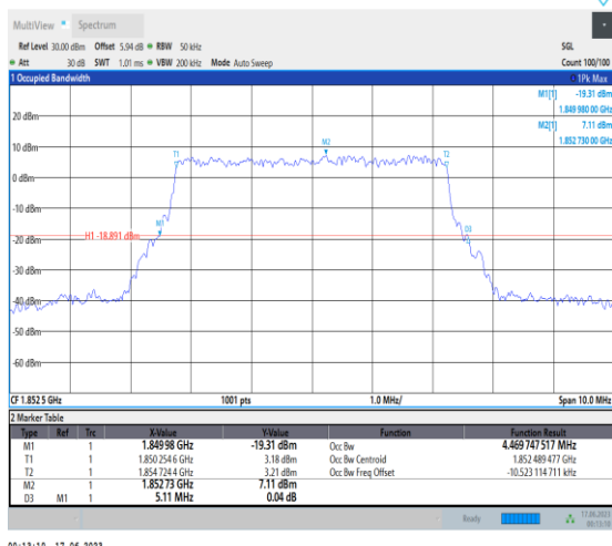
1-N2-PC3-15-5-L-9-CP-256QAM-Outer_Full-25@0-A nt3-4.47-5.110-≤5-PASS
