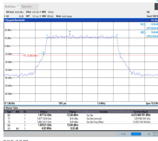
1-N2-PC3-15-5-M-1-DFT-QPSK-Outer_Full-25@0-A nt3-4.472-4.920-≤5-PASS
