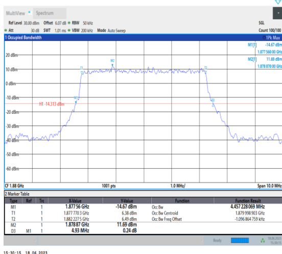
1-N2-PC3-15-5-M-2-DFT-PI2BPSK-Outer_Full-25@0-A -Ant3-4.457-4.930-≤5-PASS
