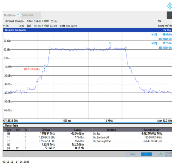
1-N2-PC3-15-5-L-3-DFT-16QAM-Outter_Full-25@0- Ant3-4.482-5.100-≤5-PASS
