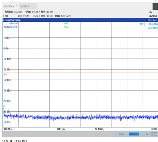
1-N2-PC3-15-20-M-1-DFT-PI2BPSK-Inner_1RB_Lef t-1@1-30-1000-Ant3-32.91--58.32--23-PASS
