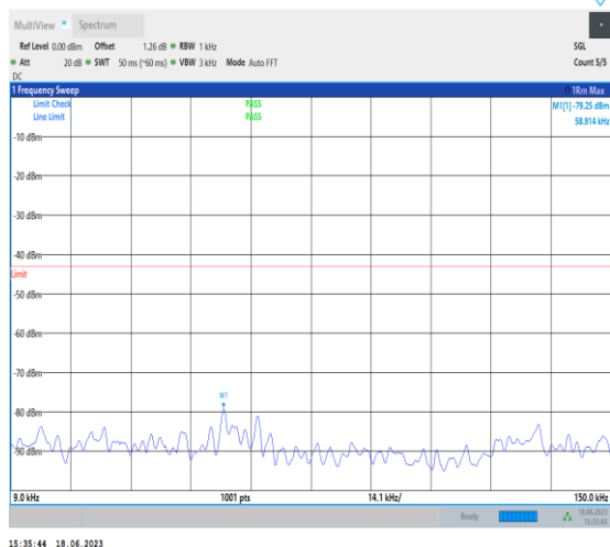
1-N2-PC3-15-20-L-1-DFT-PI2BPSK-Inner_1RB_Left -1@1-0.009-0.15-Ant3-0.06--79.25--43-PASS
