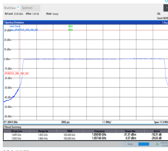
1-N2-PC3-15-10-L-6-CP-QPSK-Outer_Full-52@0-Ant3-1-seegraph-PASS-see graph
