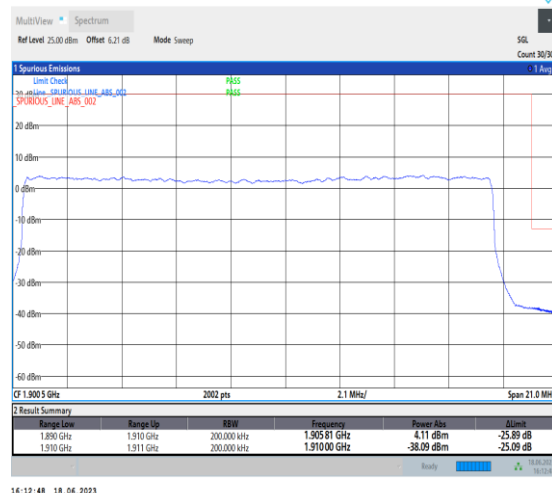
1-N2-PC3-15-20-H-3-DFT-PI2BPSK-Outer_Full-100@0-Ant3-1-seegraph-PASS-see graph
