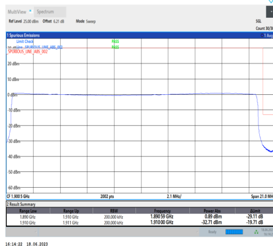
1-N2-PC3-15-20-H-6-CP-QPSK-Outer_Full-106@0-Ant3-1-seegraph-PASS-see graph
