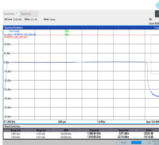
1-N2-PC3-15-15-H-3-DFT-PI2BPSK-Outer_Full-75@0-Ant3-1-seegraph-PASS-see graph
