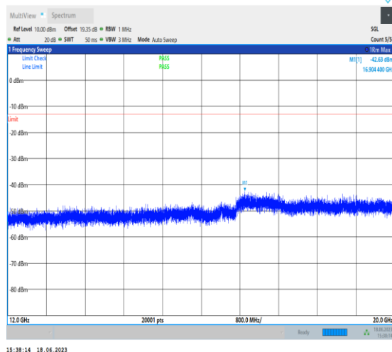
1-N2-PC3-15-20-H-1-DFT-PI2BPSK-Inner_1RB_Left- 1@1-12000-20000-Ant3-16904.40--42.63--13-PASS
