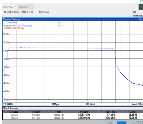
1-N2-PC3-15-5-H-6-CP-QPSK-Outer_Full-25@0-A nt3-1-seegraph-PASS-see graph
