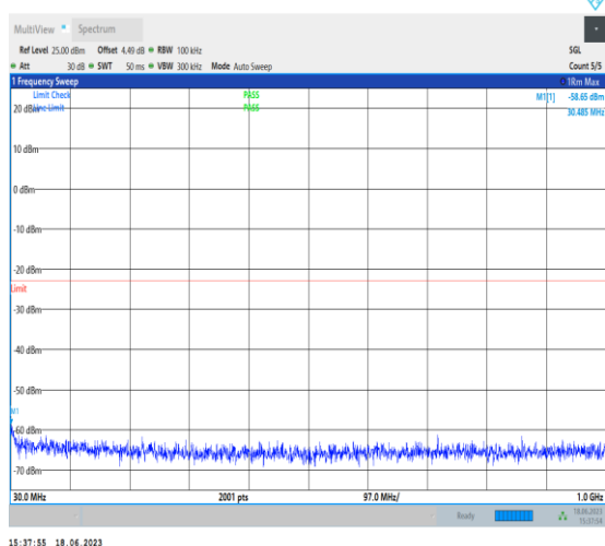
1-N2-PC3-15-20-H-1-DFT-PI2BPSK-Inner_1RB_Lef t-1@1-30-1000-Ant3-30.49--58.65--23-PASS
