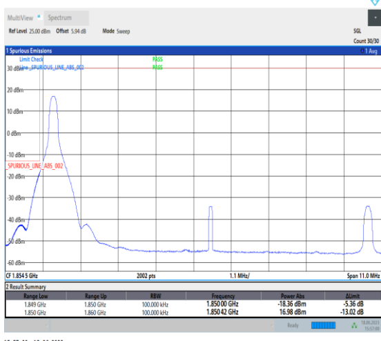
1-N2-PC3-15-10-L-4-CP-QPSK-Edge_1RB_Left-1@0-Ant3-1-seegraph-PASS-see graph
