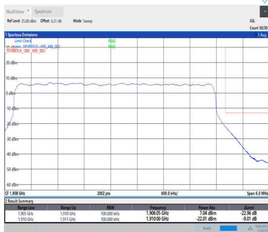
1-N2-PC3-15-5-H-3-DFT-PI2BPSK-Outer_Full-25 @0-Ant3-1-seegraph-PASS-see graph
