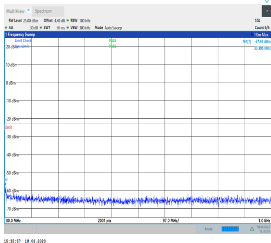
1-N2-PC3-15-20-L-1-DFT-PI2BPSK-Inner_1RB_Left -1@1-30-1000-Ant3-33.40--57.44--23-PASS
