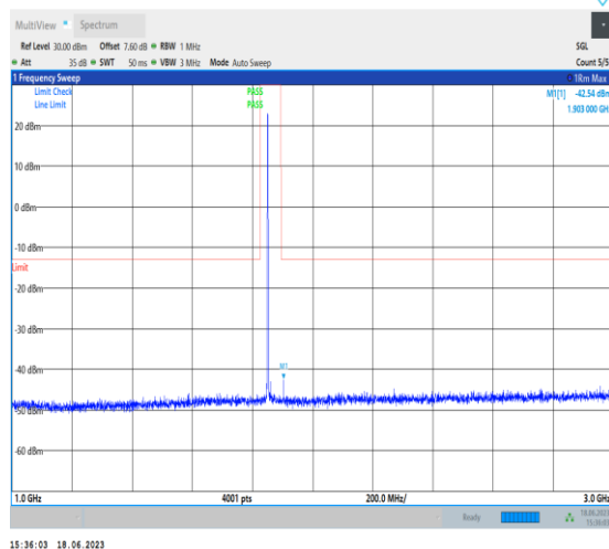
1-N2-PC3-15-20-L-1-DFT-PI2BPSK-Inner_1RB_Left- 1@1-1000-3000-Ant3-1903.00--42.54--13-PASS
