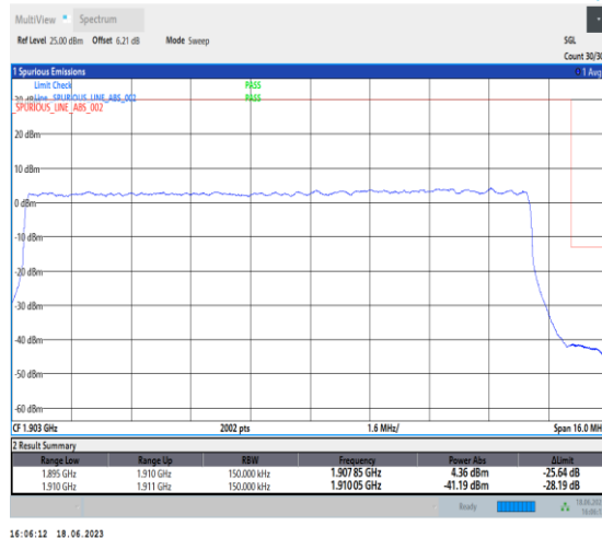
1-N2-PC3-15-15-H-3-DFT-PI2BPSK-Outer_Full-75@0-Ant3-1-seegraph-PASS-see graph
