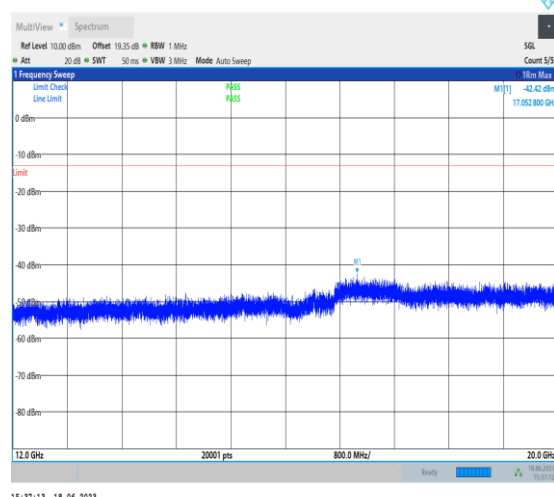
1-N2-PC3-15-20-M-1-DFT-PI2BPSK-Inner_1RB_Left- 1@1-12000-20000-Ant3-17052.80--42.42--13-PASS
