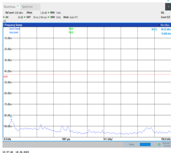
1-N2-PC3-15-20-H-1-DFT-PI2BPSK-Inner_1RB_Lef t-1@1-0.009-0.15-Ant3-0.02--85.25--43-PASS
