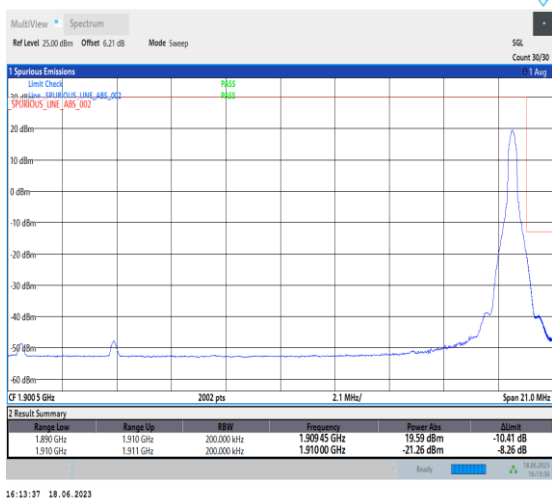
1-N2-PC3-15-20-H-5-CP-QPSK-Edge_1RB_Right-1@105-Ant3-1-seegraph-PASS-see graph
