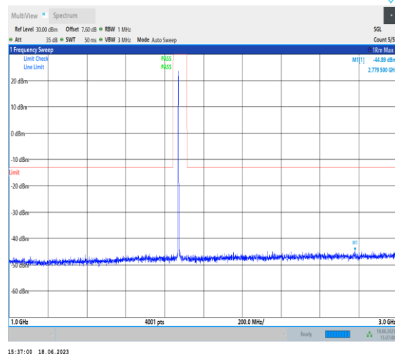
1-N2-PC3-15-20-M-1-DFT-PI2BPSK-Inner_1RB_Left- 1@1-1000-3000-Ant3-2779.50--44.89--13-PASS
