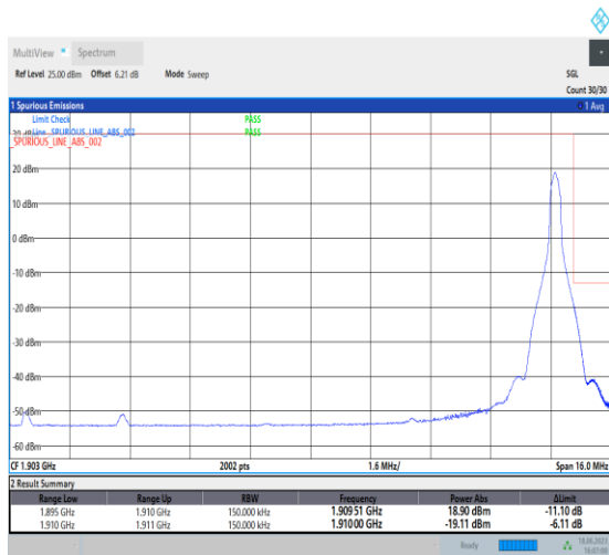
1-N2-PC3-15-15-H-2-DFT-PI2BPSK-Edge_1RB_Right-1@78-Ant3-1-seegraph-PASS-see graph
