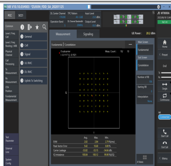
1-N5-PC3-15-20-M-8-CP-64QAM-Outer_Full-106@0- Ant0-see graph-PASS
