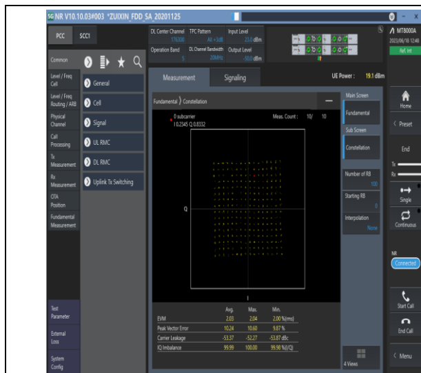
1-N5-PC3-15-20-M-5-DFT-256QAM-Outer_Full-100 @0-Ant0-see graph-PASS
