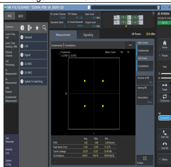
1-N5-PC3-15-20-M-6-CP-QPSK-Outer_Full-106@0- Ant0-see graph-PASS
