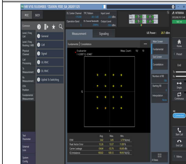
1-N5-PC3-15-20-M-7-CP-16QAM-Outer_Full-106@0- Ant0-see graph-PASS
