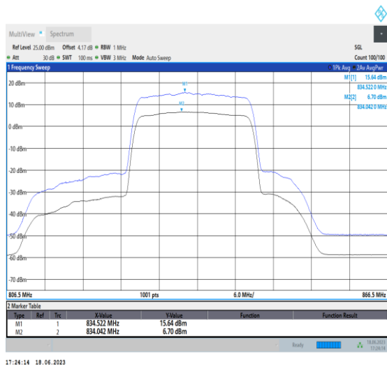
1-N5-PC3-15-20-M-1-DFT-256QAM-Outet_Full-100 @0-Ant0-8.94-100%-0.00-8.94-PASS-≤13
