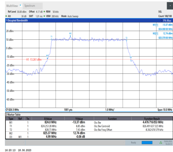
1-N5-PC3-15-5-L-2-DFT-P12BPSK-Outet_Full-25@0 -Ant0-4.477-4.990-≤5-PASS
