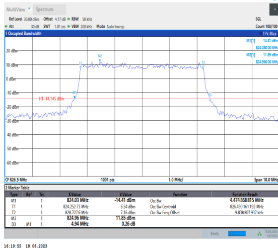
1-N5-PC3-15-5-L-1-DFT-QPSK-Outet_Full-25@0-An t0-4.475-4.940-≤5-PASS
