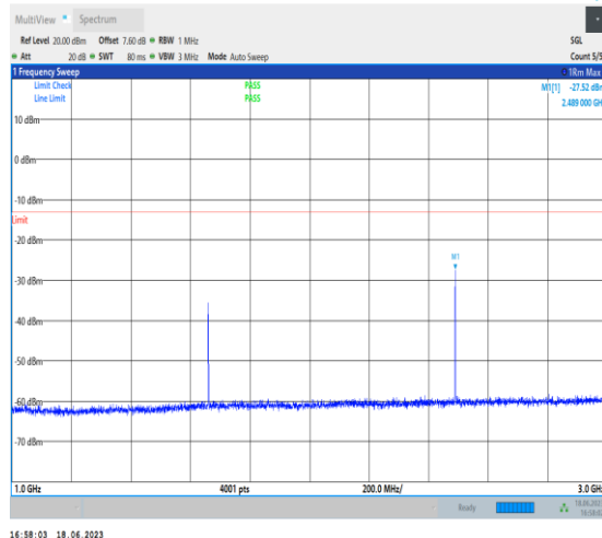
1-N5-PC3-15-20-H-1-DFT-PI2BPSK-Inner_1RB_Left -1@1-1000-3000-Ant0-2489.00--27.52--13-PASS
