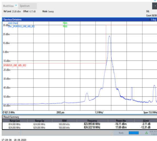
1-N5-PC3-15-5-L-4-CP-QPSK-Edge_1RB_Left-1@0-A nt0-1-seegraph-PASS-see graph
