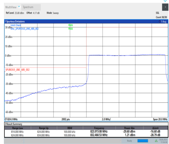
1-N5-PC3-15-10-L-6-CP-QPSK-Outer_Full-52@0-Ant0-1-seegraph-PASS-see graph
