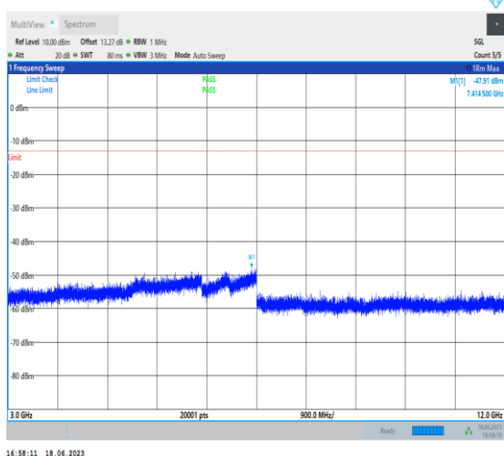
1-N5-PC3-15-20-H-1-DFT-PI2BPSK-Inner_1RB_Left -1@1-3000-12000-Ant0-7414.50--47.91--13-PASS
