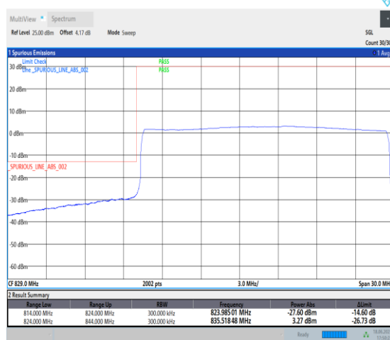
1-N5-PC3-15-20-L-6-CP-QPSK-Outer_Full-106@0 -Ant0-1-seegraph-PASS-see graph
