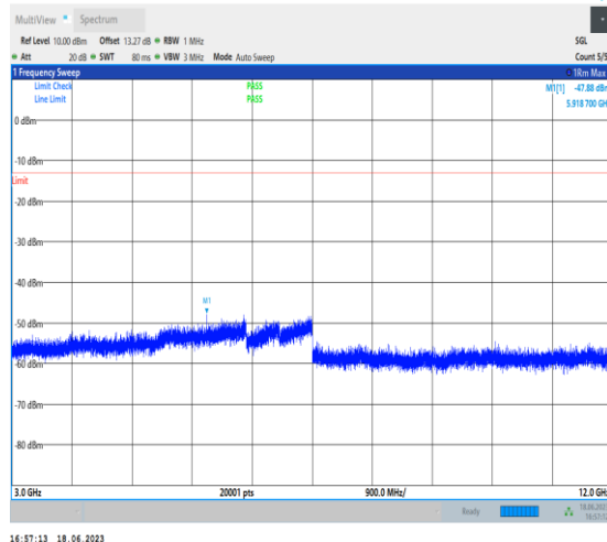
1-N5-PC3-15-20-M-1-DFT-PI2BPSK-Inner_1RB_Left -1@1-3000-12000-Ant0-5918.70--47.88--13-PASS
