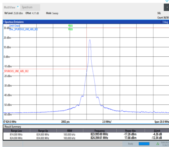
1-N5-PC3-15-10-L-4-CP-QPSK-Edge_1RB_Left-1@0-Ant0-1-seegraph-PASS-see graph
