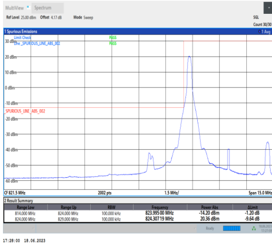
1-N5-PC3-15-5-L-1-DFT-PI2BPSK-Edge_1RB_Left-1 @0-Ant0-1-seegraph-PASS-see graph
