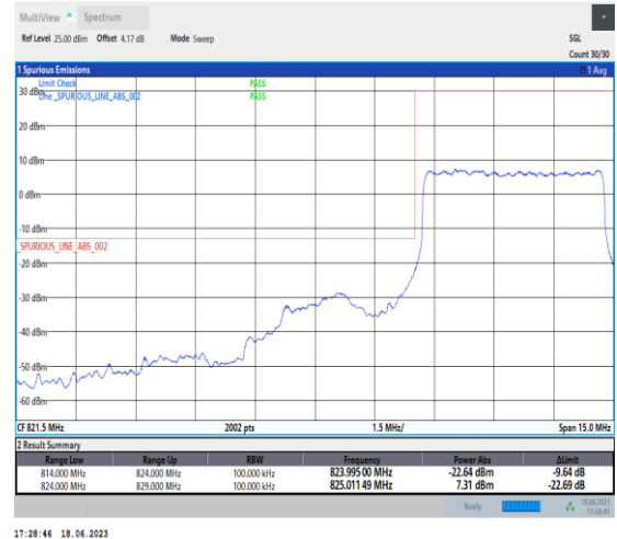
1-N5-PC3-15-5-L-3-DFT-PI2BPSK-Outer_Full-25 @0-Ant0-1-seegraph-PASS-see graph
