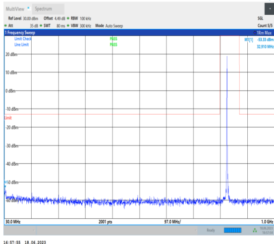
1-N5-PC3-15-20-H-1-DFT-PI2BPSK-Inner_1RB_Left -1@1-30-1000-Ant0-32.91--53.33--13-PASS
