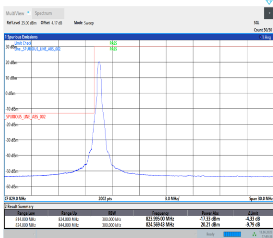
1-N5-PC3-15-20-L-4-CP-QPSK-Edge_1RB_Left-1@0- Ant0-1-seegraph-PASS-see graph
