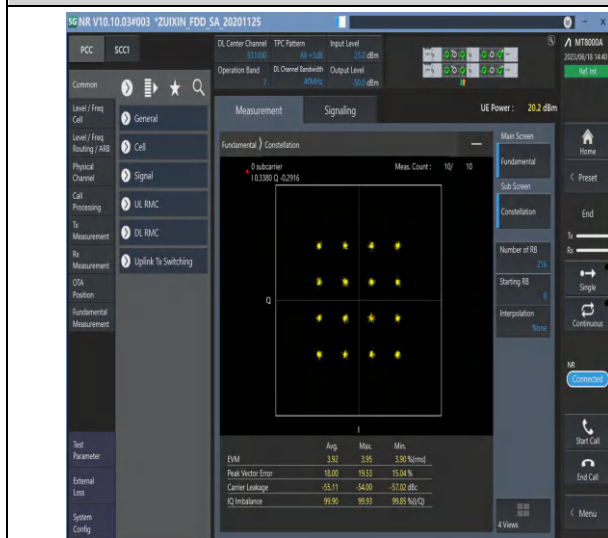
1-N7-PC3-15-40-M-7-CP-16QAM-Outer_Full-216@0-Ant0-see graph-PASS
