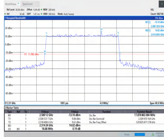
1-N7-PC3-15-20-L-1-DFT-QPSK-Outer_Full-100@0-Ant0-17.877-18.680-≤20-PASS
