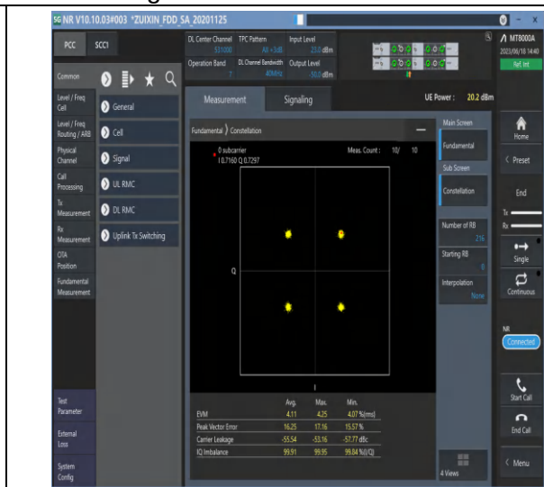
1-N7-PC3-15-40-M-6-CP-QPSK-Outer_Full-216@0-Ant0-see graph-PASS
