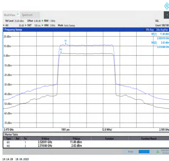
1-N7-PC3-15-40-M-1-DFT-256QAM-Outter_Full-216 @0-Ant0-9.07-100%-0.00-9.07-PASS-≤13
