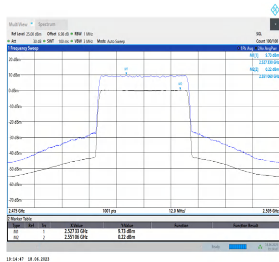
1-N7-PC3-15-40-M-2-CP-256QAM-Outter_Full-216 @0-Ant0-9.51-100%-0.00-9.51-PASS-≤13
