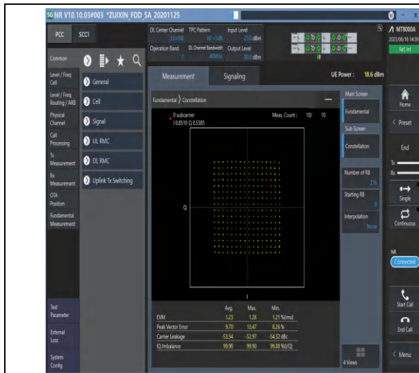
1-N7-PC3-15-40-M-5-DFT-256QAM-Outer_Full-216@0-Ant0-see graph-PASS
