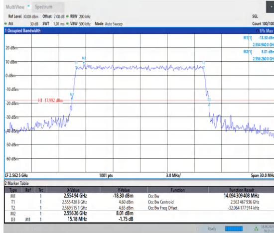
1-N7-PC3-15-15-H-9-CP-256QAM-Outer_Full-79@0-Ant0-14.094-15.180-≤15-PASS
