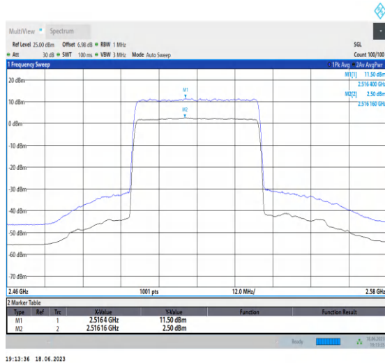
1-N7-PC3-15-40-L-1-DFT-256QAM-Outter_Full-216@ 0-Ant0-9.00-100%-0.00-9.00-PASS-≤13
