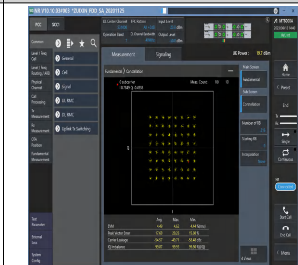
1-N7-PC3-15-40-M-8-CP-64QAM-Outer_Full-216@0-Ant0-see graph-PASS
