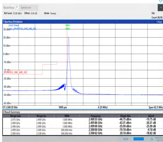
1-N7-PC3-15-25-L-4-CP-QPSK-Edge_1RB_Left-1@0-Ant0-1--PASS-see graph
