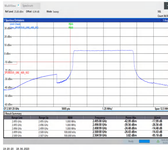
1-N7-PC3-15-5-L-6-CP-QPSK-Outer_Full-25@0-Ant0-1--PASS-see graph
