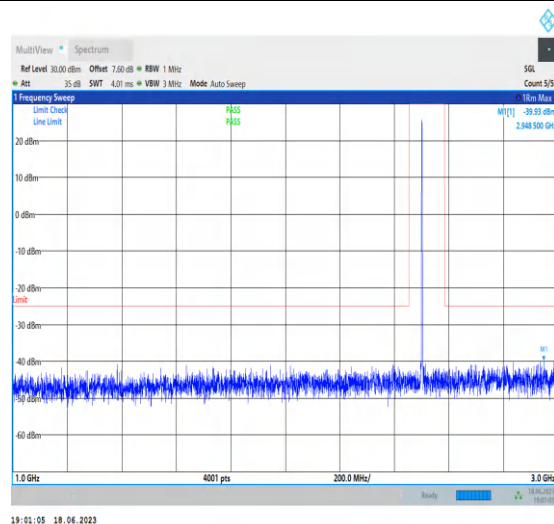
1-N7-PC3-15-40-L-1-DFT-PI2BPSK-Inner_1RB_Left- 1@1-1000-3000-Ant0-2948.50--39.93--25-PASS
