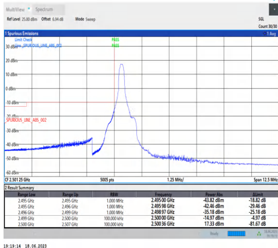
1-N7-PC3-15-5-L-4-CP-QPSK-Edge_1RB_Left-1@0-Ant0-1--PASS-see graph
