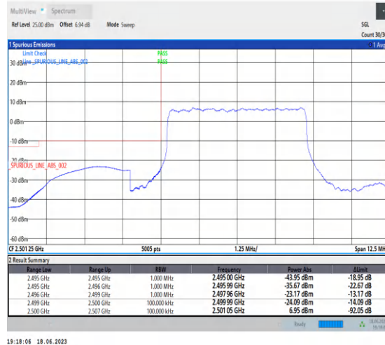
1-N7-PC3-15-5-L-3-DFT-PI2BPSK-Outer_Full-25@0-Ant0-1--PASS-see graph
