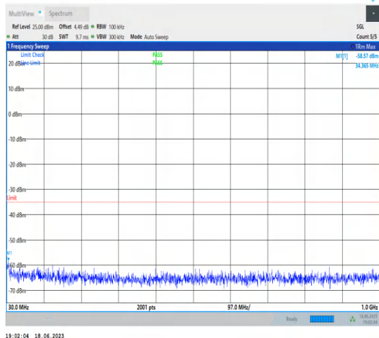
1-N7-PC3-15-40-M-1-DFT-PI2BPSK-Inner_1RB_Lef t-1@1-30-1000-Ant0-34.37--58.57--35-PASS
