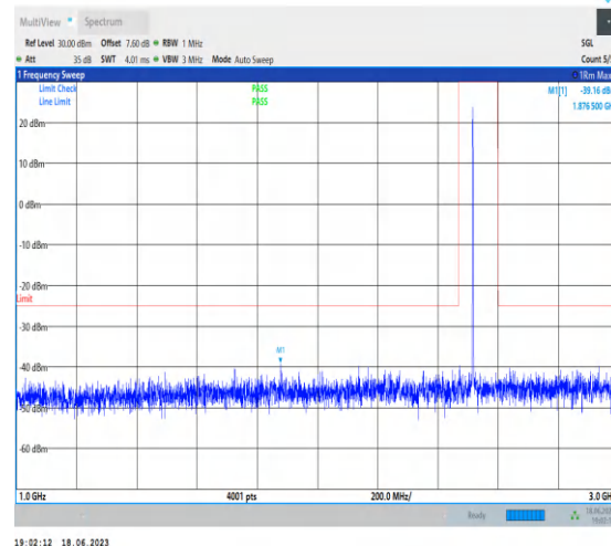
1-N7-PC3-15-40-M-1-DFT-PI2BPSK-Inner_1RB_Left- 1@1-1000-3000-Ant0-1876.50--39.16--25-PASS
