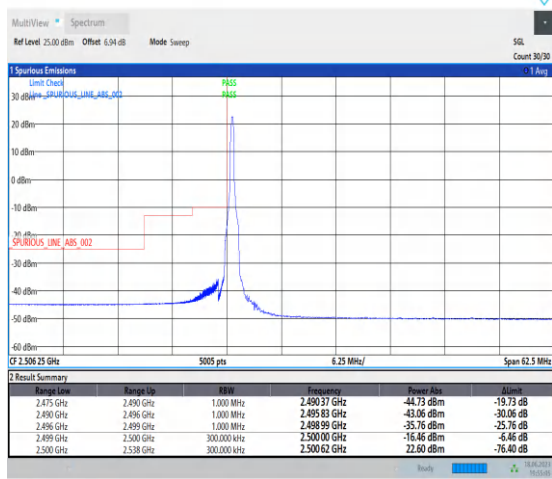
1-N7-PC3-15-25-L-1-DFT-PI2BPSK-Edge_1RB_Left-1@0-Ant0-1--PASS-see graph
