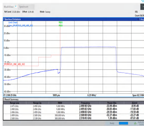
1-N7-PC3-15-25-L-6-CP-QPSK-Outer_Full-133@0-Ant0-1--PASS-see graph
