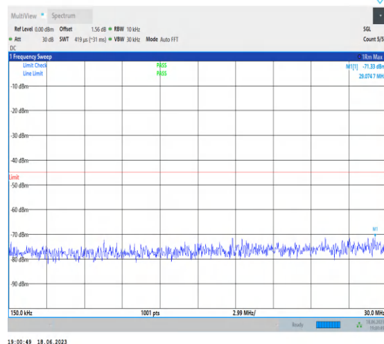
1-N7-PC3-15-40-L-1-DFT-PI2BPSK-Inner_1RB_Left- 1@1-0.15-30-Ant0-29.07--71.33--45-PASS
