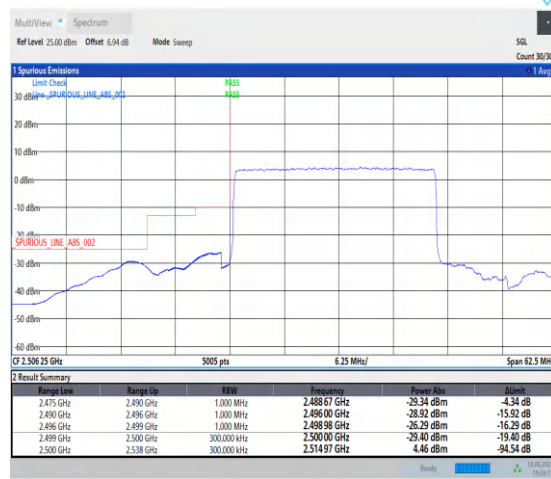
1-N7-PC3-15-25-L-3-DFT-PI2BPSK-Outer_Full-128@0-Ant0-1--PASS-see graph
