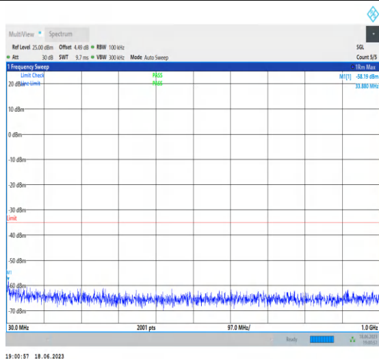
1-N7-PC3-15-40-L-1-DFT-PI2BPSK-Inner_1RB_Left -1@1-30-1000-Ant0-33.88--58.19--35-PASS
