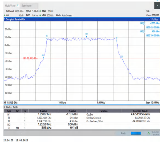
1-N25-PC3-15-5-L-4-DFT-64QAM-Outter_Full-25@0-Ant3-4.475-5.050-≤5-PASS
