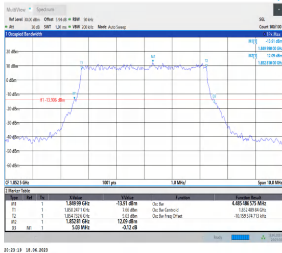
1-N25-PC3-15-5-L-1-DFT-QPSK-Outter_Full-25@0-A nt3-4.485-5.030-≤5-PASS
