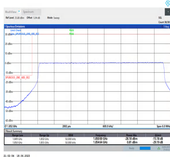
1-N25-PC3-15-5-L-6-CP-QPSK-Outer_Full-25@0- Ant3-1-seegraph-PASS-see graph
