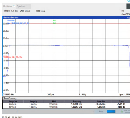
1-N25-PC3-15-30-L-6-CP-QPSK-Outer_Full-160@0-Ant3-1-seegraph-PASS-see graph
