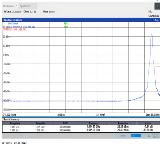
1-N25-PC3-15-30-H-2-DFT-PI2BPSK-Edge_1RB_Righ t-1@159-Ant3-1-seegraph-PASS-see graph
