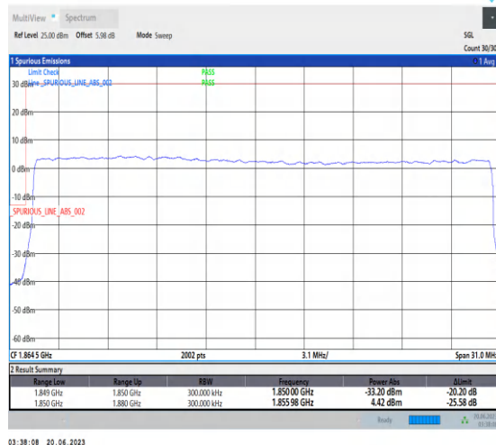
1-N25-PC3-15-30-L-3-DFT-PI2BPSK-Outer_Full-160@0-Ant3-1-seegraph-PASS-see graph
