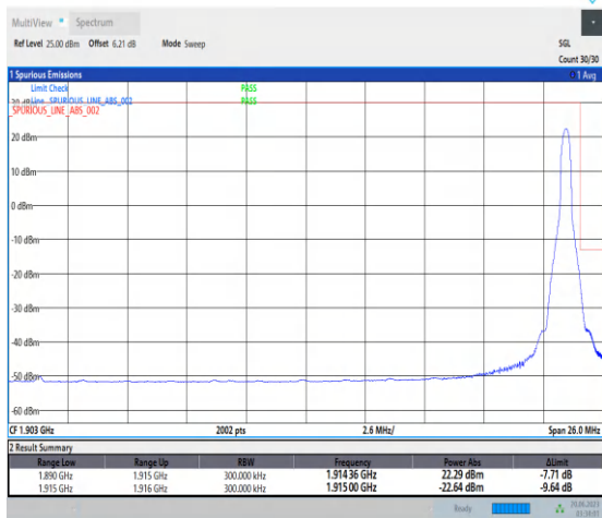
1-N25-PC3-15-25-H-2-DFT-PI2BPSK-Edge_1RB_Righ t-1@132-Ant3-1-seegraph-PASS-see graph
