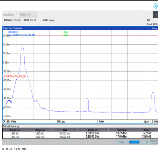
1-N25-PC3-15-10-L-4-CP-QPSK-Edge_1RB_Left-1@0-Ant3-1-seegraph-PASS-see graph
