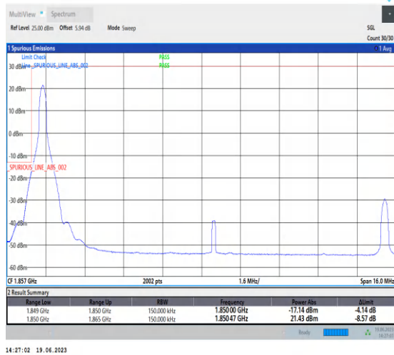
1-N25-PC3-15-15-L-1-DFT-PI2BPSK-Edge_1RB_Left-1@0-Ant3-1-seegraph-PASS-see graph
