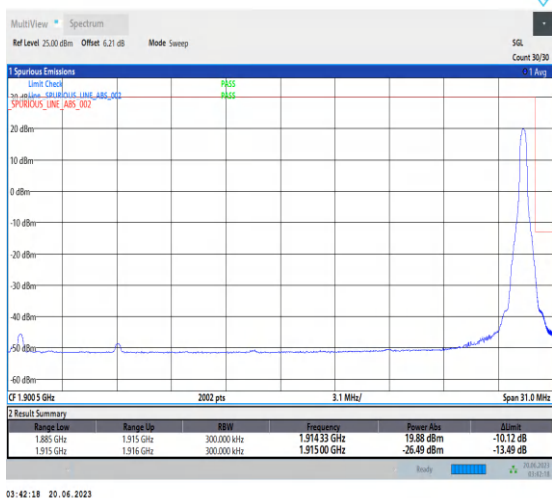
1-N25-PC3-15-30-H-5-CP-QPSK-Edge_1RB_Right-1 @159-Ant3-1-seegraph-PASS-see graph
