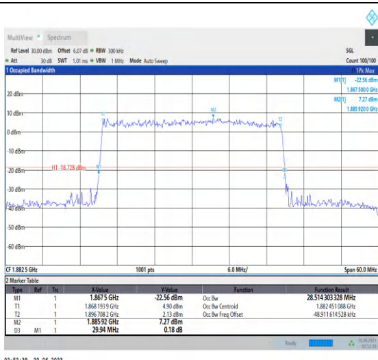
1-N25-PC3-15-30-M-9-CP-256QAM-Outer_Full-160 @0-Ant3-28.514-29.940-≤30-PASS
