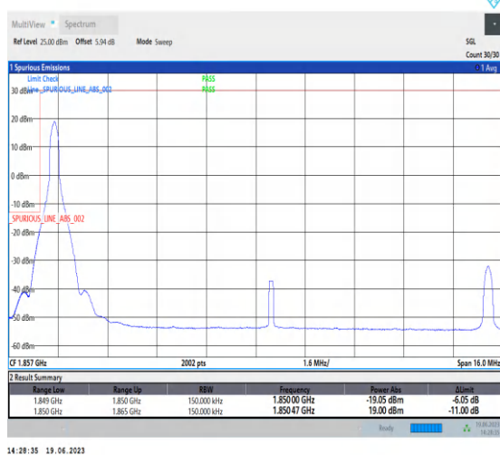
1-N25-PC3-15-15-L-4-CP-QPSK-Edge_1RB_Left-1@0-Ant3-1-seegraph-PASS-see graph
