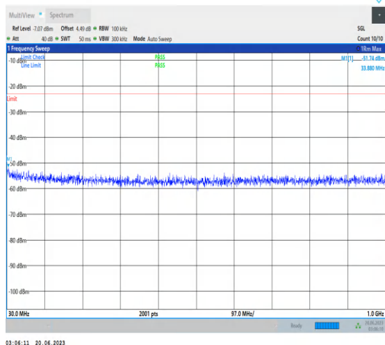
1-N25-PC3-15-40-M-1-DFT-PI2BPSK-Inner_1RB_L eft-1@1-30-1000-Ant3-33.88--51.74--23-PASS
