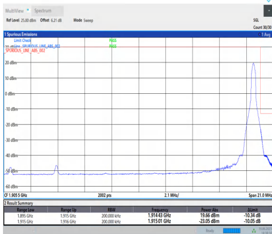
1-N25-PC3-15-20-H-5-CP-QPSK-Edge_1RB_Right-1 @105-Ant3-1-seegraph-PASS-see graph
