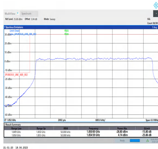
1-N25-PC3-15-5-L-3-DFT-PI2BPSK-Outer_Full-25 @0-Ant3-1-seegraph-PASS-see graph
