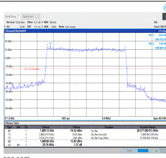
1-N25-PC3-15-30-H-1-DFT-QPSK-Outer_Full-160@ 0-Ant3-28.577-29.760-≤30-PASS
