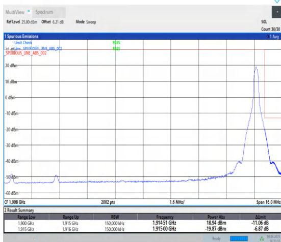
1-N25-PC3-15-15-H-5-CP-QPSK-Edge_1RB_Righ t-1@78-Ant3-1-seegraph-PASS-see graph
