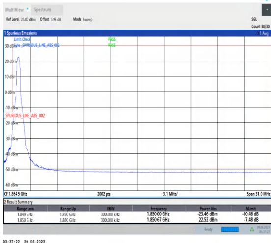
1-N25-PC3-15-30-L-1-DFT-PI2BPSK-Edge_1RB_Left-1@0-Ant3-1-seegraph-PASS-see graph
