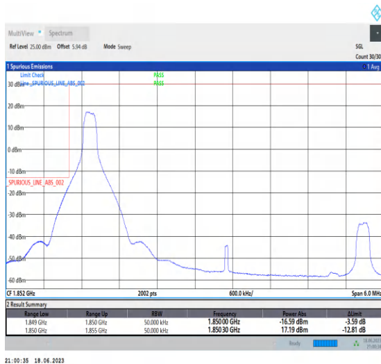
1-N25-PC3-15-5-L-1-DFT-PI2BPSK-Edge_1RB_Left-1 @0-Ant3-1-seegraph-PASS-see graph
