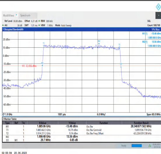
1-N25-PC3-15-30-H-2-DFT-PI2BPSK-Outer_Full-160 @0-Ant3-28.549-29.700-≤30-PASS
