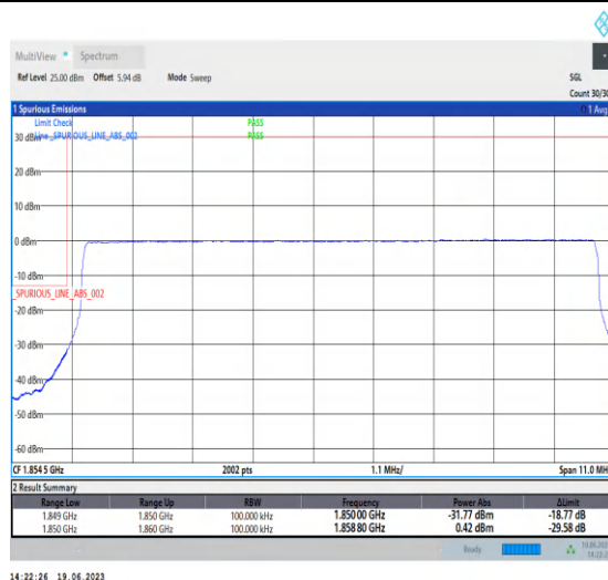
1-N25-PC3-15-10-L-6-CP-QPSK-Outer_Full-52@0-Ant3-1-seegraph-PASS-see graph
