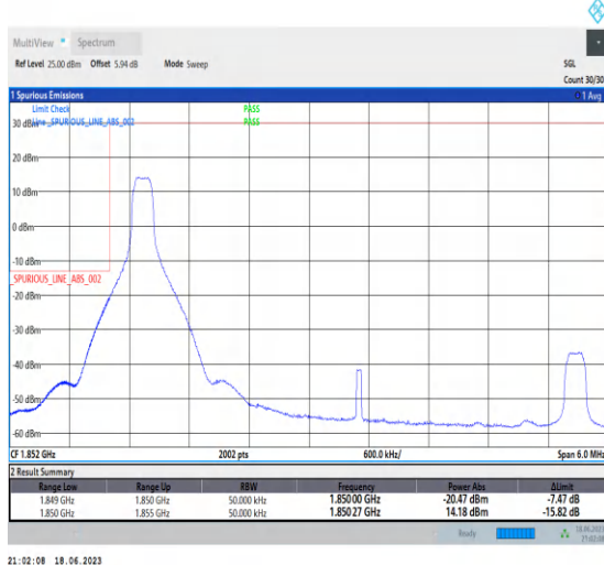
1-N25-PC3-15-5-L-4-CP-QPSK-Edge_1RB_Left-1@0- Ant3-1-seegraph-PASS-see graph
