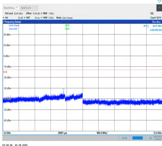
1-N25-PC3-15-40-M-1-DFT-PI2BPSK-Inner_1RB_L eft-1@1-3000-12000-Ant3-6425.40--34.07--13-PAS S
