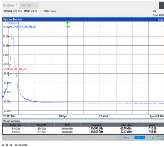
1-N25-PC3-15-25-L-1-DFT-PI2BPSK-Edge_1RB_Left-1@0-Ant3-1-seegraph-PASS-see graph
