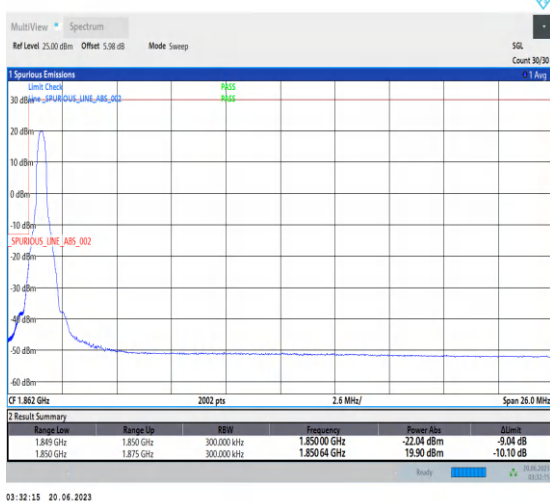
1-N25-PC3-15-25-L-4-CP-QPSK-Edge_1RB_Left-1@0-Ant3-1-seegraph-PASS-see graph
