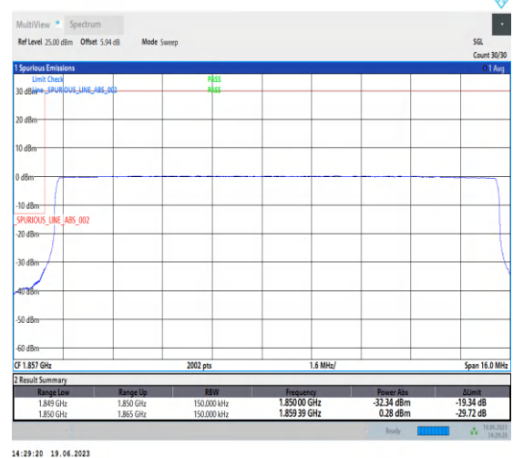
1-N25-PC3-15-15-L-6-CP-QPSK-Outer_Full-79@0-Ant3-1-seegraph-PASS-see graph
