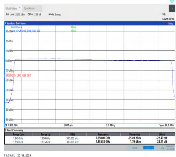
1-N25-PC3-15-25-L-6-CP-QPSK-Outer_Full-133@0-Ant3-1-seegraph-PASS-see graph
