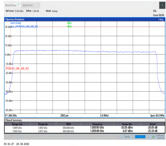
1-N25-PC3-15-25-L-3-DFT-PI2BPSK-Outer_Full-128@0-Ant3-1-seegraph-PASS-see graph
