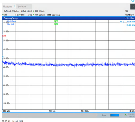
1-N25-PC3-15-40-H-1-DFT-PI2BPSK-Inner_1RB_L eft-1@1-30-1000-Ant3-33.88--51.59--23-PASS
