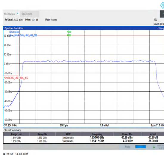
1-N25-PC3-15-10-L-3-DFT-PI2BPSK-Outer_Full-50@0-Ant3-1-seegraph-PASS-see graph
