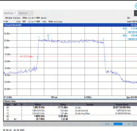
1-N25-PC3-15-30-H-3-DFT-16QAM-Outer_Full-160 @0-Ant3-28.607-29.700-≤30-PASS
