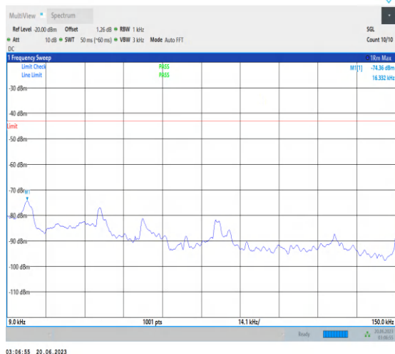
1-N25-PC3-15-40-H-1-DFT-PI2BPSK-Inner_1RB_L eft-1@1-0.009-0.15-Ant3-0.02--74.36--43-PASS
