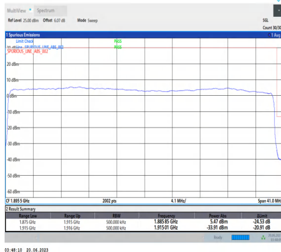
1-N25-PC3-15-40-H-3-DFT-PI2BPSK-Outer_Full-2 16@0-Ant3-1-seegraph-PASS-see graph
