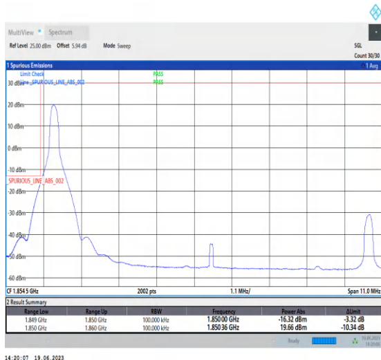
1-N25-PC3-15-10-L-1-DFT-PI2BPSK-Edge_1RB_Left-1@0-Ant3-1-seegraph-PASS-see graph
