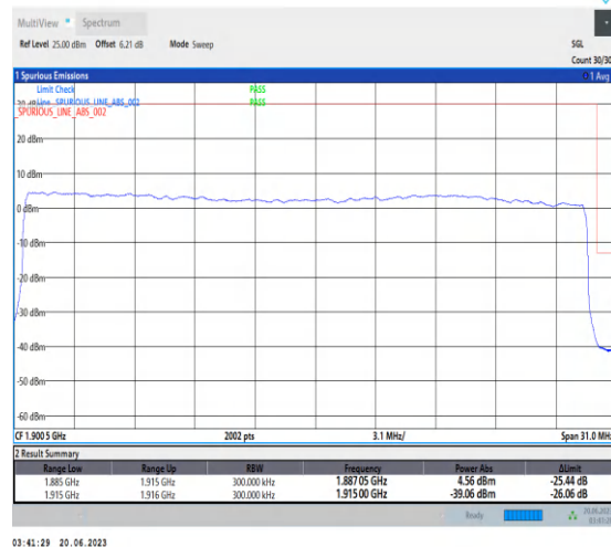
1-N25-PC3-15-30-H-3-DFT-PI2BPSK-Outer_Full-1 60@0-Ant3-1-seegraph-PASS-see graph
