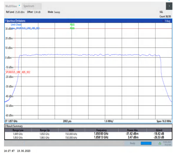
1-N25-PC3-15-15-L-3-DFT-PI2BPSK-Outer_Full-75@0-Ant3-1-seegraph-PASS-see graph
