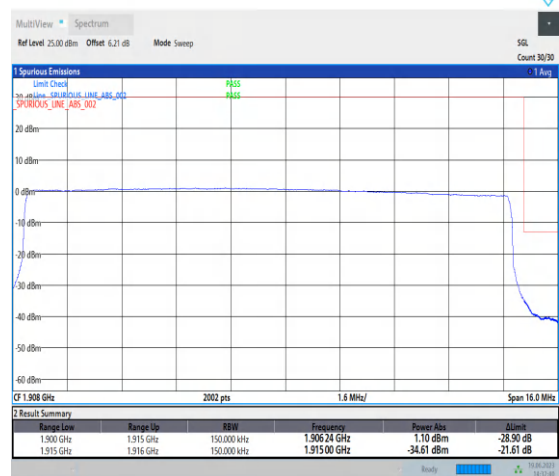
1-N25-PC3-15-15-H-6-CP-QPSK-Outer_Full-79@0 -Ant3-1-seegraph-PASS-see graph
