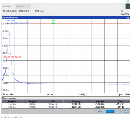
1-N25-PC3-15-30-L-4-CP-QPSK-Edge_1RB_Left-1@0-Ant3-1-seegraph-PASS-see graph
