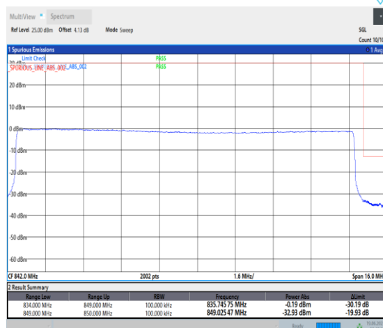
1-N26-824-849-PC3-15-15-H-6-CP-QPSK-Outer_Full-79@0-Ant0-1-seegraph-PASS-see graph
