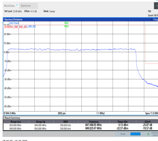
1-N26-824-849-PC3-15-10-H-3-DFT-PI2BPSK-Out er_Full-50@0-Ant0-1-seegraph-PASS-see graph
