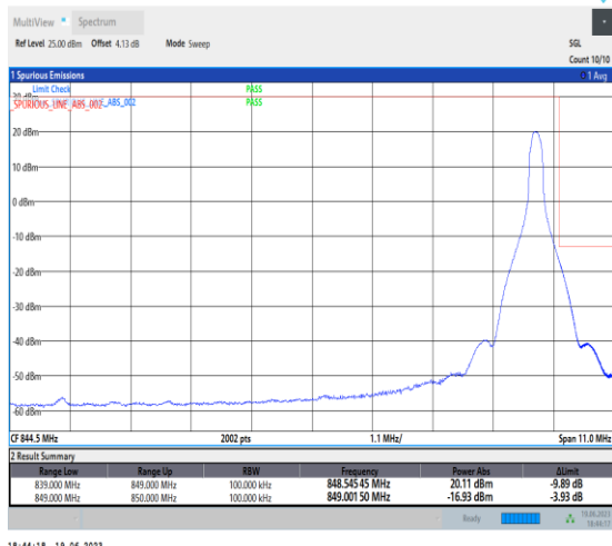
1-N26-824-849-PC3-15-10-H-2-DFT-PI2BPSK-Edge_1 RB_Right-1@51-Ant0-1-seegraph-PASS-see graph
