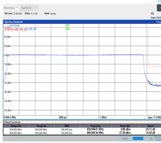
1-N26-824-849-PC3-15-10-H-6-CP-QPSK-Outer_F ull-52@0-Ant0-1-seegraph-PASS-see graph
