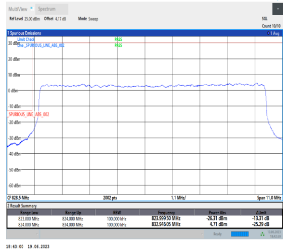
1-N26-824-849-PC3-15-10-L-3-DFT-PI2BPSK-Out er_Full-50@0-Ant0-1-seegraph-PASS-see graph
