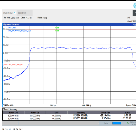
1-N26-824-849-PC3-15-5-L-3-DFT-PI2BPSK-Outer _Full-25@0-Ant0-1-seegraph-PASS-see graph
