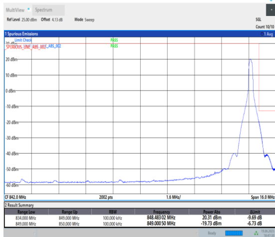
1-N26-824-849-PC3-15-15-H-2-DFT-PI2BPSK-Edge_1_RB_Right-1@78-Ant0-1-seegraph-PASS-see graph
