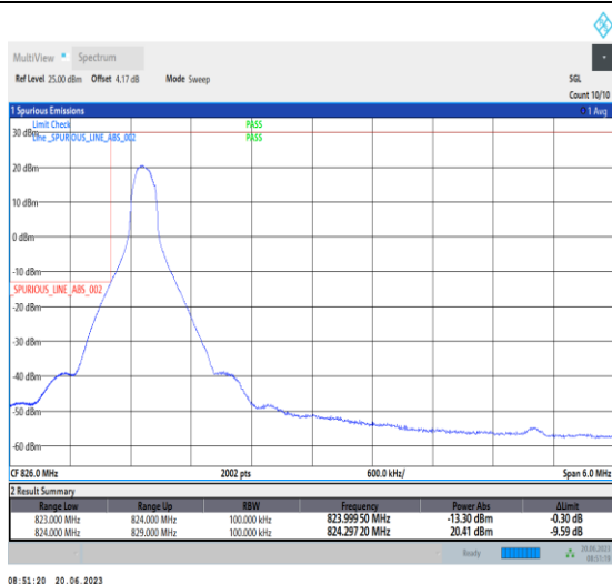
1-N26-824-849-PC3-15-5-L-1-DFT-PI2BPSK-Edge_1R B_Left-1@0-Ant0-1-seegraph-PASS-see graph
