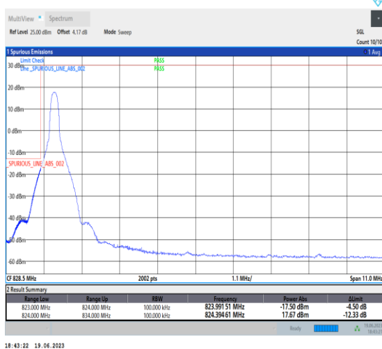
1-N26-824-849-PC3-15-10-L-4-CP-QPSK-Edge_1RB_Left-1@0-Ant0-1-seegraph-PASS-see graph
