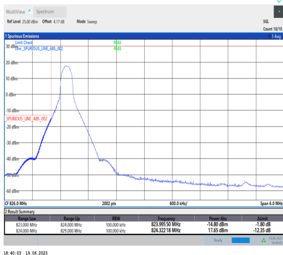
1-N26-824-849-PC3-15-5-L-4-CP-QPSK-Edge_1RB_L eft-1@0-Ant0-1-seegraph-PASS-see graph
