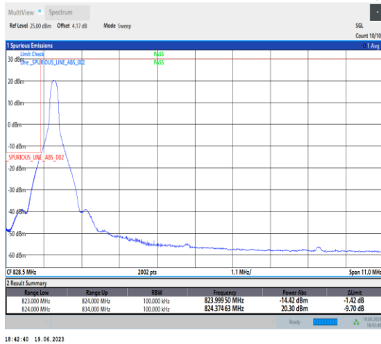
1-N26-824-849-PC3-15-10-L-1-DFT-PI2BPSK-Edge_1 RB_Left-1@0-Ant0-1-seegraph-PASS-see graph
