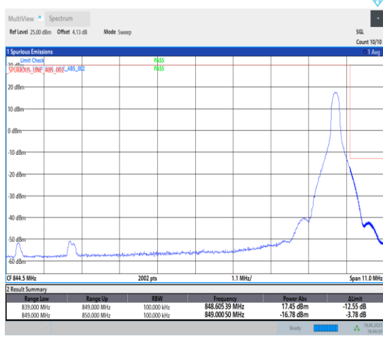
1-N26-824-849-PC3-15-10-H-5-CP-QPSK-Edge_1RB_Right-1@51-Ant0-1-seegraph-PASS-see graph
