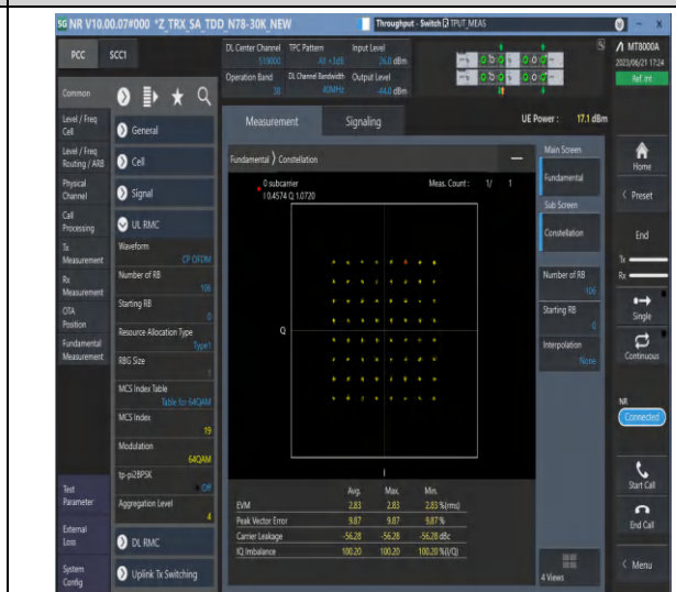
1-N38-PC3-30-40-M-8-CP-64QAM-Outter_Full-106 @0-Ant0-see graph-PASS
