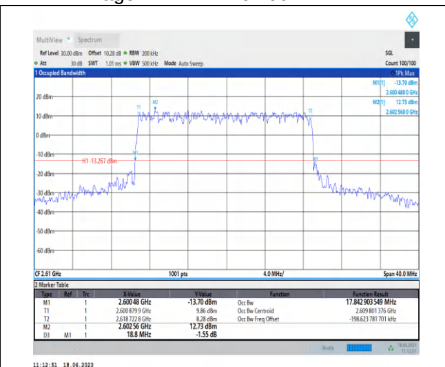
1-N38-PC3-30-20-H-2-DFT-QPSK-Outer_Full-50@0-Ant0-17.843-18.800-≤20-PASS
