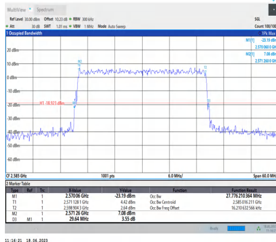
1-N38-PC3-30-30-L-9-CP-256QAM-Outer_Full-78@0-Ant0-27.776-29.640-≤30-PASS
