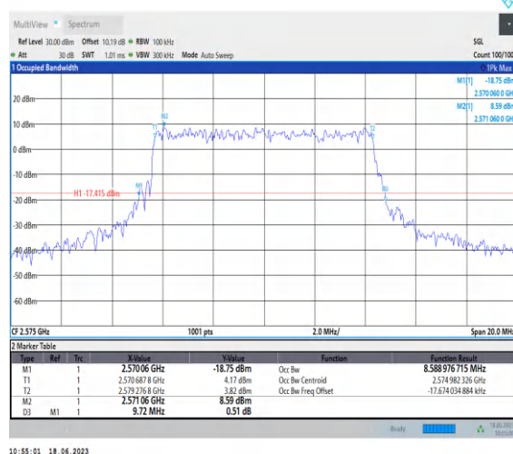
1-N38-PC3-30-10-L-8-CP-64QAM-Outer_Full-24@0-Ant0-8.589-9.720-≤10-PASS
