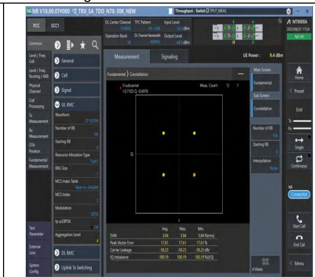
1-N38-PC3-30-40-M-6-CP-QPSK-Outter_Full-106@ 0-Ant0-see graph-PASS
