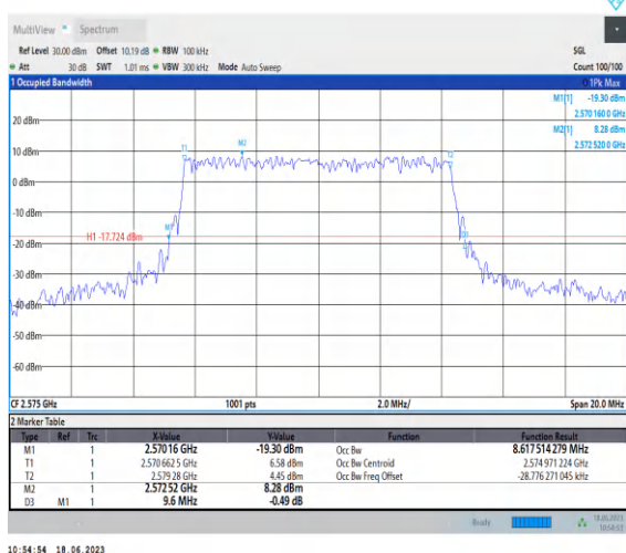
1-N38-PC3-30-10-L-7-CP-16QAM-Outer_Full-24@0-Ant0-8.618-9.600-≤10-PASS
