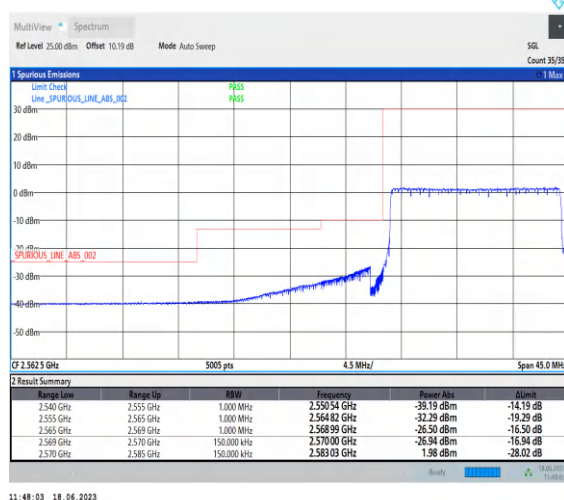
1-N38-PC3-30-15-L-6-CP-QPSK-Outer_Full-38@0-Ant0-1--PASS-see graph
