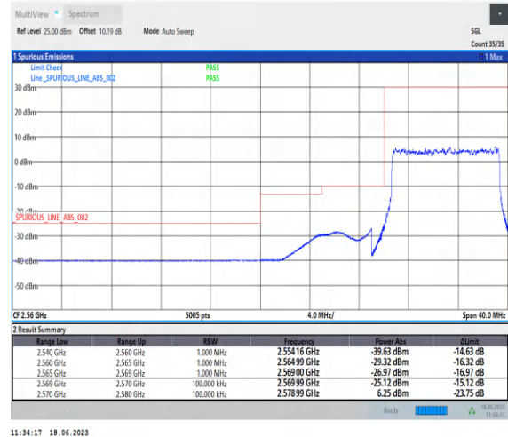
1-N38-PC3-30-10-L-3-DFT-PI2BPSK-Outer_Full-24@0-Ant0-1--PASS-see graph
