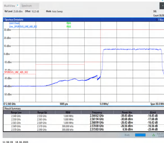
1-N38-PC3-30-20-L-3-DFT-PI2BPSK-Outer_Full-50@0-Ant0-1--PASS-see graph
