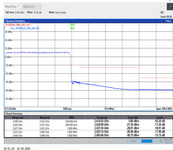
1-N38-PC2-30-40-H-3-CP-QPSK-Outer_Full-106@0-Ant0-1--PASS-see graph
