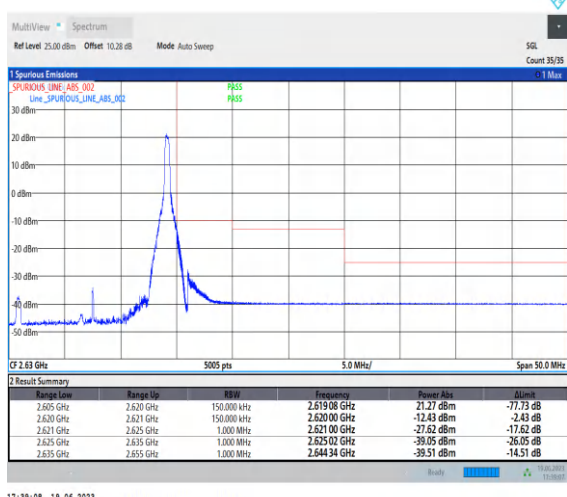
1-N38-PC2-30-15-H-2-CP-QPSK-Edge_1RB_Right-1@37-Ant0-1--PASS-see graph
