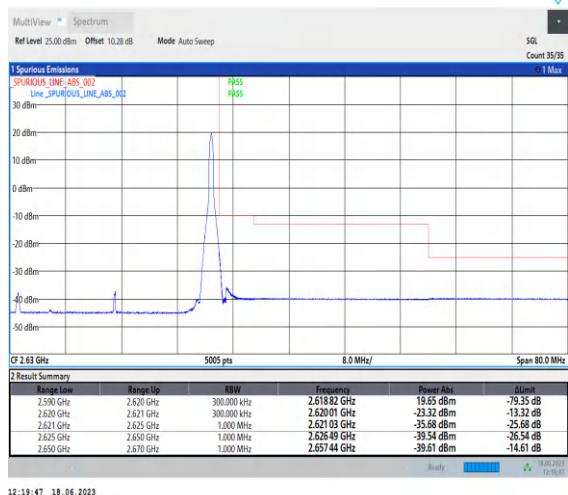
1-N38-PC3-30-30-H-5-CP-QPSK-Edge_1RB_Right-1 @77-Ant0-1--PASS-see graph
