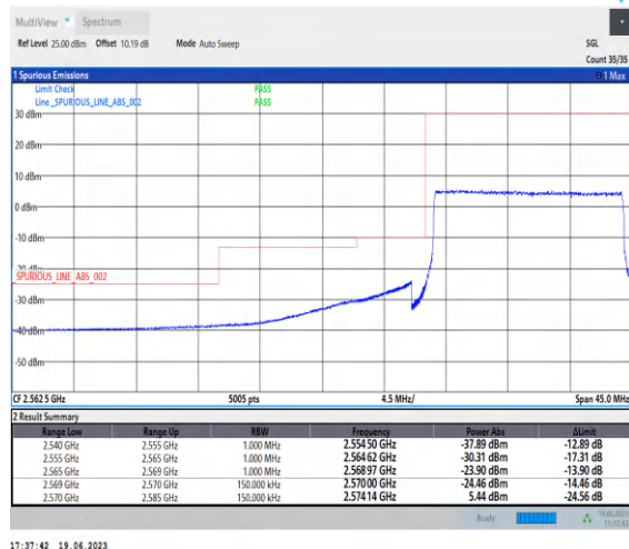
1-N38-PC2-30-15-L-3-CP-QPSK-Outer_Full-38@0-Ant0-1--PASS-see graph
