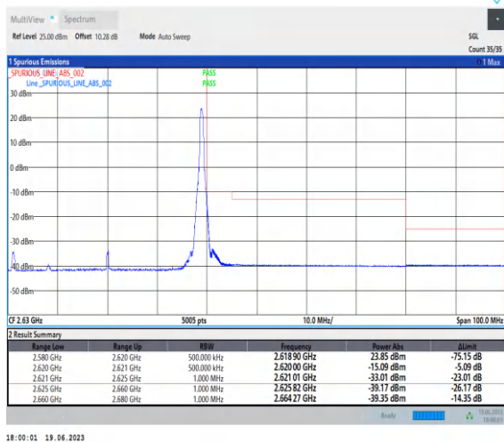
1-N38-PC2-30-40-H-2-CP-QPSK-Edge_1RB_Right-1@105-Ant0-1--PASS-see graph
