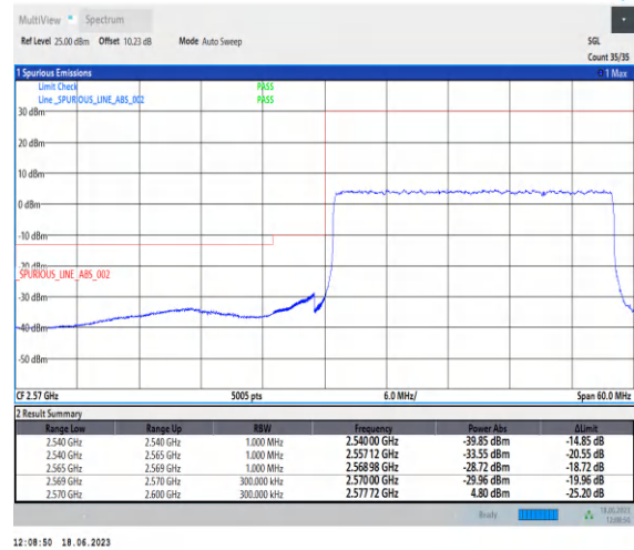
1-N38-PC3-30-30-L-3-DFT-PI2BPSK-Outer_Full-75@0-Ant0-1--PASS-see graph
