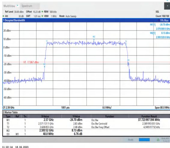
1-N38-PC3-30-40-L-9-CP-256QAM-Outer_Full-106 @0-Ant0-37.724-40.000-≤40-PASS
