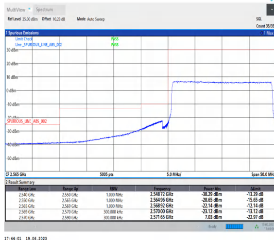
1-N38-PC2-30-20-L-3-CP-QPSK-Outer_Full-51@ 0-Ant0-1--PASS-see graph
