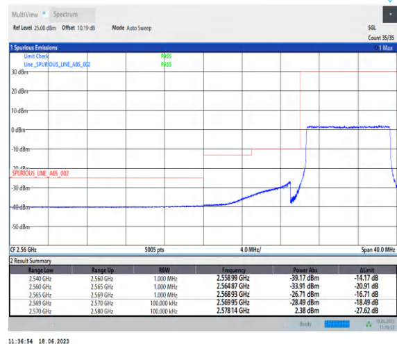
1-N38-PC3-30-10-L-6-CP-QPSK-Outer_Full-24@0-Ant0-1--PASS-see graph
