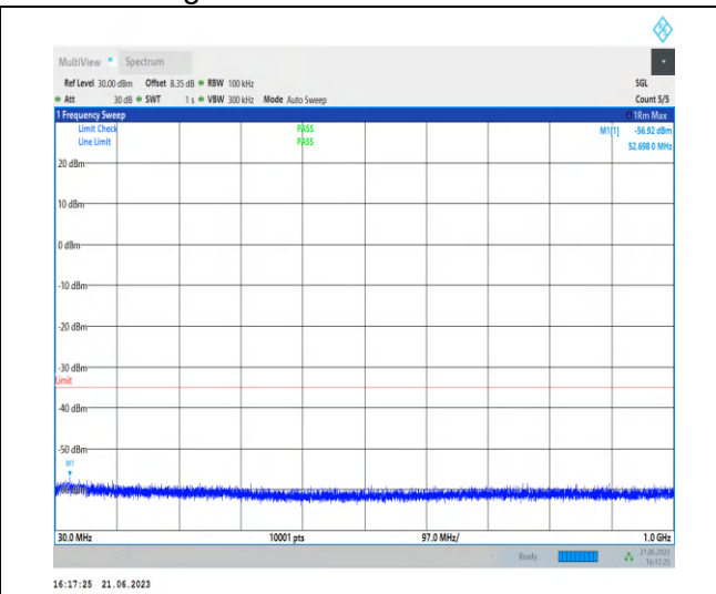
1-N38-PC3-30-40-H-1-N/A-DFT-PI2BPSK-Inner_1R B_Left-1@1-30-1000-Ant0-137.67--56.92--35-PASS
