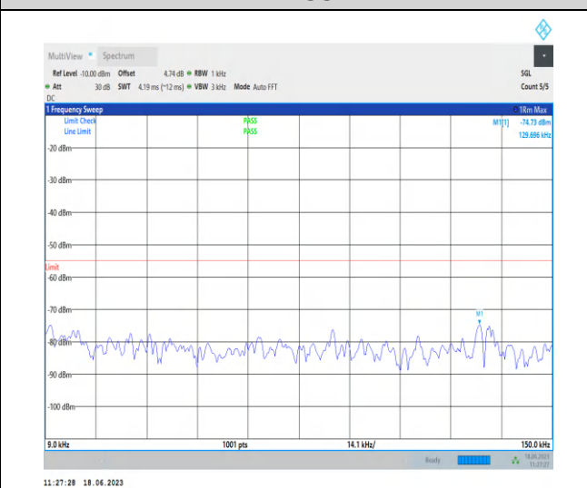
1-N38-PC3-30-40-H-1-N/A-DFT-PI2BPSK-Inner_1R B_Left-1@1-0.009-0.15-Ant0-0.13--74.73--55-PASS
