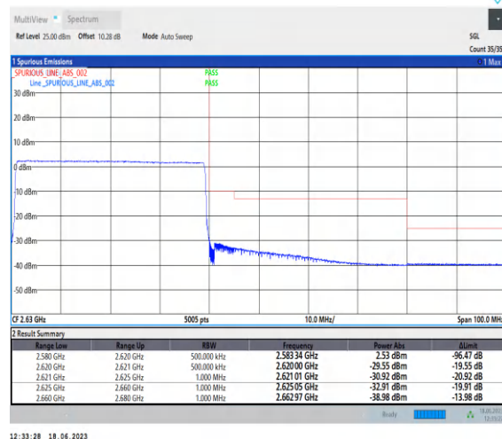
1-N38-PC3-30-40-H-6-CP-QPSK-Outer_Full-106 @0-Ant0-1--PASS-see graph
