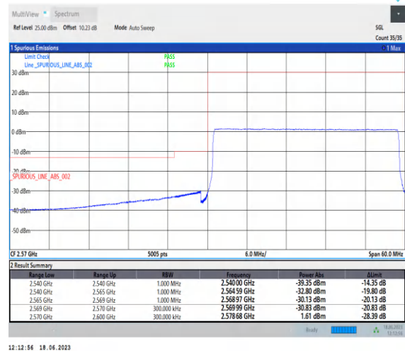
1-N38-PC3-30-30-L-6-CP-QPSK-Outer_Full-78@0-Ant0-1--PASS-see graph
