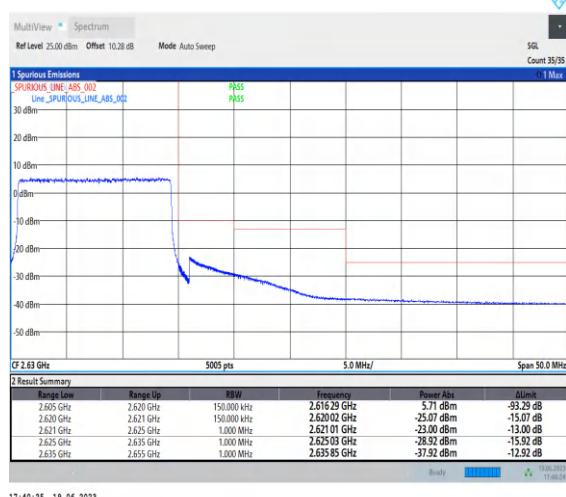
1-N38-PC2-30-15-H-3-CP-QPSK-Outer_Full-38@0-Ant0-1--PASS-see graph
