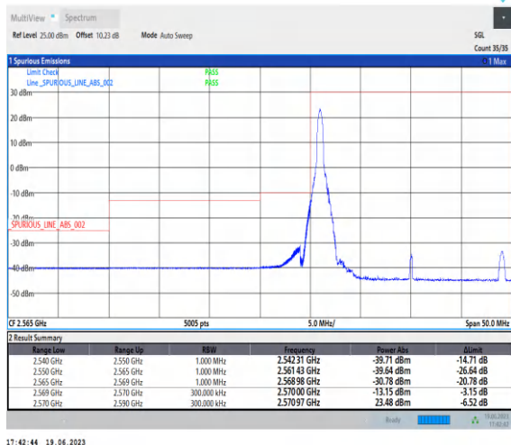
1-N38-PC2-30-20-L-1-CP-QPSK-Edge_1RB_Left-1@0 -Ant0-1--PASS-see graph
