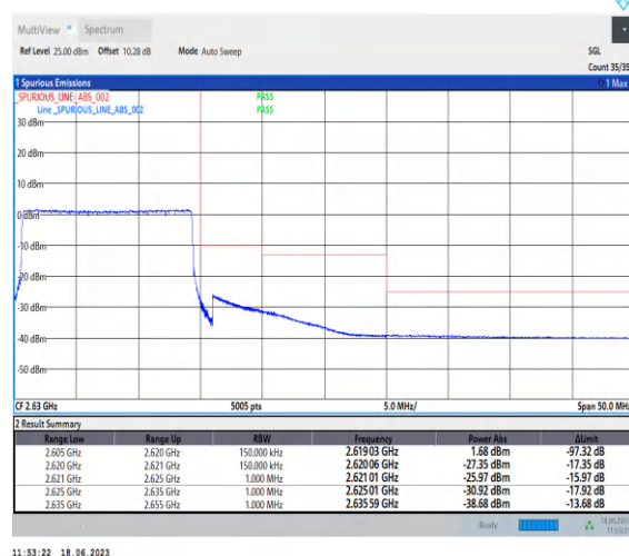
1-N38-PC3-30-15-H-6-CP-QPSK-Outer_Full-38@ 0-Ant0-1--PASS-see graph
