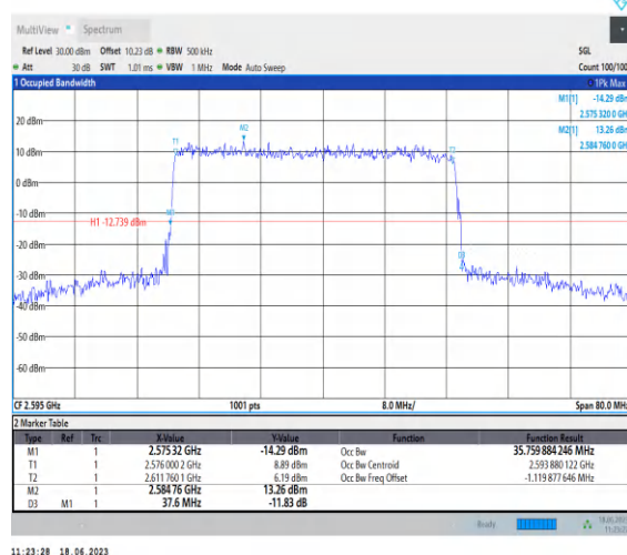
1-N38-PC3-30-40-M-3-DFT-16QAM-Outer_Full-100 @0-Ant0-35.76-37.600-≤40-PASS
