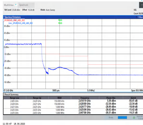
1-N38-PC3-30-15-H-3-DFT-PI2BPSK-Outer_Full-3 6@0-Ant0-1--PASS-see graph
