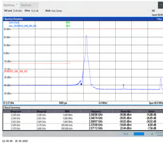
1-N38-PC3-30-30-L-1-DFT-PI2BPSK-Edge_1RB_Left-1@0-Ant0-1--PASS-see graph
