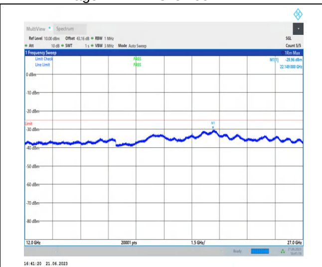
1-N38-PC3-30-40-M-1-N/A-DFT-PI2BPSK-Inner_1R B_Left-1@1-12000-27000-Ant0-22099.50--29.96--25 -PASS
