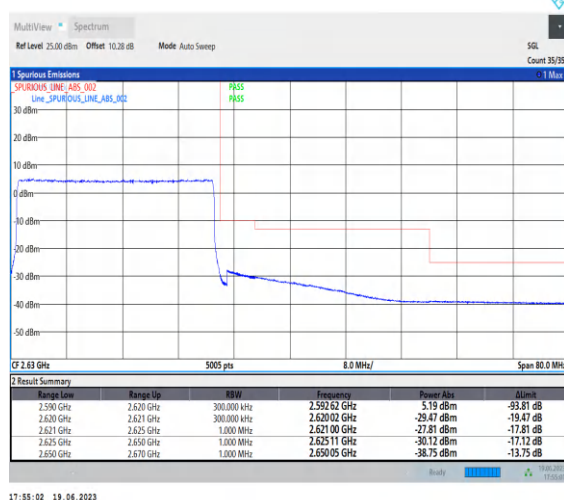
1-N38-PC2-30-30-H-3-CP-QPSK-Outer_Full-78@ 0-Ant0-1--PASS-see graph
