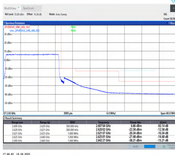
1-N38-PC2-30-20-H-3-CP-QPSK-Outer_Full-51@ 0-Ant0-1--PASS-see graph
