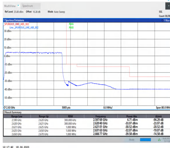
1-N38-PC3-30-30-H-3-DFT-PI2BPSK-Outer_Full-7 5@0-Ant0-1--PASS-see graph
