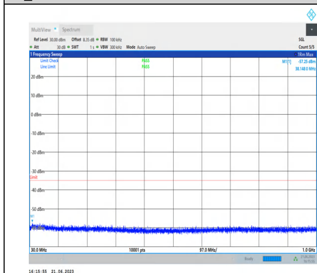
1-N38-PC3-30-40-M-1-N/A-DFT-PI2BPSK-Inner_1R B_Left-1@1-0.009-0.15-Ant0-0.13--76.68--55-PASS
