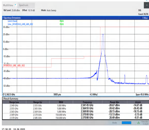
1-N38-PC2-30-15-L-1-CP-QPSK-Edge_1RB_Left-1@0-Ant0-1--PASS-see graph
