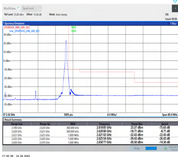
1-N38-PC2-30-30-H-2-CP-QPSK-Edge_1RB_Right-1@ 77-Ant0-1--PASS-see graph
