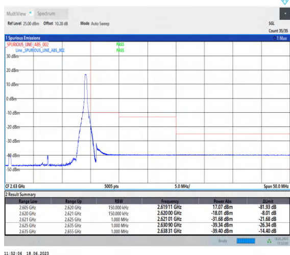
1-N38-PC3-30-15-H-5-CP-QPSK-Edge_1RB_Right-1 @37-Ant0-1--PASS-see graph
