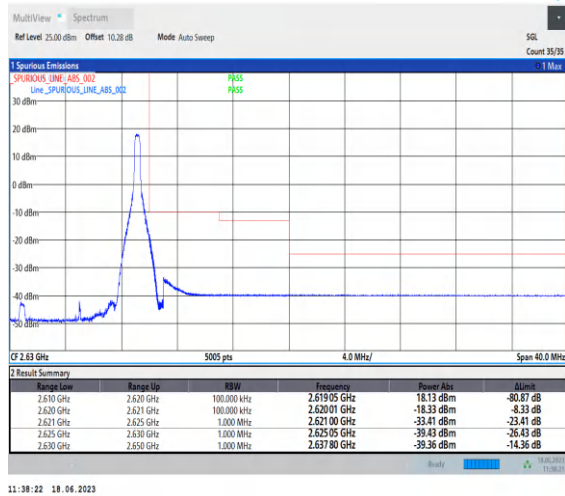
1-N38-PC3-30-10-H-2-DFT-PI2BPSK-Edge_1RB_Righ t-1@23-Ant0-1--PASS-see graph
