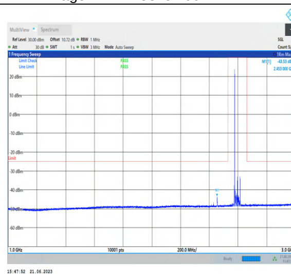
1-N38-PC2-30-40-M-1-N/A-DFT-QPSK-Edge_1RB_Left-1@0-1000-3000-Ant0-2755.40--43.53--25-PASS
