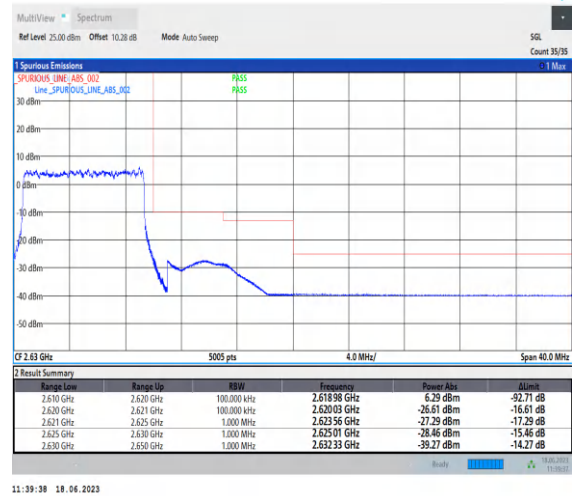
1-N38-PC3-30-10-H-3-DFT-PI2BPSK-Outer_Full-2 4@0-Ant0-1--PASS-see graph
