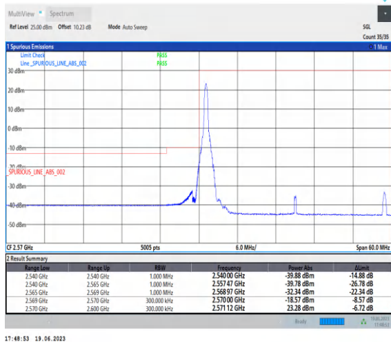
1-N38-PC2-30-30-L-1-CP-QPSK-Edge_1RB_Left-1@0 -Ant0-1--PASS-see graph
