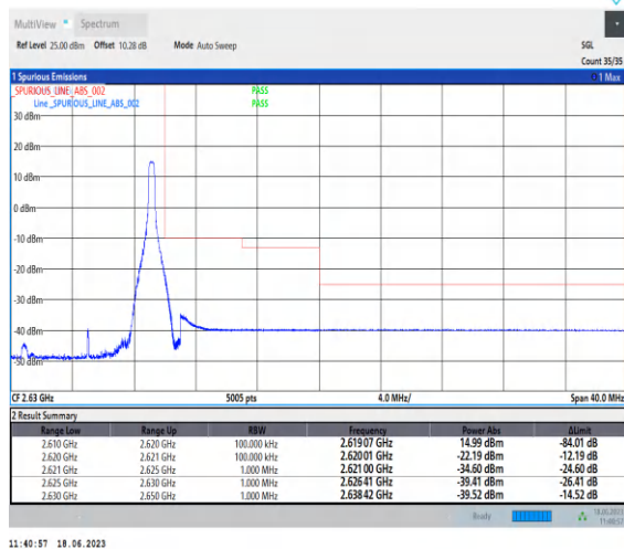
1-N38-PC3-30-10-H-5-CP-QPSK-Edge_1RB_Right-1 @23-Ant0-1--PASS-see graph
