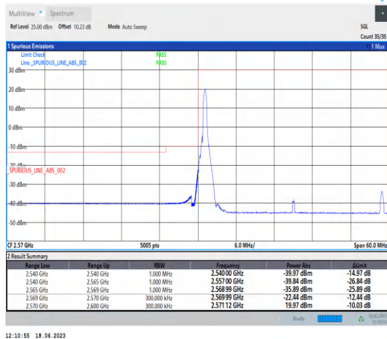
1-N38-PC3-30-30-L-4-CP-QPSK-Edge_1RB_Left-1@0-Ant0-1--PASS-see graph
