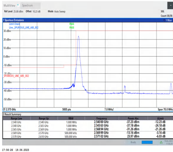
1-N38-PC2-30-40-L-1-CP-QPSK-Edge_1RB_Left-1@0-Ant0-1--PASS-see graph
