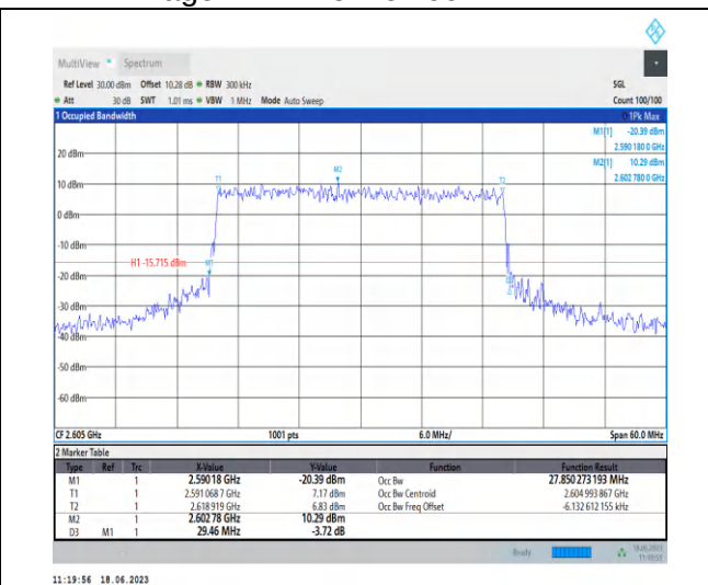
1-N38-PC3-30-30-H-7-CP-16QAM-Outer_Full-78@0-Ant0-27.85-29.460-≤30-PASS
