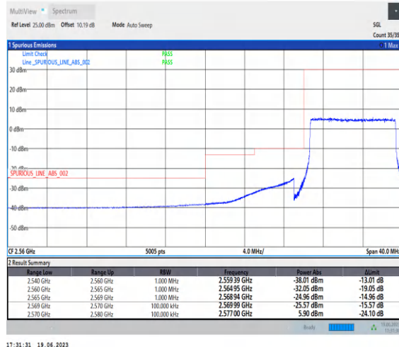
1-N38-PC2-30-10-L-3-CP-QPSK-Outer_Full-24@ 0-Ant0-1--PASS-see graph
