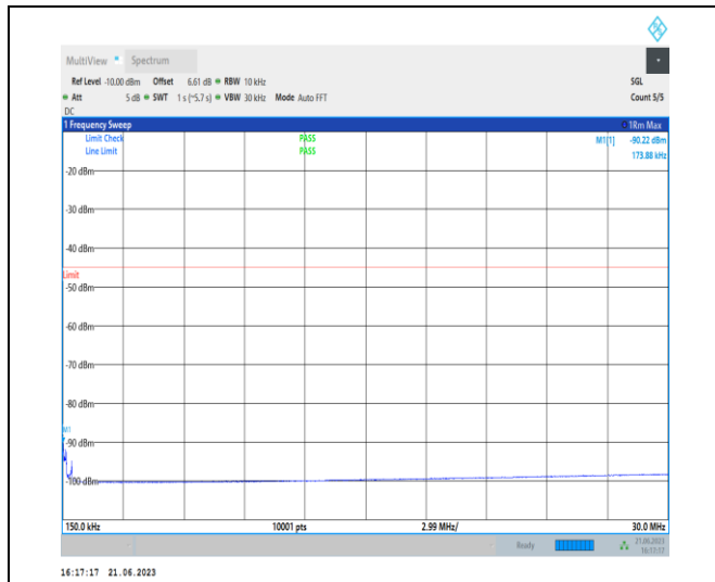
1-N38-PC3-30-40-H-1-N/A-DFT-PI2BPSK-Inner_1R B_Left-1@1-0.15-30-Ant0-18.84--90.22--45-PASS
