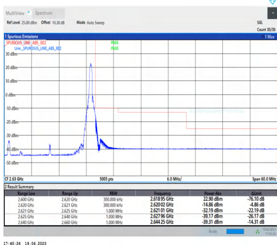
1-N38-PC2-30-20-H-2-CP-QPSK-Edge_1RB_Right-1@ 50-Ant0-1--PASS-see graph
