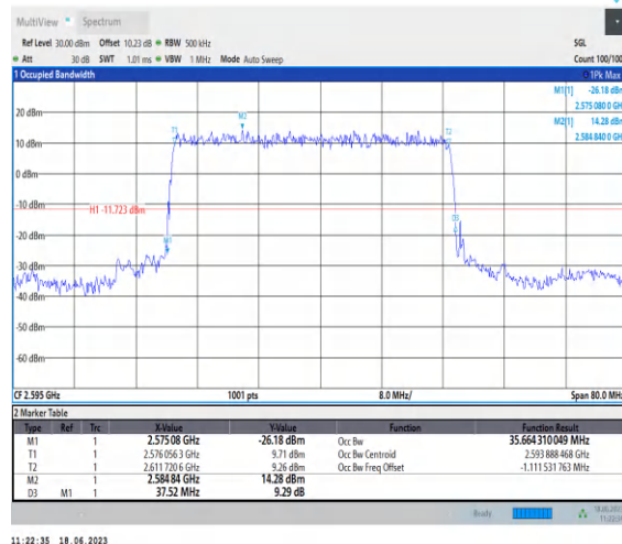
1-N38-PC3-30-40-M-1-DFT-PI2BPSK-Outer_Full-10 0@0-Ant0-35.664-37.520-≤40-PASS
