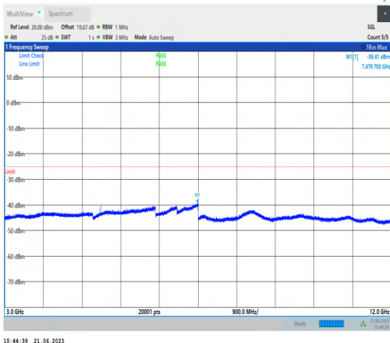
1-N38-PC2-30-40-L-1-N/A-DFT-QPSK-Edge_1RB_Left-1@0-3000-12000-Ant0-5218.95--39.41--25-PA SS
