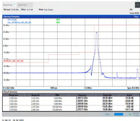
1-N38-PC3-30-15-L-1-DFT-PI2BPSK-Edge_1RB_Left-1@0-Ant0-1--PASS-see graph
