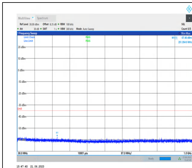
1-N38-PC2-30-40-M-1-N/A-DFT-QPSK-Edge_1RB_Left-1@0-30-1000-Ant0-36.98--57.40--35-PASS
