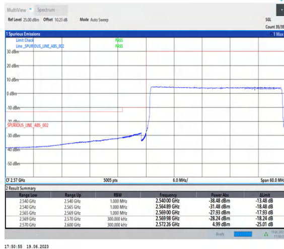
1-N38-PC2-30-30-L-3-CP-QPSK-Outer_Full-78@ 0-Ant0-1--PASS-see graph
