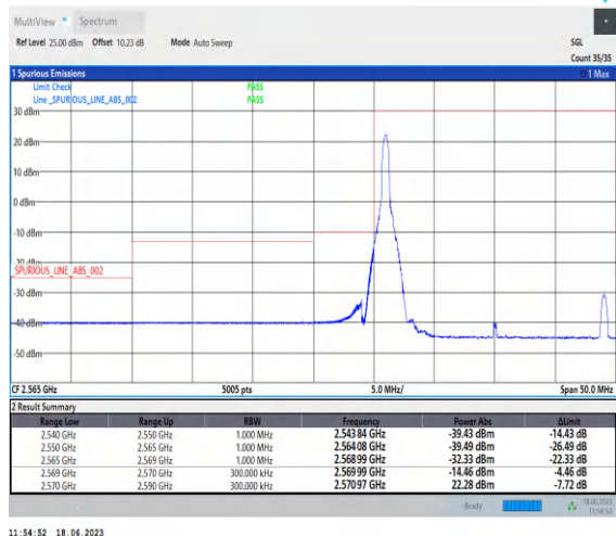
1-N38-PC3-30-20-L-1-DFT-PI2BPSK-Edge_1RB_Left-1@0-Ant0-1--PASS-see graph
