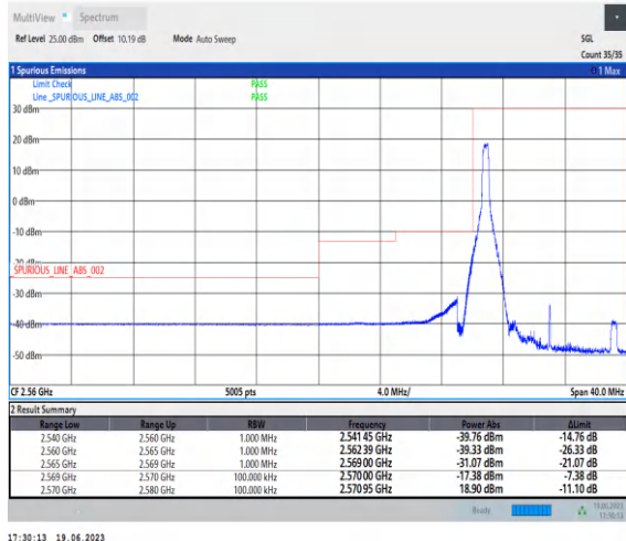
1-N38-PC2-30-10-L-1-CP-QPSK-Edge_1RB_Left-1@0 -Ant0-1--PASS-see graph
