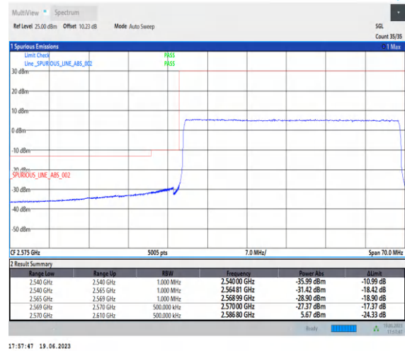
1-N38-PC2-30-40-L-3-CP-QPSK-Outer_Full-106@0-Ant0-1--PASS-see graph
