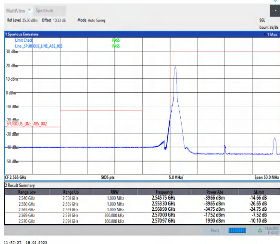
1-N38-PC3-30-20-L-4-CP-QPSK-Edge_1RB_Left-1@0-Ant0-1--PASS-see graph
