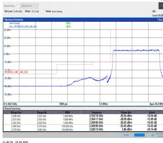
1-N38-PC3-30-15-L-3-DFT-PI2BPSK-Outer_Full-36@0-Ant0-1--PASS-see graph
