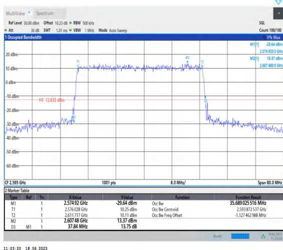
1-N38-PC3-30-40-M-2-DFT-QPSK-Outer_Full-100@ 0-Ant0-35.689-37.840-≤40-PASS
