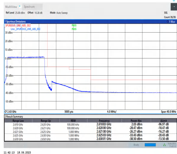
1-N38-PC3-30-10-H-6-CP-QPSK-Outer_Full-24@ 0-Ant0-1--PASS-see graph
