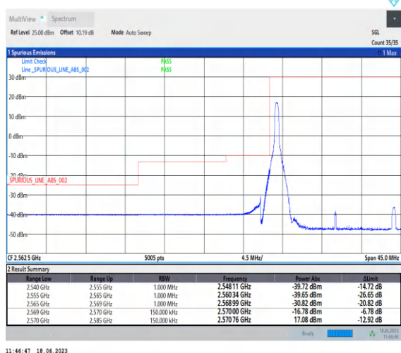
1-N38-PC3-30-15-L-4-CP-QPSK-Edge_1RB_Left-1@0-Ant0-1--PASS-see graph
