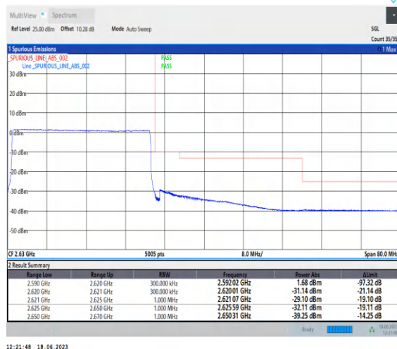
1-N38-PC3-30-30-H-6-CP-QPSK-Outer_Full-78@ 0-Ant0-1--PASS-see graph
