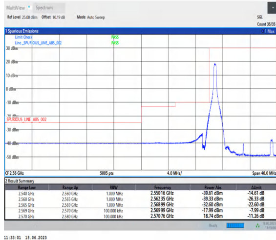
1-N38-PC3-30-10-L-1-DFT-PI2BPSK-Edge_1RB_Left-1@0-Ant0-1--PASS-see graph
