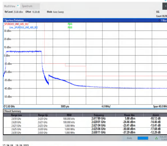
1-N38-PC2-30-10-H-3-CP-QPSK-Outer_Full-24@ 0-Ant0-1--PASS-see graph
