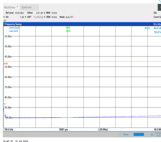
1-N38-PC2-30-40-M-1-N/A-DFT-QPSK-Edge_1RB_L eft-1@0-0.15-30-Ant0-0.16--90.07--45-PASS
