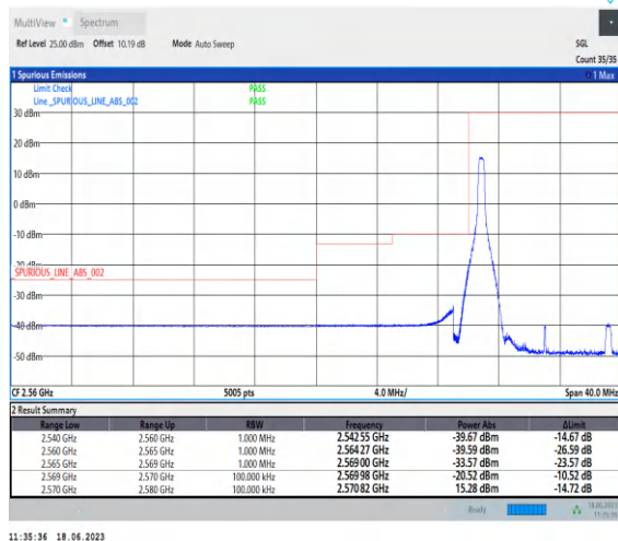
1-N38-PC3-30-10-L-4-CP-QPSK-Edge_1RB_Left-1@0-Ant0-1--PASS-see graph
