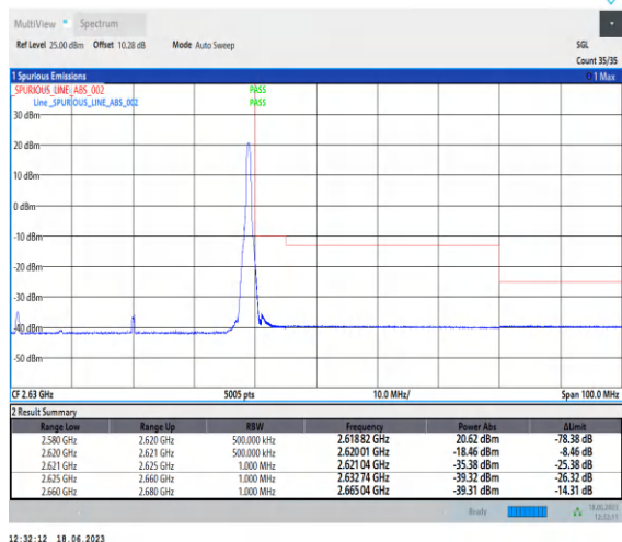
1-N38-PC3-30-40-H-5-CP-QPSK-Edge_1RB_Right-1 @105-Ant0-1--PASS-see graph
