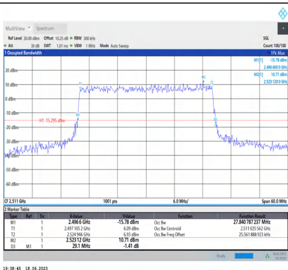
1-N41-PC3-30-30-L-6-CP-QPSK-Outer_Full-78@0-A Ant0-27.841-29.100-≤30-PASS
