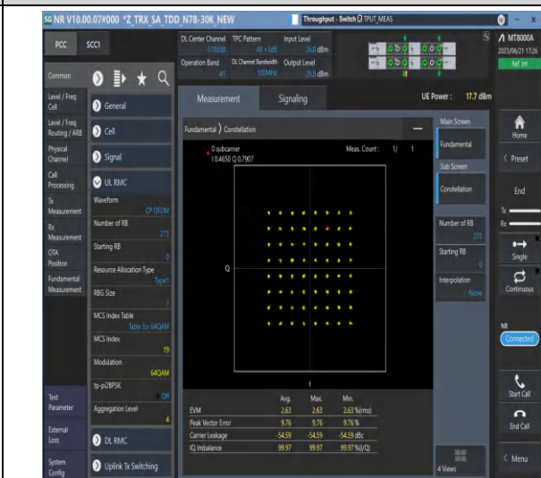
1-N41-PC3-30-100-M-8-CP-64QAM-Outer_Full-273 @0-Ant0-see graph-PASS
