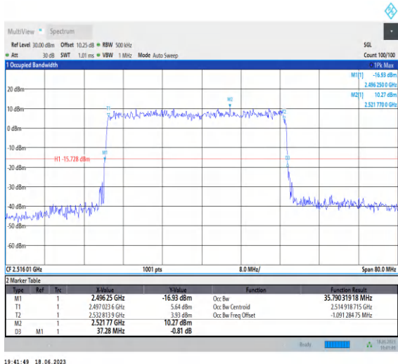
1-N41-PC3-30-40-L-5-DFT-256QAM-Outer_Full-100 @0-Ant0-35.79-37.280-≤40-PASS
