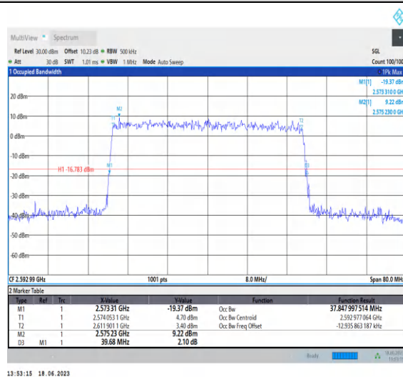
1-N41-PC3-30-40-M-9-CP-256QAM-Outer_Full-106@ 0-Ant0-37.848-39.680-≤40-PASS
