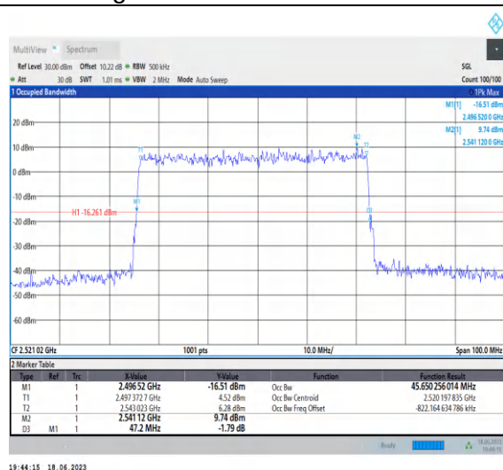
1-N41-PC3-30-50-L-5-DFT-256QAM-Outer_Full-128 @0-Ant0-45.65-47.200-≤50-PASS
