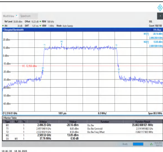
1-N41-PC3-30-40-L-3-DFT-16QAM-Outer_Full-100 @0-Ant0-35.802-37.760-≤40-PASS
