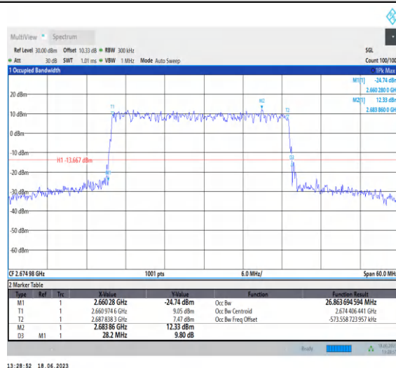
1-N41-PC3-30-30-H-3-DFT-16QAM-Outer_Full-75@ 0-Ant0-26.864-28.200-≤30-PASS
