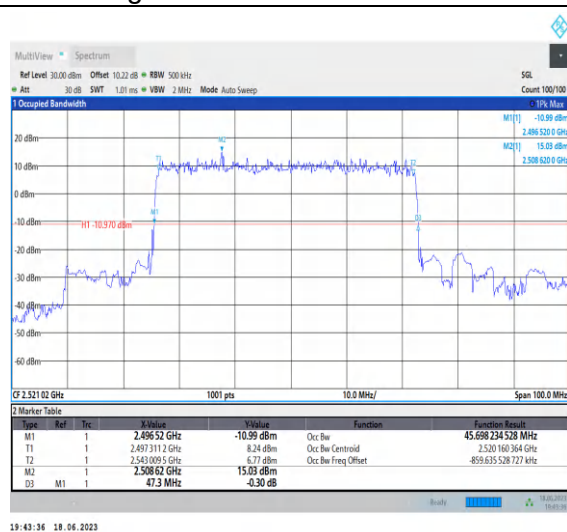
1-N41-PC3-30-50-L-1-DFT-PI2BPSK-Outer_Full-128 @0-Ant0-45.698-47.300-≤50-PASS
