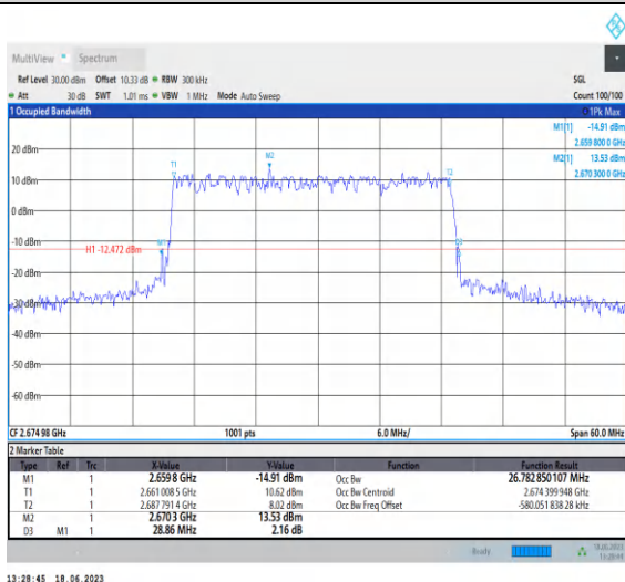
1-N41-PC3-30-30-H-2-DFT-QPSK-Outer_Full-75@0- Ant0-26.783-28.860-≤30-PASS
