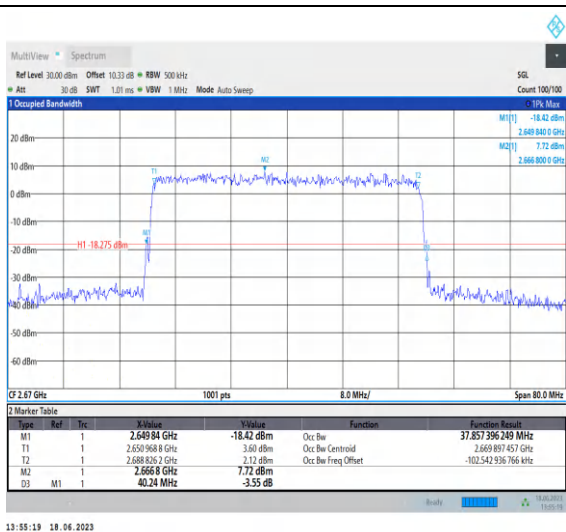
1-N41-PC3-30-40-H-9-CP-256QAM-Outer_Full-106 @0-Ant0-37.857-40.240-≤40-PASS
