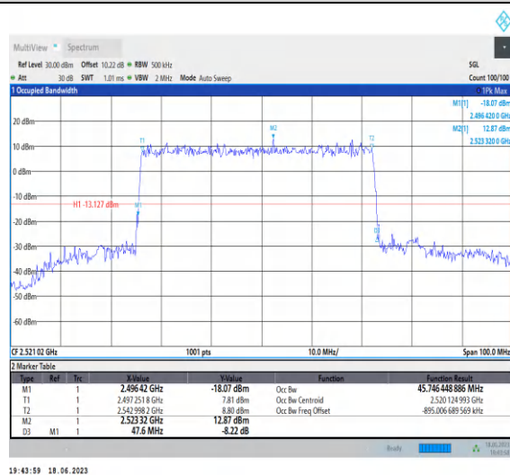
1-N41-PC3-30-50-L-3-DFT-16QAM-Outer_Full-128 @0-Ant0-45.746-47.600-≤50-PASS
