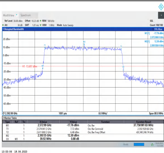
1-N41-PC3-30-40-M-8-CP-64QAM-Outer_Full-106@ 0-Ant0-37.759-39.920-≤40-PASS
