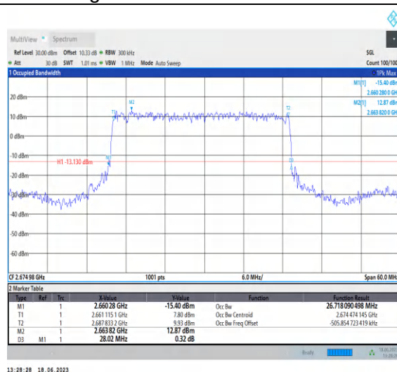
1-N41-PC3-30-30-H-1-DFT-PI2BPSK-Outer_Full-75 @0-Ant0-26.718-28.020-≤30-PASS
