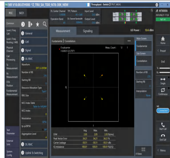
1-N41-PC3-30-100-M-2-DFT-QPSK-Outter_Full-270 @0-Ant0-see graph-PASS
