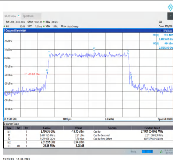
1-N41-PC3-30-30-L-9-CP-256QAM-Outer_Full-78@0-A Ant0-27.801-29.580-≤30-PASS
