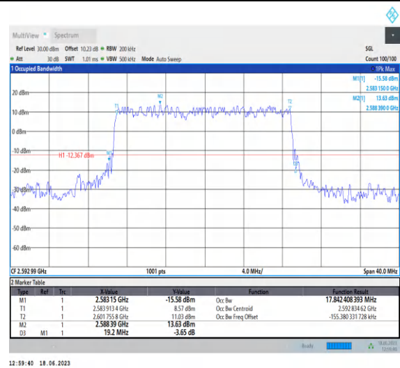
1-N41-PC3-30-20-M-1-DFT-PI2BPSK-Outer_Full-50 @0-Ant0-17.842-19.200-≤20-PASS
