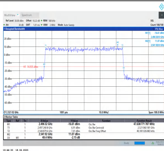
1-N41-PC3-30-50-L-7-CP-16QAM-Outer_Full-133@ 0-Ant0-47.639-49.400-≤50-PASS
