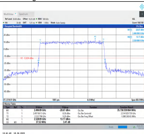
1-N41-PC3-30-40-L-4-DFT-64QAM-Outer_Full-100 @0-Ant0-35.737-37.520-≤40-PASS
