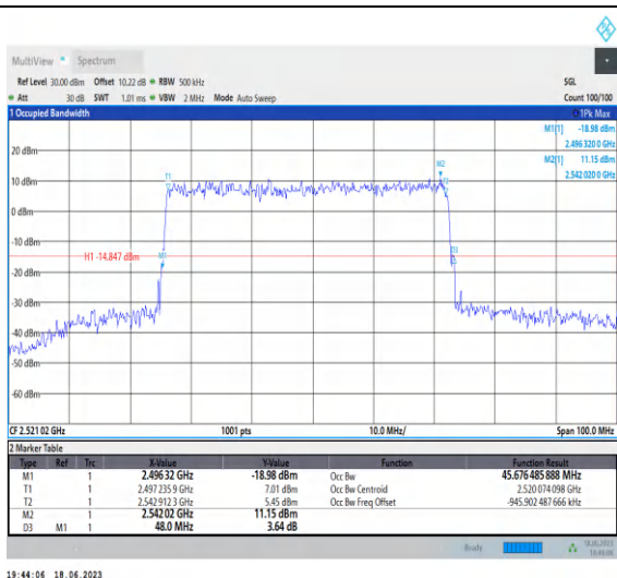
1-N41-PC3-30-50-L-4-DFT-64QAM-Outer_Full-128 @0-Ant0-45.676-48.000-≤50-PASS
