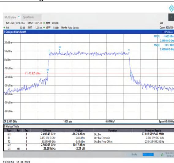
1-N41-PC3-30-30-L-7-CP-16QAM-Outer_Full-78@0-A Ant0-27.819-29.280-≤30-PASS
