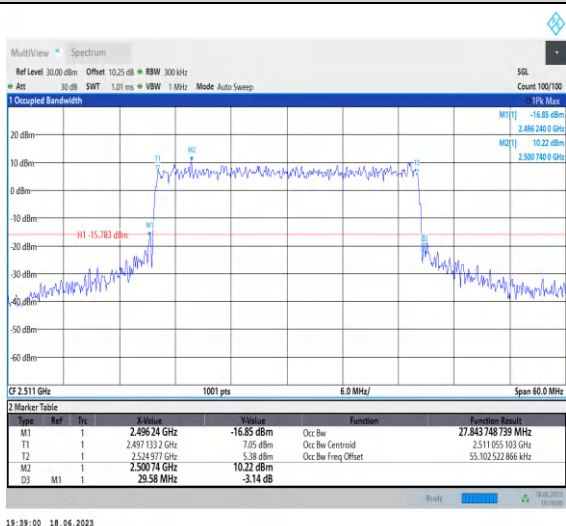
1-N41-PC3-30-30-L-8-CP-64QAM-Outer_Full-78@0-A Ant0-27.844-29.580-≤30-PASS
