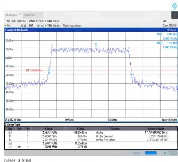
1-N41-PC3-30-20-M-3-DFT-16QAM-Outer_Full-50@ 0-Ant0-17.754-18.960-≤20-PASS
