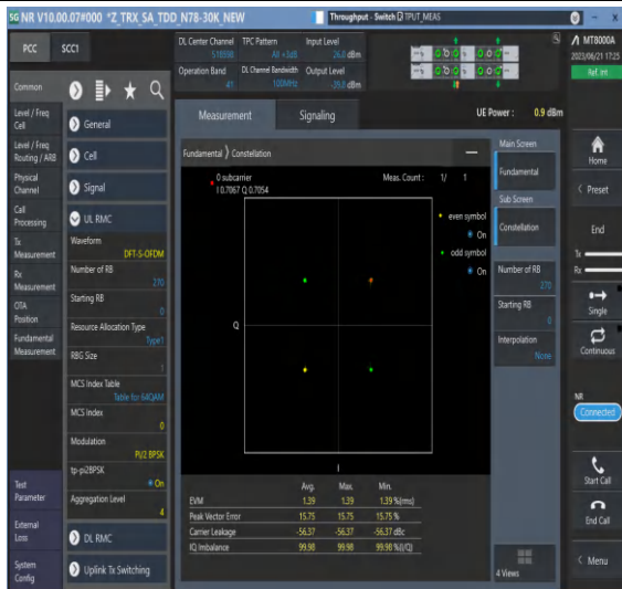
1-N41-PC3-30-100-M-1-DFT-PI2BPSK-Outter_Full-27 0@0-Ant0-see graph-PASS
