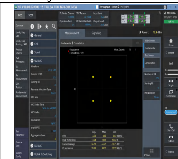
1-N41-PC3-30-100-M-6-CP-QPSK-Outer_Full-273 @0-Ant0-see graph-PASS
