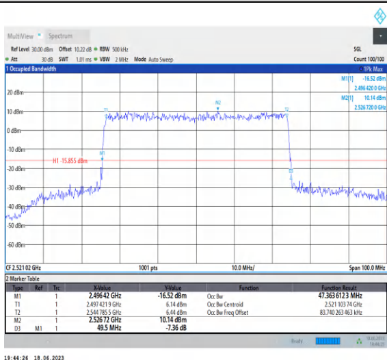
1-N41-PC3-30-50-L-6-CP-QPSK-Outer_Full-133@0- Ant0-47.364-49.500-≤50-PASS
