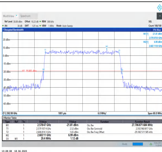
1-N41-PC3-30-30-M-9-CP-256QAM-Outer_Full-78@ 0-Ant0-27.707-29.400-≤30-PASS
