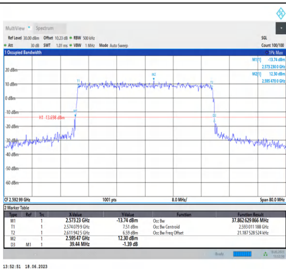
1-N41-PC3-30-40-M-6-CP-QPSK-Outer_Full-106@0 -Ant0-37.863-39.440-≤40-PASS
