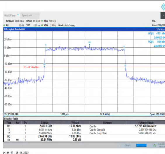
1-N41-PC3-30-60-H-2-DFT-QPSK-Outer_Full-162@ 0-Ant0-57.785-59.640-≤60-PASS
