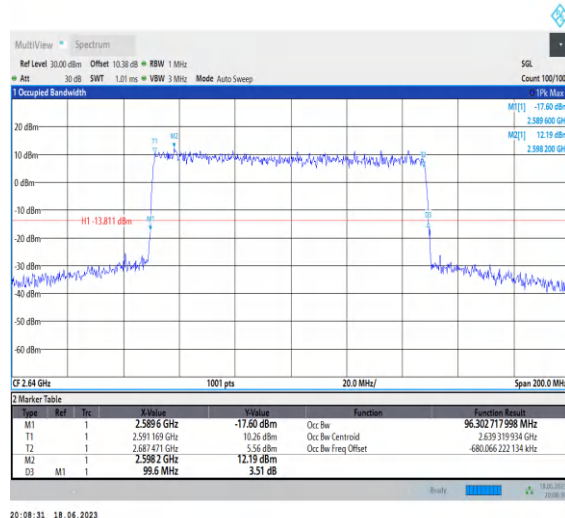
1-N41-PC3-30-100-H-3-DFT-16QAM-Out-270 @0-Ant0-96.303-99.600-≤100-PASS
