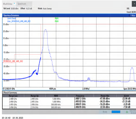
1-N41-PC3-30-20-L-1-DFT-PI2BPSK-Edge_1RB_Left-1@0-Ant0-1--PASS-see graph
