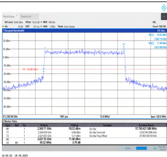
1-N41-PC3-30-60-M-8-CP-64QAM-Outer_Full-162@ 0-Ant0-57.766-59.520-≤60-PASS
