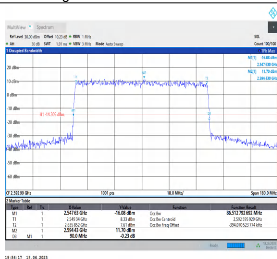
1-N41-PC3-30-90-M-4-DFT-64QAM-Outer_Full-243 @0-Ant0-86.513-90.000-≤90-PASS
