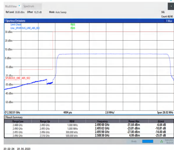
1-N41-PC3-30-20-L-6-CP-QPSK-Outer_Full-51@0-Ant0-1--PASS-see graph
