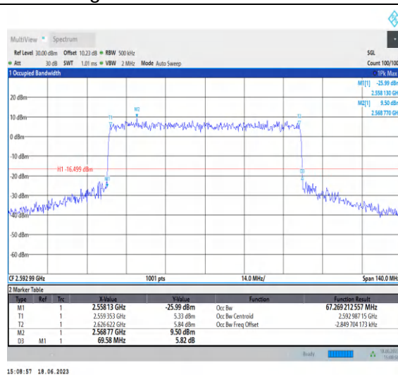
1-N41-PC3-30-70-M-6-CP-QPSK-Out_ Full-189@0 -Ant0-67.269-69.580-≤70-PASS
