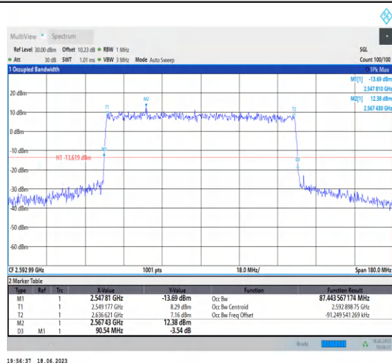
1-N41-PC3-30-90-M-6-CP-QPSK-Outer_Full-245@0 -Ant0-87.444-90.540-≤90-PASS
