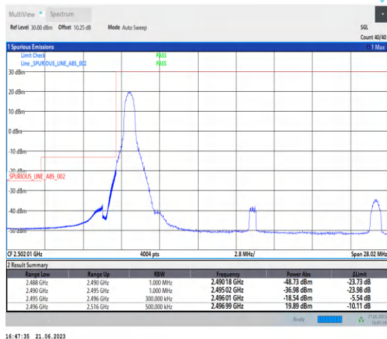
1-N41-PC3-30-20-L-4-CP-QPSK-Edge_1RB_Left-1@0-Ant0-1--PASS-see graph
