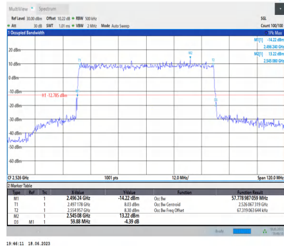
1-N41-PC3-30-60-L-2-DFT-QPSK-Outet_Full-162@ 0-Ant0-57.779-59.880-≤60-PASS
