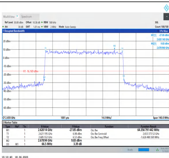
1-N41-PC3-30-70-H-4-DFT-64QAM-Outer_Full-180 @0-Ant0-64.357-66.500-≤70-PASS
