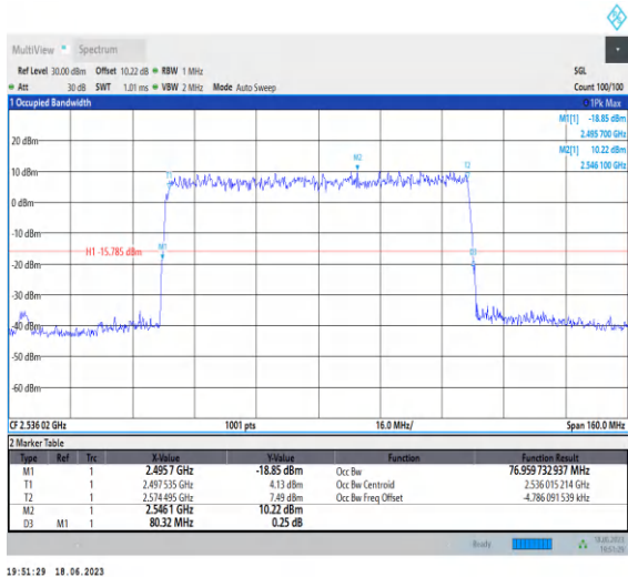
1-N41-PC3-30-80-L-5-DFT-256QAM-Outer_Full-216 @0-Ant0-76.96-80.320-≤80-PASS
