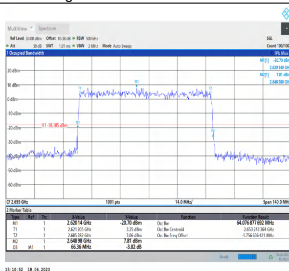
1-N41-PC3-30-70-H-5-DFT-256QAM-Outer_Full-180 @0-Ant0-64.077-66.360-≤70-PASS
