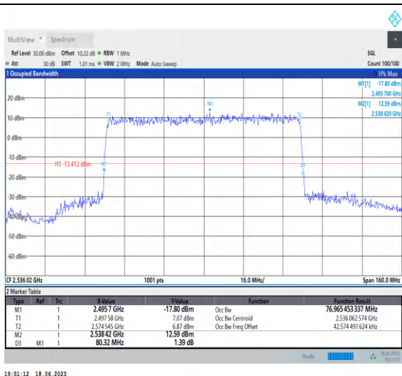
1-N41-PC3-30-80-L-3-DFT-16QAM-Outer_Full-216 @0-Ant0-76.965-80.320-≤80-PASS
