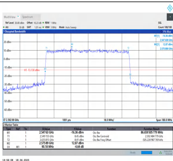
1-N41-PC3-30-90-M-3-DFT-16QAM-Outer_Full-243 @0-Ant0-86.66-90.180-≤90-PASS
