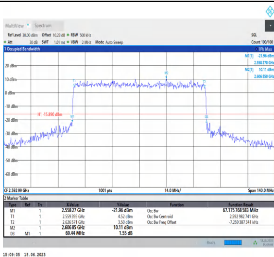
1-N41-PC3-30-70-M-7-CP-16QAM-Out_ Full-189@0-Ant0-67.176-69.440-≤70-PASS
