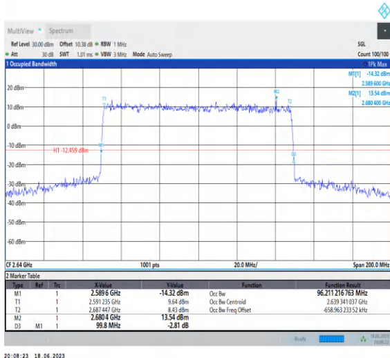
1-N41-PC3-30-100-H-2-DFT-QPSK-Out-270 @0-Ant0-96.211-99.800-≤100-PASS
