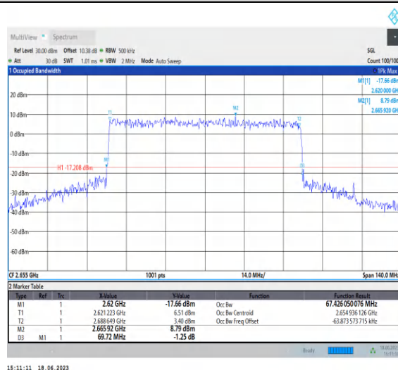
1-N41-PC3-30-70-H-7-CP-16QAM-Outer_Full-189@0 -Ant0-67.426-69.720-≤70-PASS
