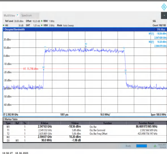
1-N41-PC3-30-90-M-5-DFT-256QAM-Outer_Full-243 @0-Ant0-86.47-90.000-≤90-PASS
