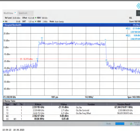
1-N41-PC3-30-70-M-8-CP-64QAM-Out_ Full-189@0-Ant0-67.344-69.860-≤70-PASS
