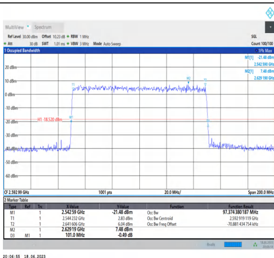
1-N41-PC3-30-100-M-9-CP-256QAM-Out-273 @0-Ant0-97.374-101.000-≤100-PASS
