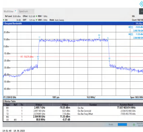
1-N41-PC3-30-80-L-6-CP-QPSK-Outer_Full-217@0-Ant0-77.657-80.800-≤80-PASS
