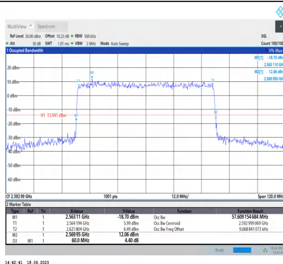
1-N41-PC3-30-60-M-3-DFT-16QAM-Outer_Full-162 @0-Ant0-57.609-60.000-≤60-PASS
