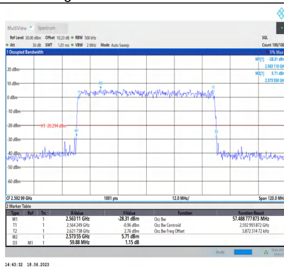
1-N41-PC3-30-60-M-9-CP-256QAM-Outer_Full-162 @0-Ant0-57.489-59.880-≤60-PASS
