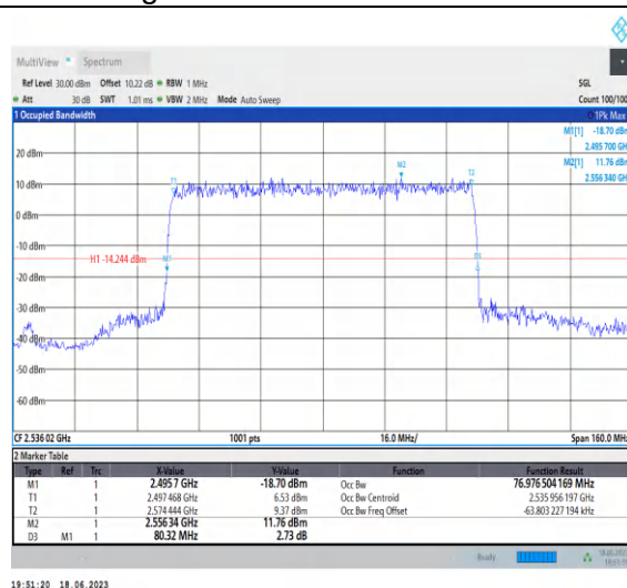
1-N41-PC3-30-80-L-4-DFT-64QAM-Outer_Full-216 @0-Ant0-76.977-80.320-≤80-PASS
