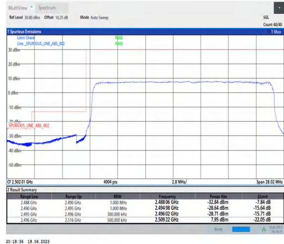
1-N41-PC3-30-20-L-3-DFT-PI2BPSK-Outer_Full-50@0-Ant0-1--PASS-see graph
