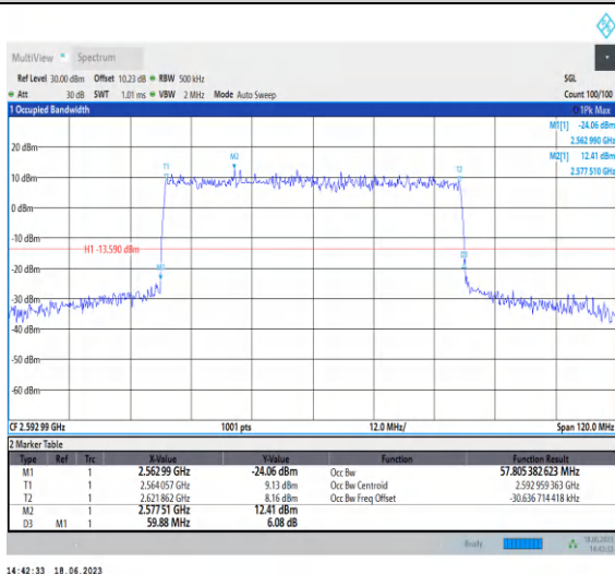
1-N41-PC3-30-60-M-2-DFT-QPSK-Outer_Full-162@ 0-Ant0-57.805-59.880-≤60-PASS
