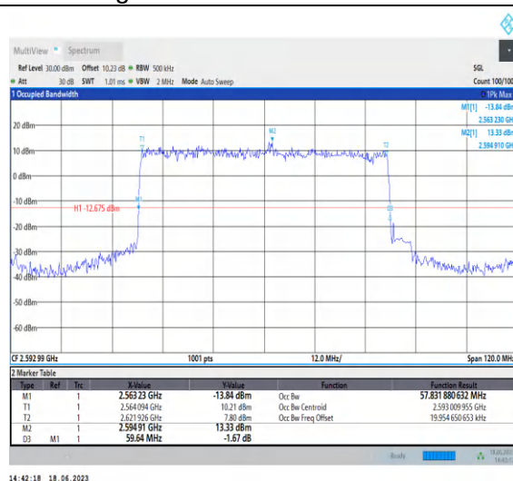
1-N41-PC3-30-60-M-1-DFT-PI2BPSK-Outer_Full-16 2@0-Ant0-57.832-59.640-≤60-PASS
