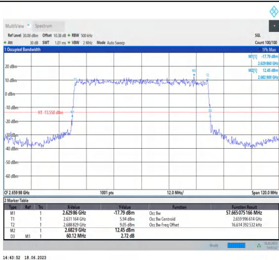
1-N41-PC3-30-60-H-1-DFT-PI2BPSK-Outer_Full-162@ 2@0-Ant0-57.665-60.120-≤60-PASS
