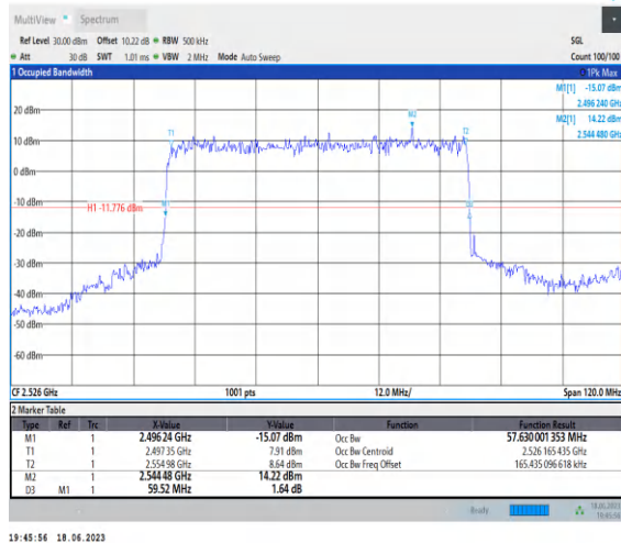
1-N41-PC3-30-60-L-1-DFT-PI2BPSK-Outet_Full-162 @0-Ant0-57.63-59.520-≤60-PASS
