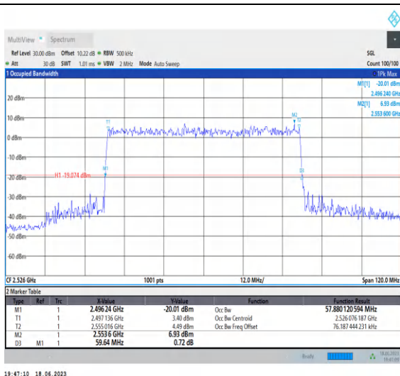
1-N41-PC3-30-60-L-9-CP-256QAM-Outer_Full-162 @0-Ant0-57.88-59.640-≤60-PASS
