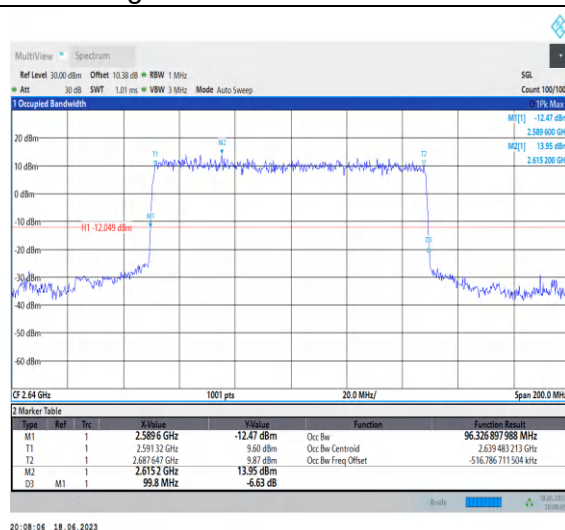
1-N41-PC3-30-100-H-1-DFT-PI2BPSK-Out-270 @0-Ant0-96.327-99.800-≤100-PASS
