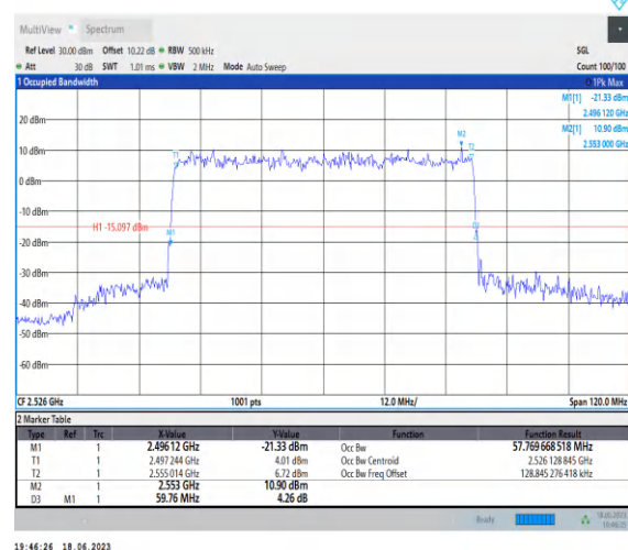
1-N41-PC3-30-60-L-4-DFT-64QAM-Outet_Full-162 @0-Ant0-57.77-59.760-≤60-PASS
