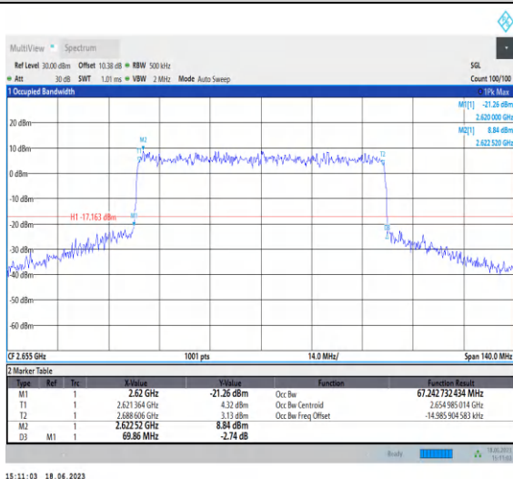
1-N41-PC3-30-70-H-6-CP-QPSK-Outer_Full-189@0 -Ant0-67.243-69.860-≤70-PASS
