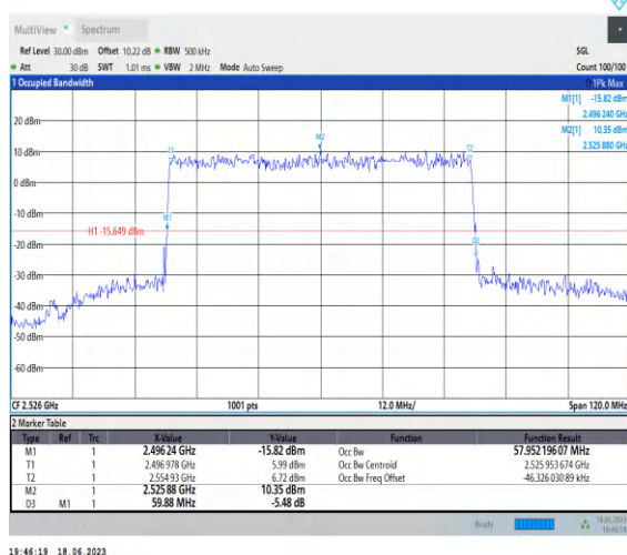
1-N41-PC3-30-60-L-3-DFT-16QAM-Outet_Full-162 @0-Ant0-57.952-59.880-≤60-PASS
