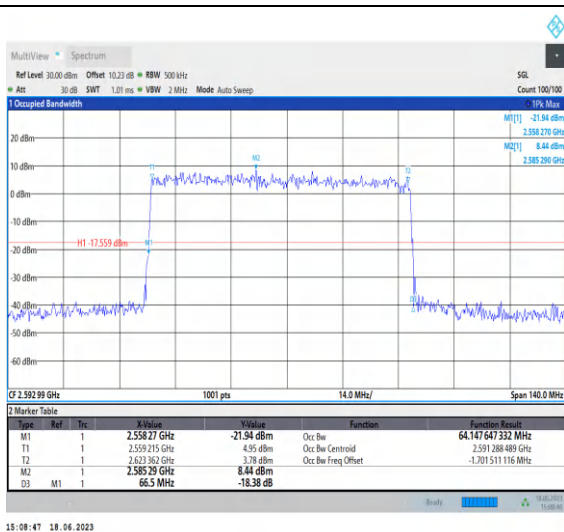
1-N41-PC3-30-70-M-5-DFT-256QAM-Out_ Full-180 @0-Ant0-64.148-66.500-≤70-PASS
