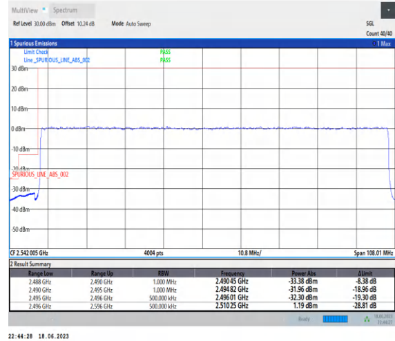
1-N41-PC3-30-100-L-3-DFT-PI2BPSK-Outer_Full-270@0-Ant0-1--PASS-see graph
