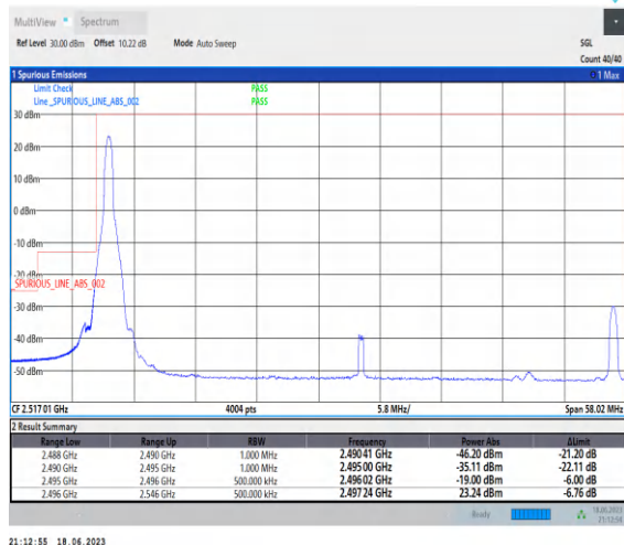
1-N41-PC3-30-50-L-1-DFT-PI2BPSK-Edge_1RB_Left-1@0-Ant0-1--PASS-see graph
