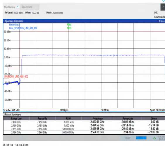
1-N41-PC2-30-70-L-3-CP-QPSK-Outer_Full-189@0-Ant0-1--PASS-see graph
