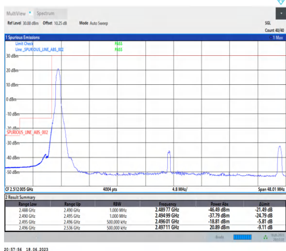
1-N41-PC3-30-40-L-4-CP-QPSK-Edge_1RB_Left-1@0-Ant0-1--PASS-see graph
