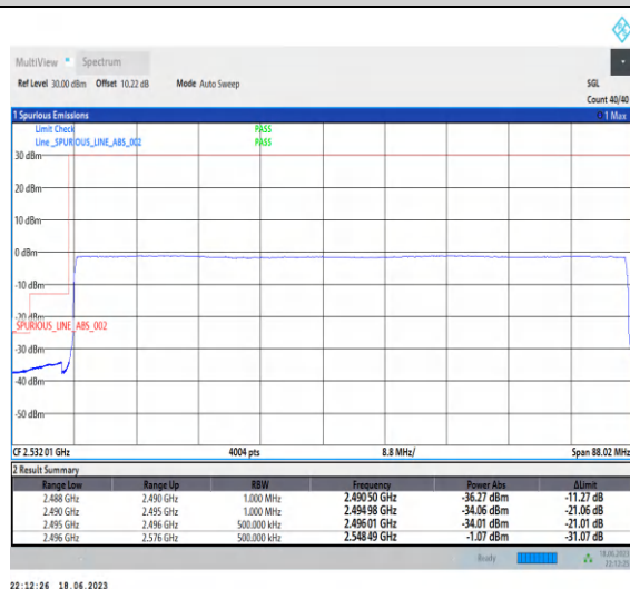
1-N41-PC3-30-80-L-6-CP-QPSK-Outer_Full-217@0-Ant0-1--PASS-see graph
