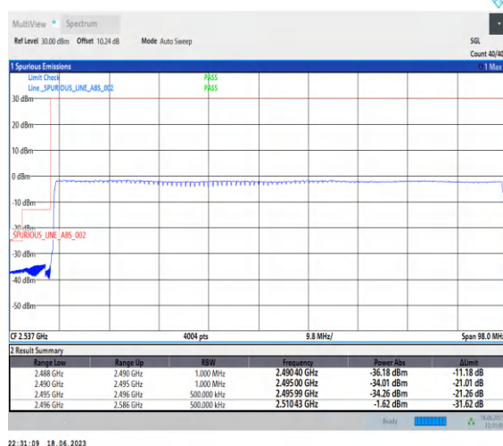
1-N41-PC3-30-90-L-6-CP-QPSK-Outer_Full-245@0-Ant0-1--PASS-see graph
