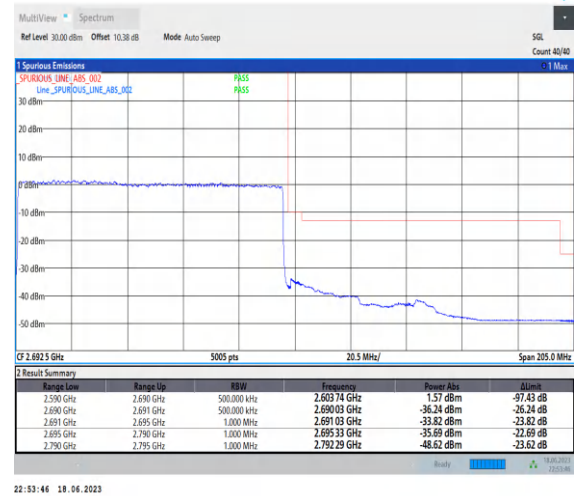
1-N41-PC3-30-100-H-3-DFT-PI2BPSK-Outer_Full- 270@0-Ant0-1--PASS-see graph
