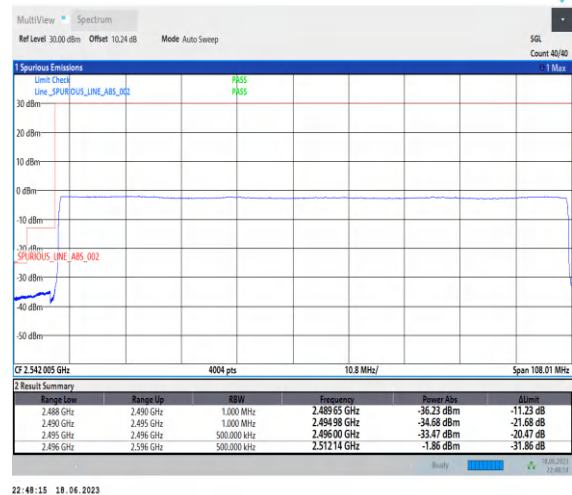
1-N41-PC3-30-100-L-6-CP-QPSK-Outer_Full-273@0-Ant0-1--PASS-see graph
