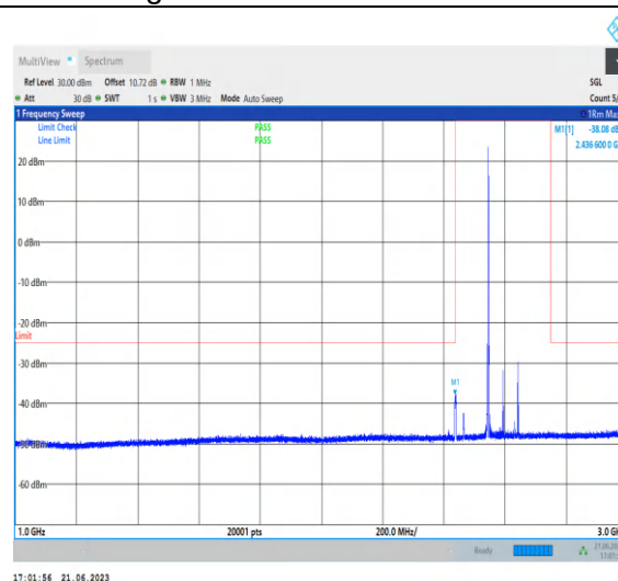
1-N41-PC3-30-100-M-1-N/A-DFT-PI2BPSK-Inner_1R B_Left-1@1-1000-3000-Ant0-2793.50--38.08--25-PA SS
