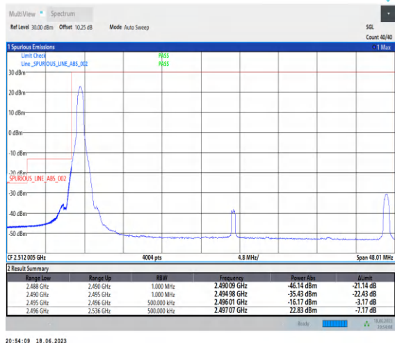
1-N41-PC3-30-40-L-1-DFT-PI2BPSK-Edge_1RB_Left-1@0-Ant0-1--PASS-see graph
