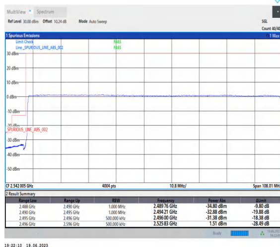
1-N41-PC2-30-100-L-3-CP-QPSK-Outer_Full-273 @0-Ant0-1--PASS-see graph
