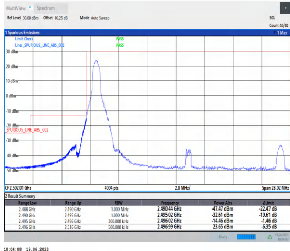
1-N41-PC2-30-20-L-1-CP-QPSK-Edge_1RB_Left-1@0 -Ant0-1--PASS-see graph
