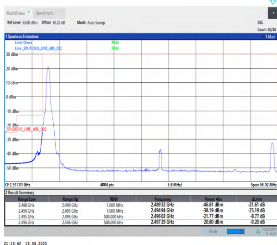
1-N41-PC3-30-50-L-4-CP-QPSK-Edge_1RB_Left-1@0-Ant0-1--PASS-see graph
