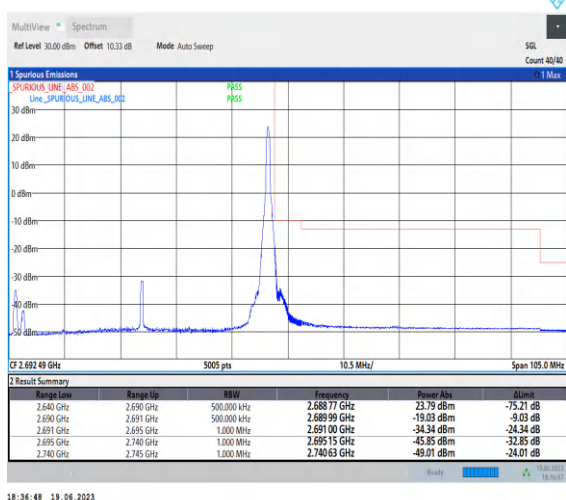
1-N41-PC2-30-50-H-2-CP-QPSK-Edge_1RB_Right-1@132-Ant0-1--PASS-see graph
