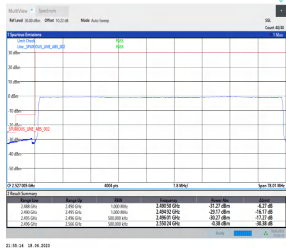
1-N41-PC3-30-70-L-6-CP-QPSK-Outer_Full-189@0-Ant0-1--PASS-see graph
