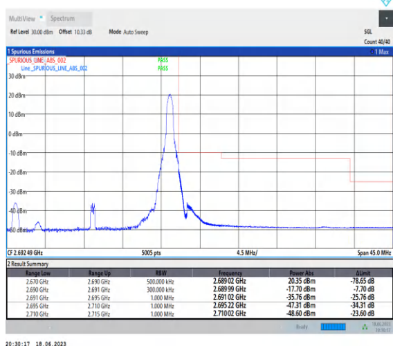
1-N41-PC3-30-20-H-5-CP-QPSK-Edge_1RB_Right-1@50-Ant0-1--PASS-see graph
