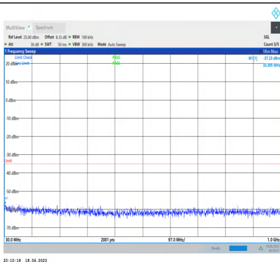
1-N41-PC3-30-100-M-1-N/A-DFT-PI2BPSK-Inner_1 RB_Left-1@1-30-1000-Ant0-33.40--57.23--35-PASS
