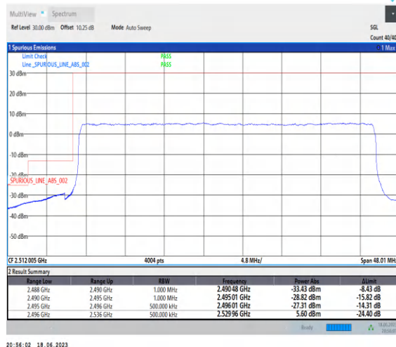
1-N41-PC3-30-40-L-3-DFT-PI2BPSK-Outer_Full-100@0-Ant0-1--PASS-see graph
