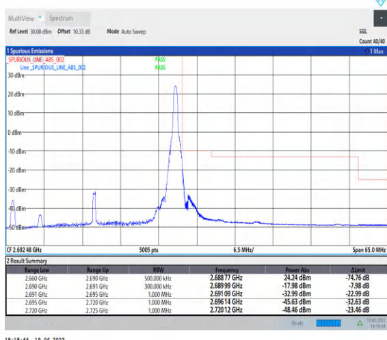
1-N41-PC2-30-30-H-2-CP-QPSK-Edge_1RB_Right-1 @77-Ant0-1--PASS-see graph
