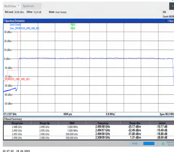
1-N41-PC3-30-90-L-3-DFT-PI2BPSK-Outer_Full-243@0-Ant0-1--PASS-see graph
