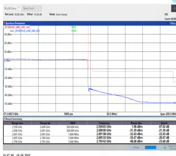
1-N41-PC2-30-100-H-3-CP-QPSK-Outer_Full-273 @0-Ant0-1--PASS-see graph
