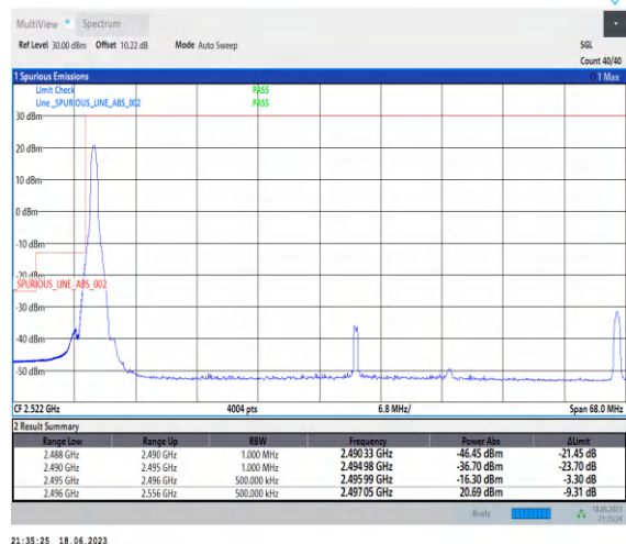
1-N41-PC3-30-60-L-4-CP-QPSK-Edge_1RB_Left-1@0 -Ant0-1--PASS-see graph
