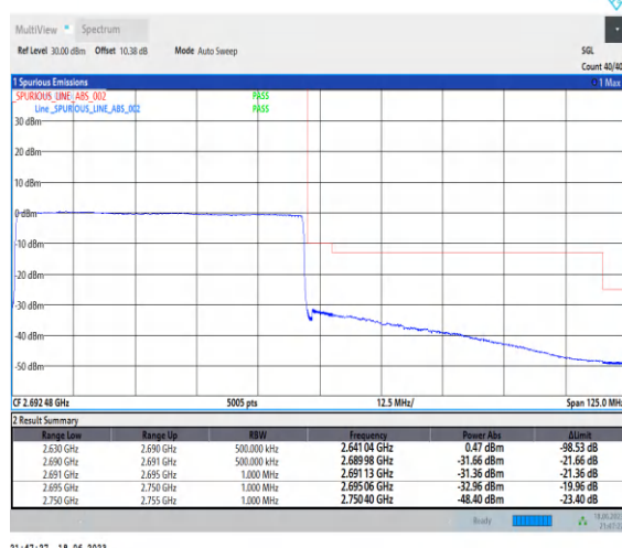
1-N41-PC3-30-60-H-6-CP-QPSK-Outer_Full-162 @0-Ant0-1--PASS-see graph
