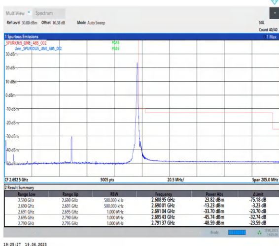
1-N41-PC2-30-100-H-2-CP-QPSK-Edge_1RB_Right-1 @272-Ant0-1--PASS-see graph
