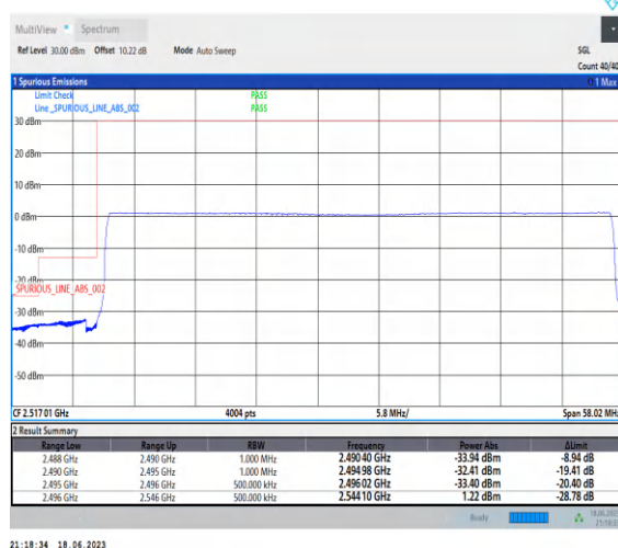
1-N41-PC3-30-50-L-6-CP-QPSK-Outer_Full-133@0-Ant0-1--PASS-see graph
