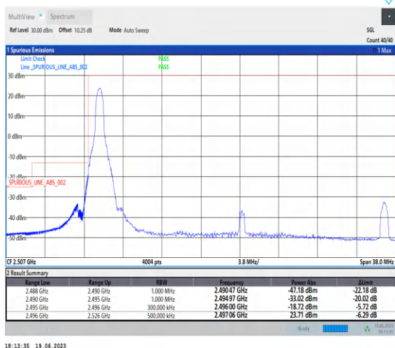
1-N41-PC2-30-30-L-1-CP-QPSK-Edge_1RB_Left-1@0 -Ant0-1--PASS-see graph
