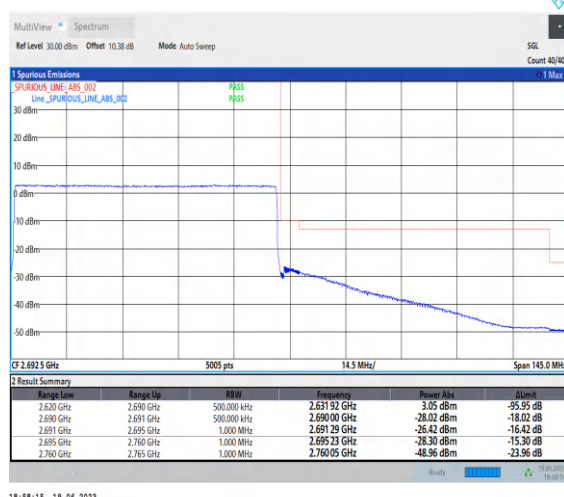
1-N41-PC2-30-70-H-3-CP-QPSK-Outer_Full-189@0-Ant0-1--PASS-see graph
