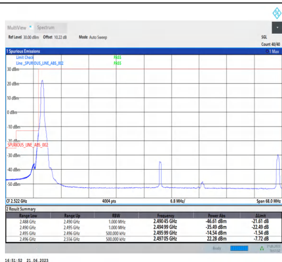
1-N41-PC3-30-60-L-1-DFT-PI2BPSK-Edge_1RB_Left- 1@0-Ant0-1--PASS-see graph
