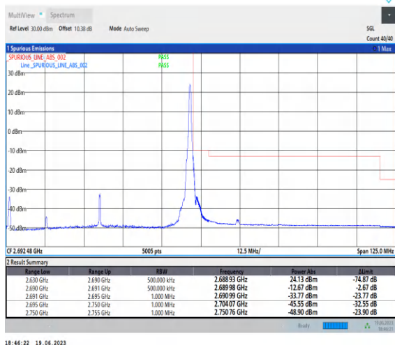
1-N41-PC2-30-60-H-2-CP-QPSK-Edge_1RB_Right-1 @161-Ant0-1--PASS-see graph
