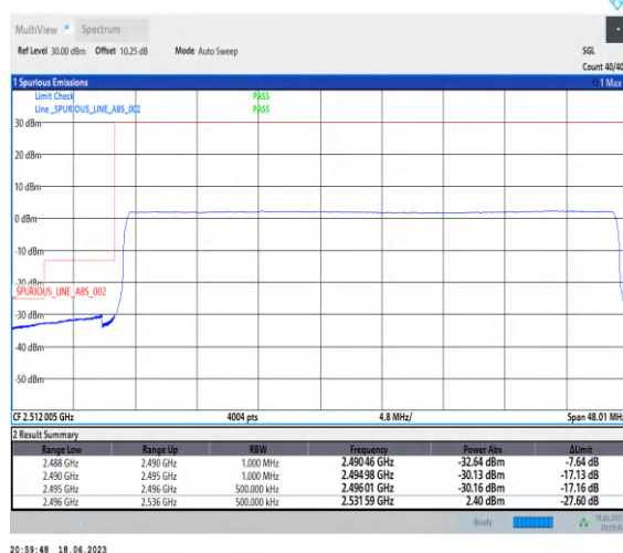
1-N41-PC3-30-40-L-6-CP-QPSK-Outer_Full-106@0-Ant0-1--PASS-see graph
