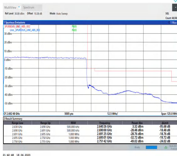
1-N41-PC3-30-60-H-3-DFT-PI2BPSK-Outer_Full-1 62@0-Ant0-1--PASS-see graph
