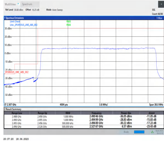
1-N41-PC3-30-30-L-3-DFT-PI2BPSK-Outer_Full-75@0-Ant0-1--PASS-see graph
