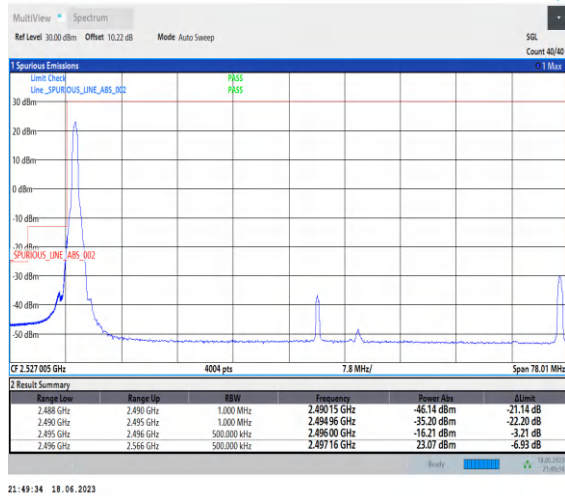
1-N41-PC3-30-70-L-1-DFT-PI2BPSK-Edge_1RB_Left-1@0-Ant0-1--PASS-see graph
