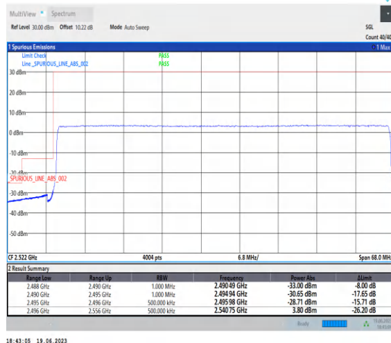
1-N41-PC2-30-60-L-3-CP-QPSK-Outer_Full-162 @0-Ant0-1--PASS-see graph
