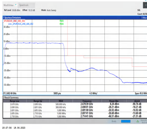
1-N41-PC3-30-20-H-3-DFT-PI2BPSK-Outer_Full-50@0-Ant0-1--PASS-see graph
