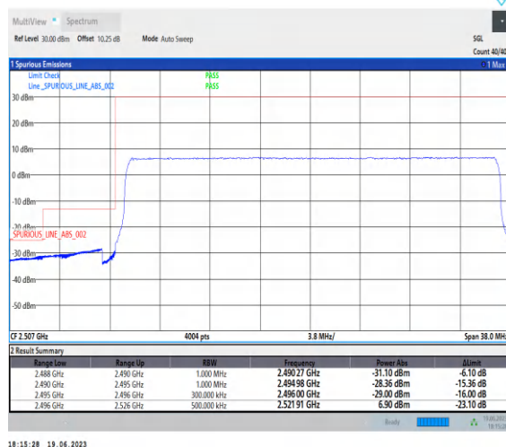
1-N41-PC2-30-30-L-3-CP-QPSK-Outer_Full-78@ 0-Ant0-1--PASS-see graph
