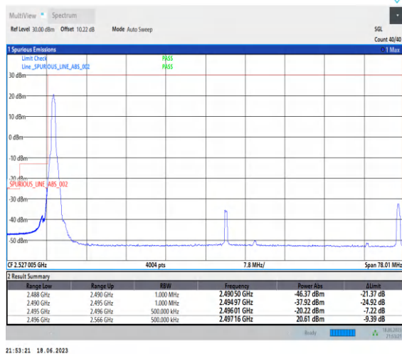
1-N41-PC3-30-70-L-4-CP-QPSK-Edge_1RB_Left-1@0-Ant0-1--PASS-see graph
