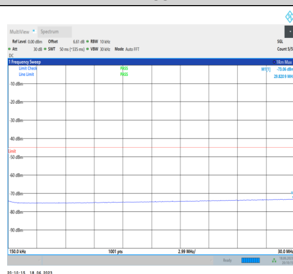
1-N41-PC3-30-100-L-1-N/A-DFT-PI2BPSK-Inner_1R B_Left-1@1-12000-27000-Ant0-22262.00--29.70--25 PASS
