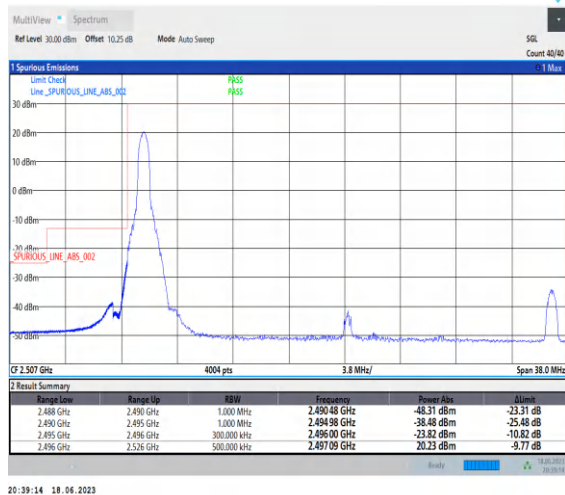
1-N41-PC3-30-30-L-4-CP-QPSK-Edge_1RB_Left-1@0-Ant0-1--PASS-see graph
