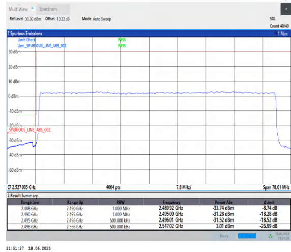
1-N41-PC3-30-70-L-3-DFT-PI2BPSK-Outer_Full-180@0-Ant0-1--PASS-see graph
