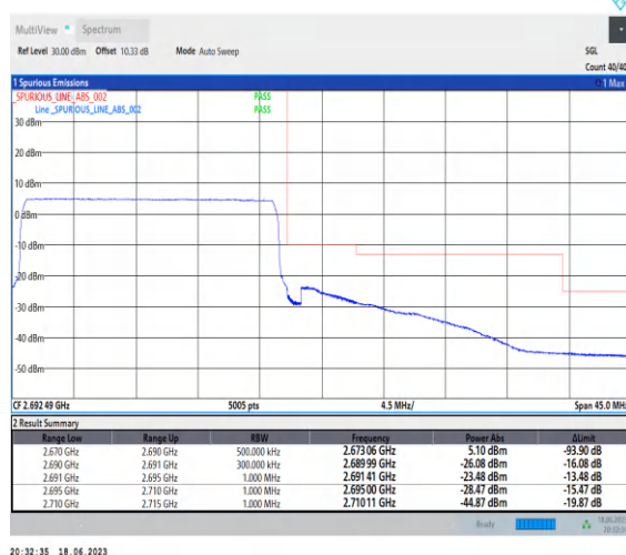
1-N41-PC3-30-20-H-6-CP-QPSK-Outer_Full-51@0-Ant0-1--PASS-see graph
