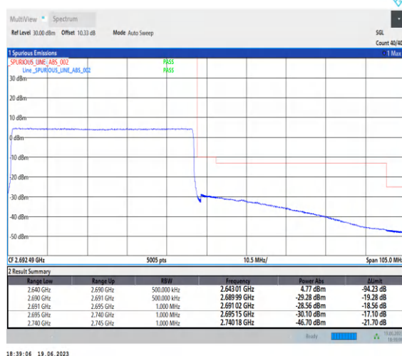
1-N41-PC2-30-50-H-3-CP-QPSK-Outer_Full-133@0-Ant0-1--PASS-see graph
