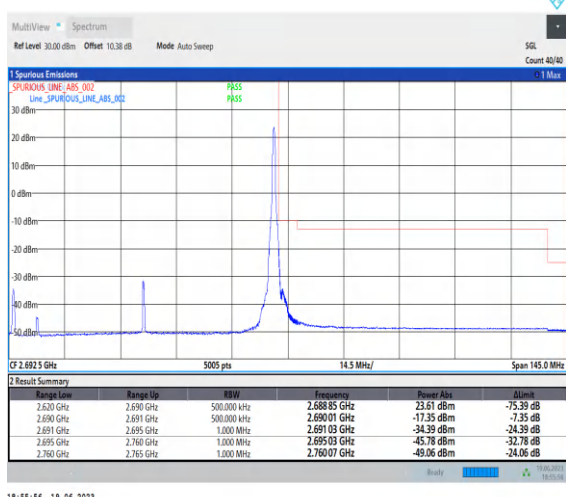
1-N41-PC2-30-70-H-2-CP-QPSK-Edge_1RB_Right-1@188-Ant0-1--PASS-see graph
