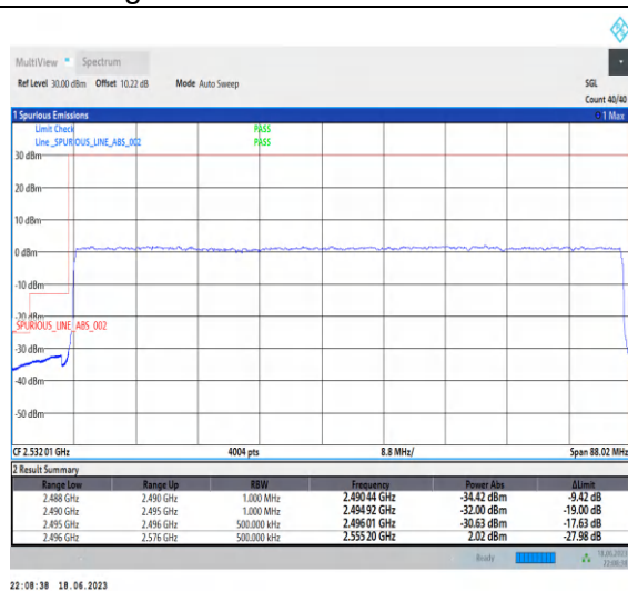
1-N41-PC3-30-80-L-3-DFT-PI2BPSK-Outer_Full-216@0-Ant0-1--PASS-see graph
