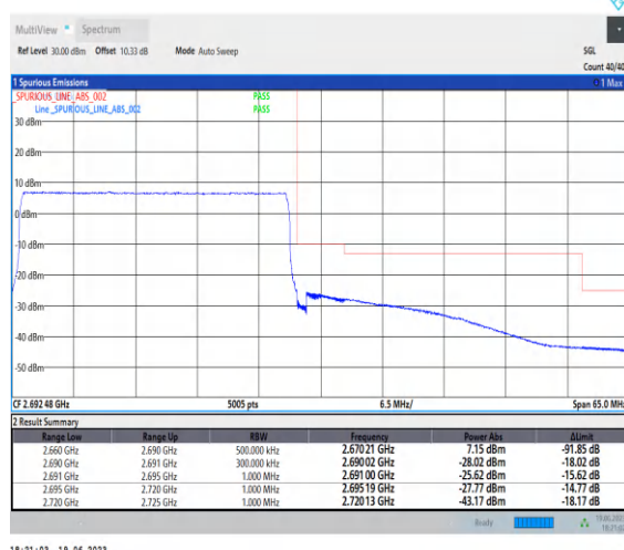
1-N41-PC2-30-30-H-3-CP-QPSK-Outer_Full-78@ 0-Ant0-1--PASS-see graph
