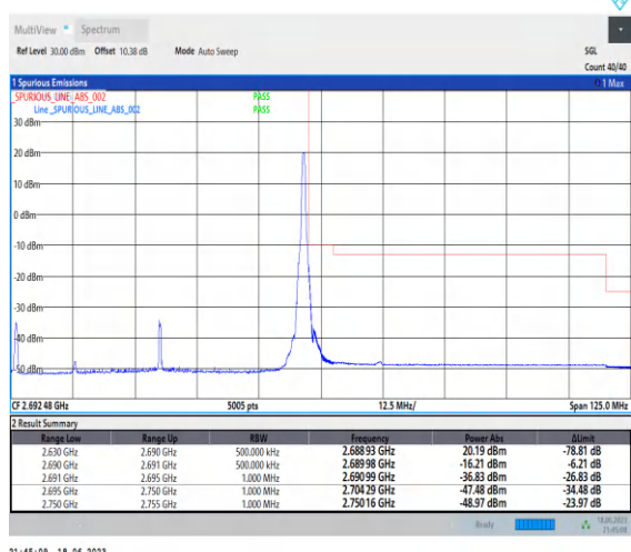
1-N41-PC3-30-60-H-5-CP-QPSK-Edge_1RB_Right-1 @161-Ant0-1--PASS-see graph
