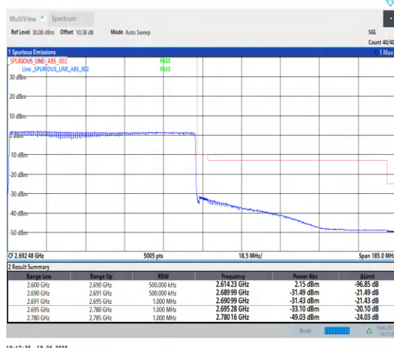
1-N41-PC2-30-90-H-3-CP-QPSK-Outer_Full-245 @0-Ant0-1--PASS-see graph
