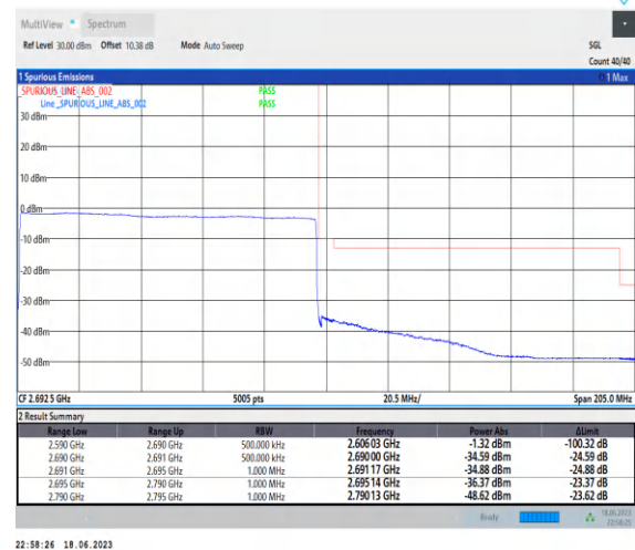
1-N41-PC3-30-100-H-6-CP-QPSK-Outer_Full-273 @0-Ant0-1--PASS-see graph
