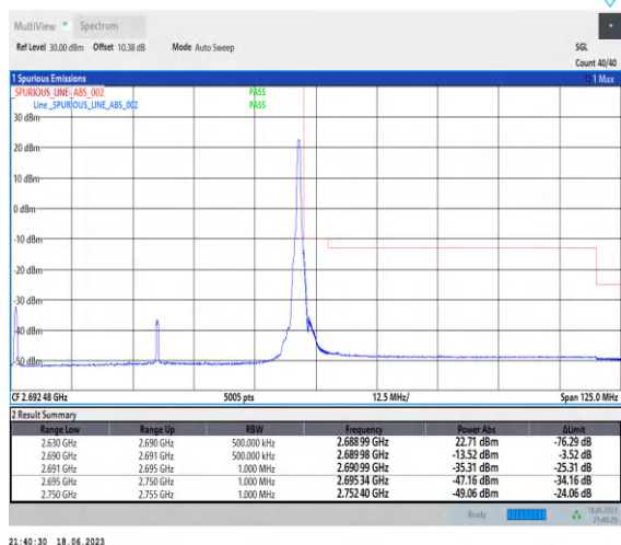
1-N41-PC3-30-60-H-2-DFT-PI2BPSK-Edge_1RB_Righ t-1@161-Ant0-1--PASS-see graph
