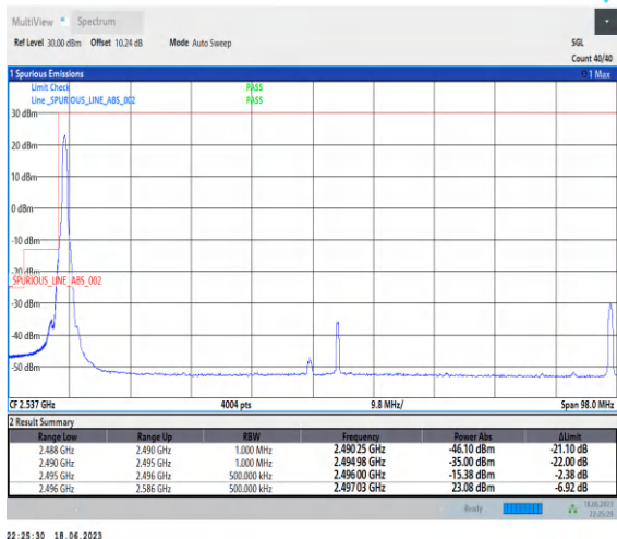
1-N41-PC3-30-90-L-1-DFT-PI2BPSK-Edge_1RB_Left-1@0-Ant0-1--PASS-see graph
