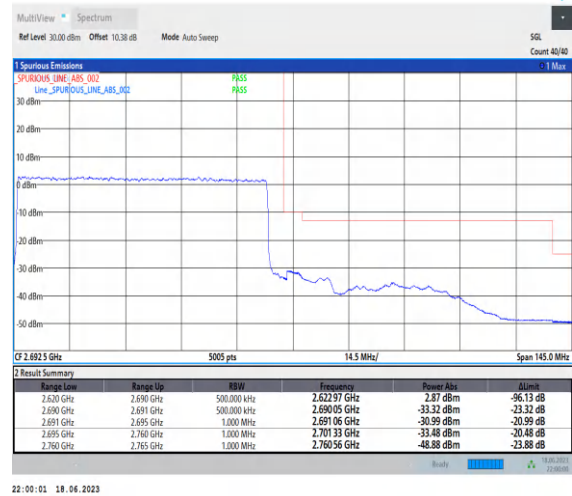
1-N41-PC3-30-70-H-3-DFT-PI2BPSK-Outer_Full-1 80@0-Ant0-1--PASS-see graph
