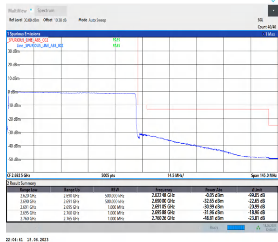
1-N41-PC3-30-70-H-6-CP-QPSK-Outer_Full-189 @0-Ant0-1--PASS-see graph
