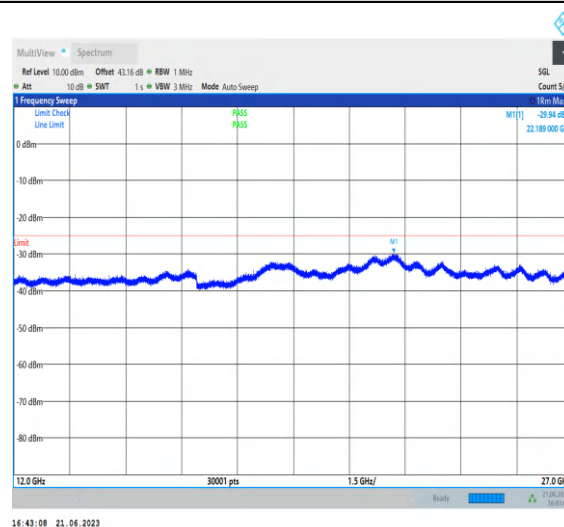
1-N41-PC3-30-100-M-1-N/A-DFT-PI2BPSK-Inner_1R B_Left-1@1-12000-27000-Ant0-22192.00--29.94--25- PASS
