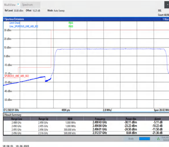
1-N41-PC2-30-20-L-3-CP-QPSK-Outer_Full-51@ 0-Ant0-1--PASS-see graph
