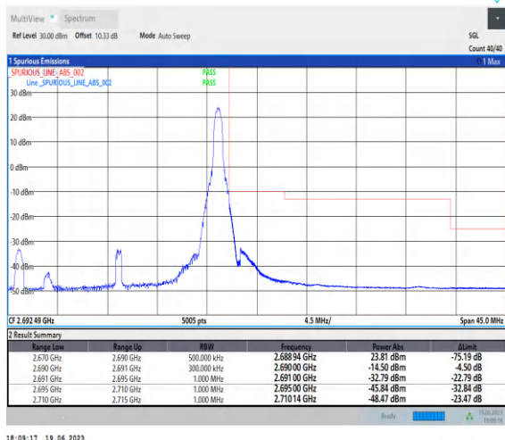
1-N41-PC2-30-20-H-2-CP-QPSK-Edge_1RB_Right-1 @50-Ant0-1--PASS-see graph
