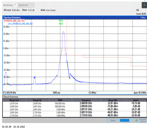
1-N41-PC3-30-20-H-2-DFT-PI2BPSK-Edge_1RB_Righ-t-1@50-Ant0-1--PASS-see graph
