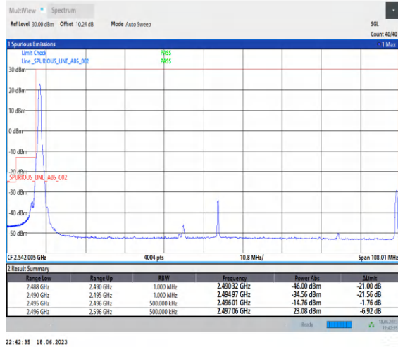
1-N41-PC3-30-100-L-1-DFT-PI2BPSK-Edge_1RB_Left-1@0-Ant0-1--PASS-see graph
