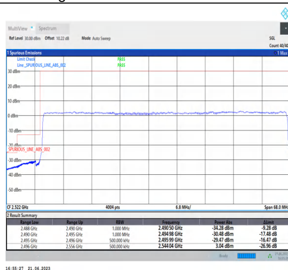
1-N41-PC3-30-60-L-3-DFT-PI2BPSK-Outer_Full-1 62@0-Ant0-1--PASS-see graph
