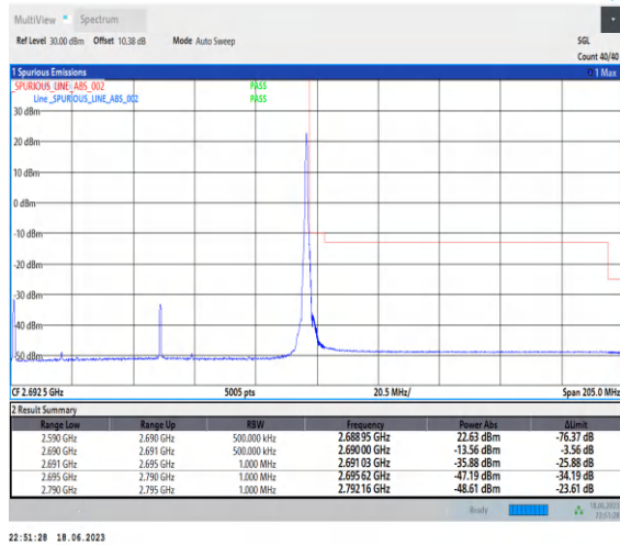
1-N41-PC3-30-100-H-2-DFT-PI2BPSK-Edge_1RB_Rig ht-1@272-Ant0-1--PASS-see graph
