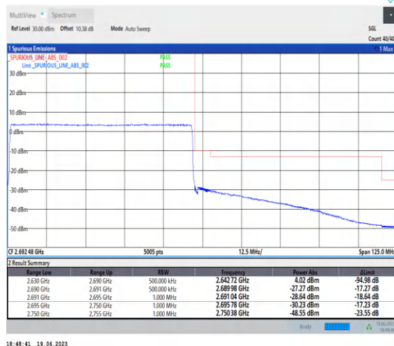
1-N41-PC2-30-60-H-3-CP-QPSK-Outer_Full-162 @0-Ant0-1--PASS-see graph
