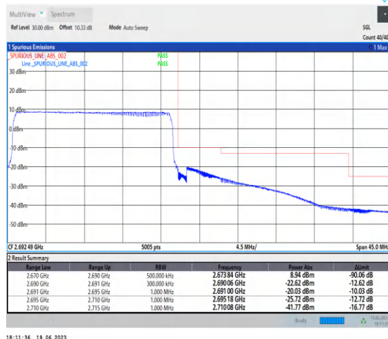
1-N41-PC2-30-20-H-3-CP-QPSK-Outer_Full-51@ 0-Ant0-1--PASS-see graph
