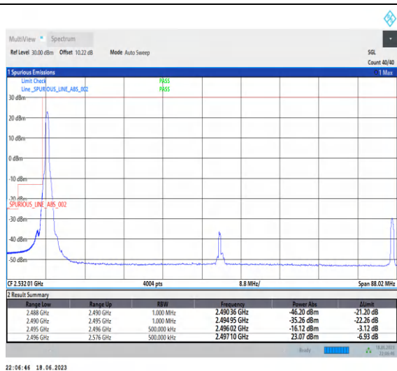
1-N41-PC3-30-80-L-1-DFT-PI2BPSK-Edge_1RB_Left-1@0-Ant0-1--PASS-see graph
