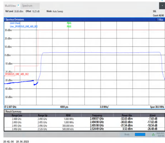
1-N41-PC3-30-30-L-6-CP-QPSK-Outer_Full-78@0-Ant0-1--PASS-see graph
