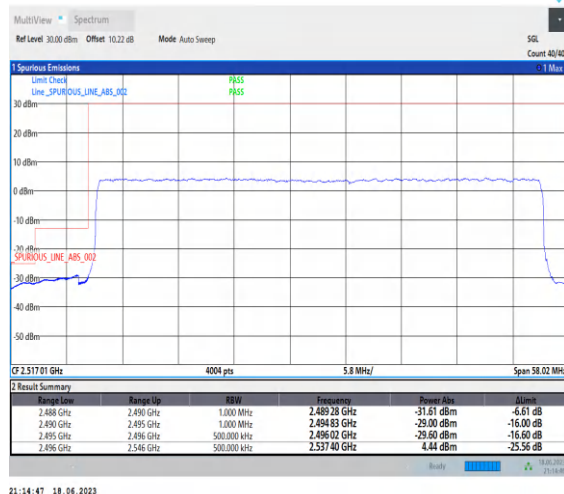
1-N41-PC3-30-50-L-3-DFT-PI2BPSK-Outer_Full-128@0-Ant0-1--PASS-see graph
