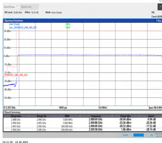
1-N41-PC2-30-90-L-3-CP-QPSK-Outer_Full-245 @0-Ant0-1--PASS-see graph
