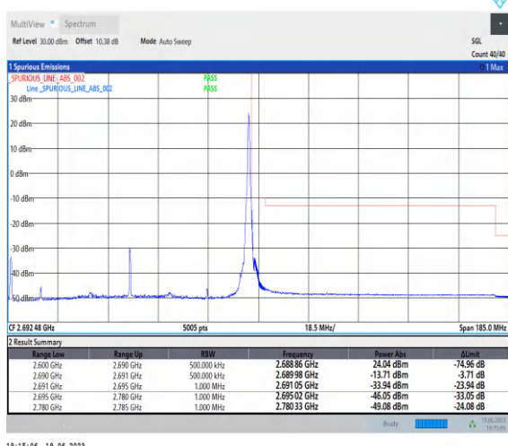
1-N41-PC2-30-90-H-2-CP-QPSK-Edge_1RB_Right-1 @244-Ant0-1--PASS-see graph
