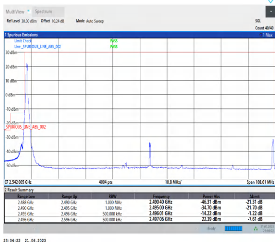
1-N41-PC2-30-100-L-1-CP-QPSK-Edge_1RB_Left-1@ 0-Ant0-1--PASS-see graph
