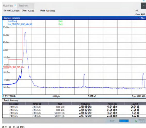
1-N41-PC2-30-50-L-1-CP-QPSK-Edge_1RB_Left-1@0-Ant0-1--PASS-see graph
