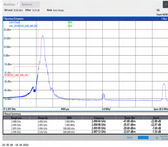
1-N41-PC3-30-30-L-1-DFT-PI2BPSK-Edge_1RB_Left-1@0-Ant0-1--PASS-see graph
