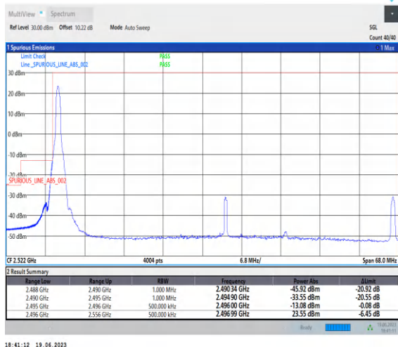
1-N41-PC2-30-60-L-1-CP-QPSK-Edge_1RB_Left-1@0 -Ant0-1--PASS-see graph
