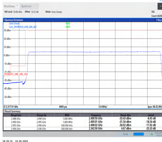
1-N41-PC2-30-50-L-3-CP-QPSK-Outer_Full-133@0-Ant0-1--PASS-see graph
