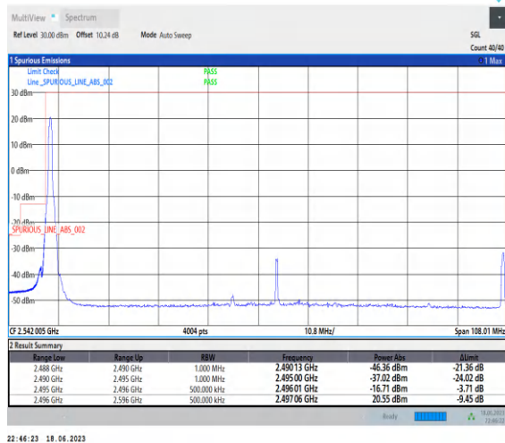
1-N41-PC3-30-100-L-4-CP-QPSK-Edge_1RB_Left-1@0-Ant0-1--PASS-see graph
