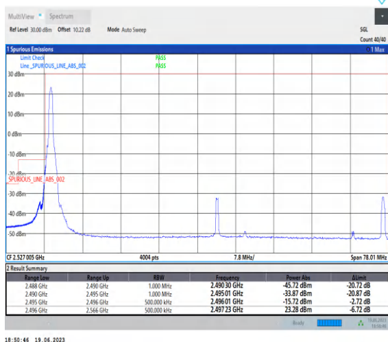
1-N41-PC2-30-70-L-1-CP-QPSK-Edge_1RB_Left-1@0-Ant0-1--PASS-see graph
