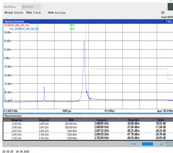
1-N41-PC3-30-70-H-5-CP-QPSK-Edge_1RB_Right-1 @188-Ant0-1--PASS-see graph
