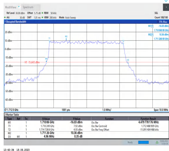
1-N66-PC3-15-5-L-4-DFT-64QAM-Outet_Full-25@0-Ant3-4.48-4.960-≤5-PASS
