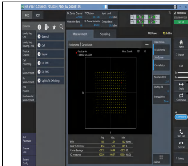
1-N66-PC3-15-40-M-5-DFT-256QAM-Outer_Full-216 @0-Ant3-see graph-PASS
