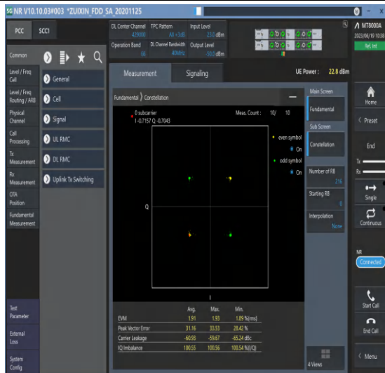
1-N66-PC3-15-40-M-1-DFT-PI2BPSK-Outter_Full-216 @0-Ant3-see graph-PASS
