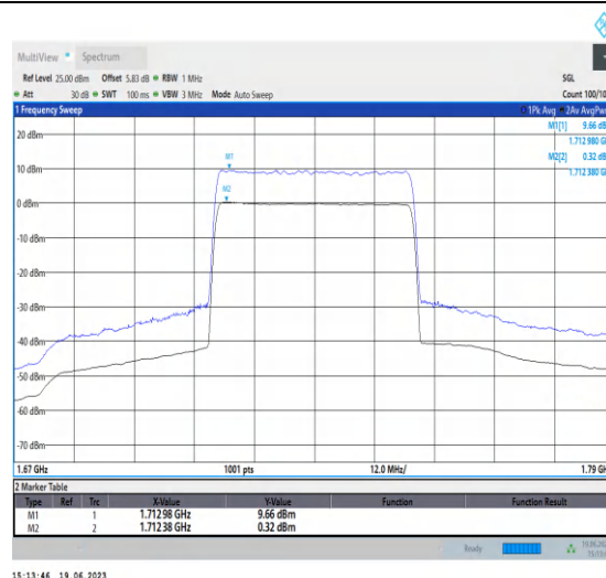
1-N66-PC3-15-40-L-2-CP-256QAM-Outer_Full-216 @0-Ant3-9.34-100%-0.00-9.34-PASS≤13
