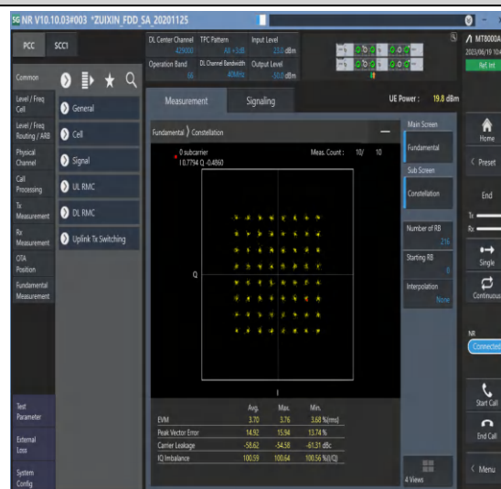
1-N66-PC3-15-40-M-8-CP-64QAM-Outer_Full-216 @0-Ant3-see graph-PASS
