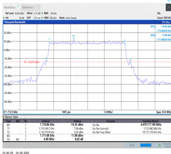
1-N66-PC3-15-5-L-3-DFT-16QAM-Outet_Full-25@0-Ant3-4.479-4.990-≤5-PASS
