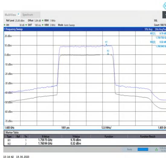
1-N66-PC3-15-40-M-2-CP-256QAM-Outer_Full-216 @0-Ant3-9.38-100%-0.00-9.38-PASS≤13
