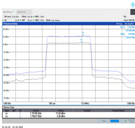
1-N66-PC3-15-40-M-1-DFT-256QAM-Outer_Full-216 @0-Ant3-9.14-100%-0.00-9.14-PASS≤13
