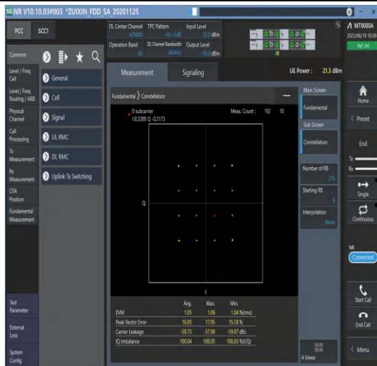
1-N66-PC3-15-40-M-3-DFT-16QAM-Outter_Full-216 @0-Ant3-see graph-PASS
