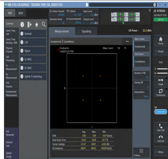
1-N66-PC3-15-40-M-2-DFT-QPSK-Outter_Full-216 @0-Ant3-see graph-PASS
