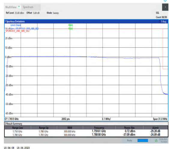
1-N66-PC3-15-30-H-6-CP-QPSK-Outer_Full-160 @0-Ant3-1-seegraph-PASS-see graph
