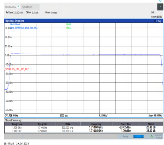
1-N66-PC3-15-40-L-6-CP-QPSK-Outer_Full-216@0-Ant3-1-seegraph-PASS-see graph
