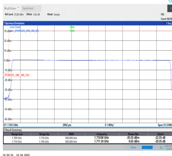
1-N66-PC3-15-30-L-6-CP-QPSK-Outer_Full-160@0-Ant3-1-seegraph-PASS-see graph
