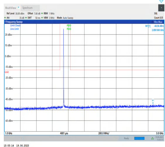
1-N66-PC3-15-40-H-1-DFT-PI2BPSK-Inner_1RB_L ef t-1@1-1000-3000-Ant3-2859.50--44.56--13-PASS
