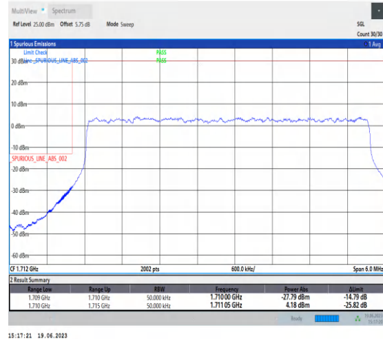
1-N66-PC3-15-5-L-3-DFT-PI2BPSK-Outer_Full-25 @0-Ant3-1-seegraph-PASS-see graph
