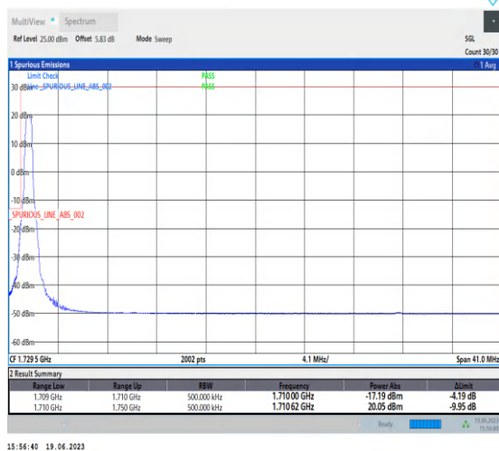
1-N66-PC3-15-40-L-4-CP-QPSK-Edge_1RB_Left-1@0-Ant3-1-seegraph-PASS-see graph
