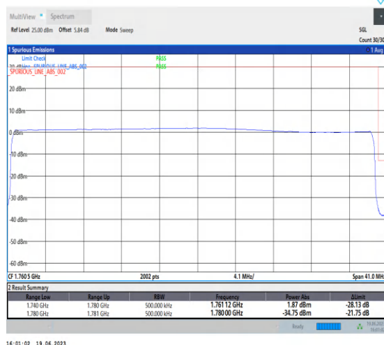
1-N66-PC3-15-40-H-6-CP-QPSK-Outer_Full-216@0-Ant3-1-seegraph-PASS-see graph
