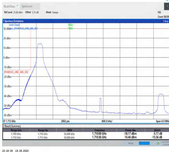
1-N66-PC3-15-5-L-4-CP-QPSK-Edge_1RB_Left-1@0-Ant3-1-seegraph-PASS-see graph
