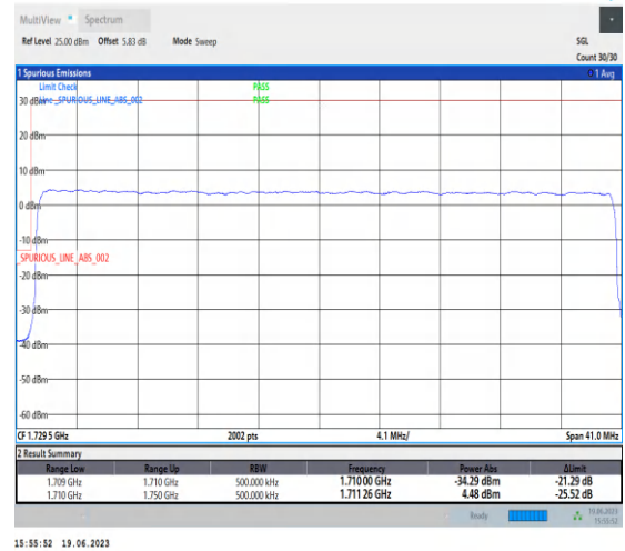
1-N66-PC3-15-40-L-3-DFT-PI2BPSK-Outer_Full-216@0-Ant3-1-seegraph-PASS-see graph
