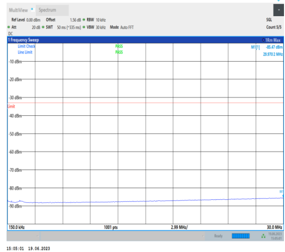
1-N66-PC3-15-40-H-1-DFT-PI2BPSK-Inner_1RB_L ef t-1@1-0.15-30-Ant3-29.97--85.47--33-PASS
