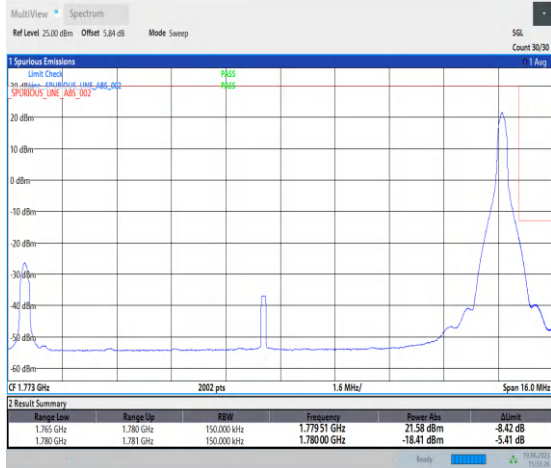
1-N66-PC3-15-15-H-2-DFT-PI2BPSK-Edge_1RB_Righ t-1@78-Ant3-1-seegraph-PASS-see graph
