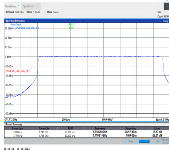
1-N66-PC3-15-5-L-6-CP-QPSK-Outer_Full-25@0-Ant3-1-seegraph-PASS-see graph
