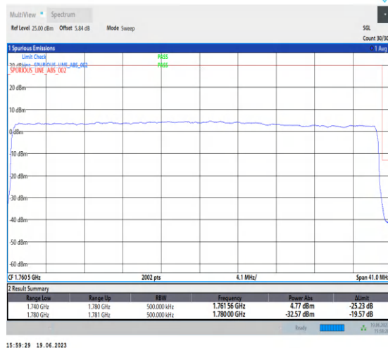
1-N66-PC3-15-40-H-3-DFT-PI2BPSK-Outer_Full-216@0-Ant3-1-seegraph-PASS-see graph
