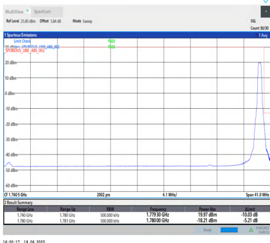
1-N66-PC3-15-40-H-5-CP-QPSK-Edge_1RB_Right-1@215-Ant3-1-seegraph-PASS-see graph
