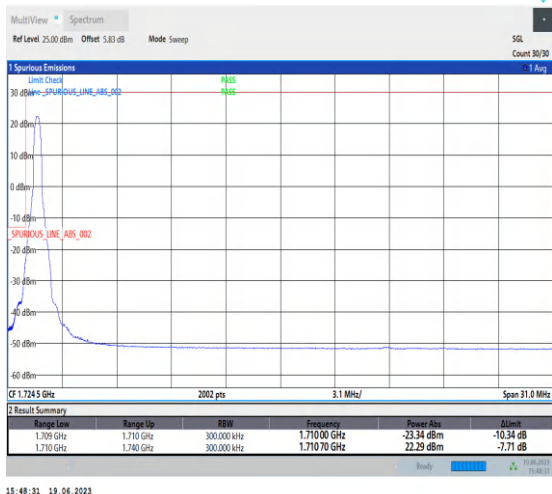
1-N66-PC3-15-30-L-1-DFT-PI2BPSK-Edge_1RB_Left-1@0-Ant3-1-seegraph-PASS-see graph
