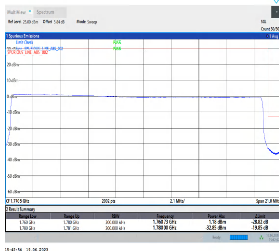
1-N66-PC3-15-20-H-6-CP-QPSK-Outer_Full-106 @0-Ant3-1-seegraph-PASS-see graph
