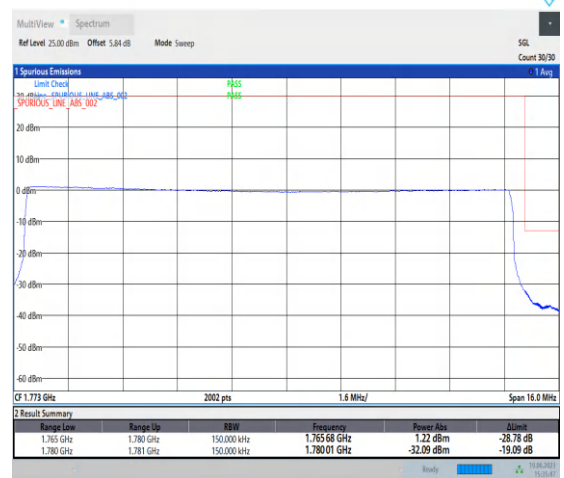
1-N66-PC3-15-15-H-6-CP-QPSK-Outer_Full-79@0 -Ant3-1-seegraph-PASS-see graph
