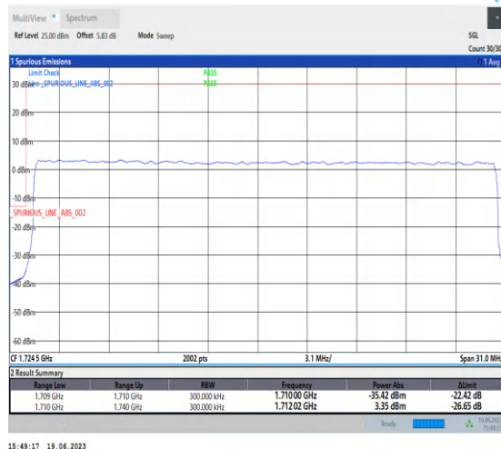
1-N66-PC3-15-30-L-3-DFT-PI2BPSK-Outer_Full-160@0-Ant3-1-seegraph-PASS-see graph
