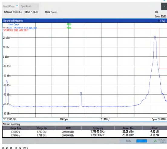
1-N66-PC3-15-20-H-2-DFT-PI2BPSK-Edge_1RB_Righ t-1@105-Ant3-1-seegraph-PASS-see graph
