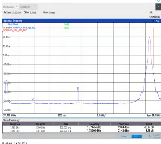
1-N66-PC3-15-20-H-5-CP-QPSK-Edge_1RB_Right-1 @105-Ant3-1-seegraph-PASS-see graph
