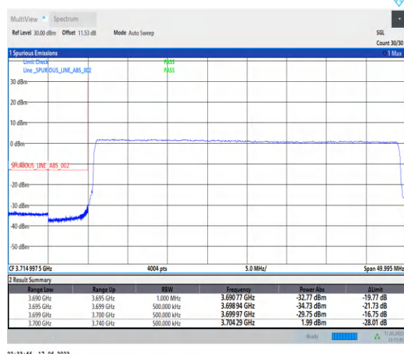
1-N77-3700-3980-PC3-30-40-L-6-CP-QPSK-Outer_Full-106@0-Ant2-1--PASS-see graph
