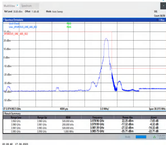
1-N77-3700-3980-PC3-30-20-H-2-DFT-PI2BPSK-Edge_1RB_Right-1@50-Ant2-1--PASS-see graph
