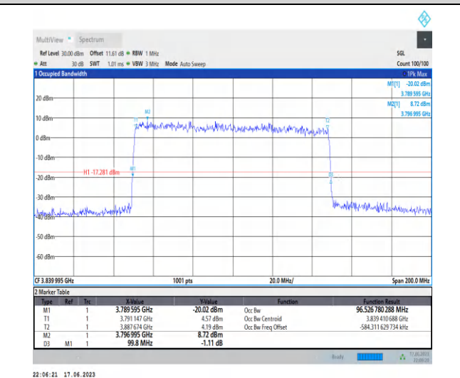
1-N77-3700-3980-PC3-30-100-M-5-DFT-256QAM-Out er_Full-270@0-Ant2-96.527-99.800-≤100-PASS
