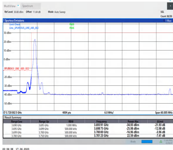
1-N77-3700-3980-PC3-30-50-L-1-DFT-PI2BPSK-Edge_1RB_Left-1@0-Ant2-1--PASS-see graph
