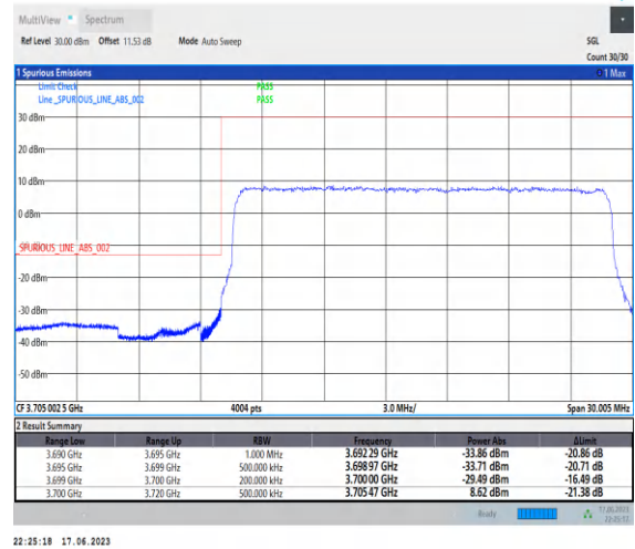
1-N77-3700-3980-PC3-30-20-L-3-DFT-PI2BPSK-Outer_Full-50@0-Ant2-1--PASS-see graph
