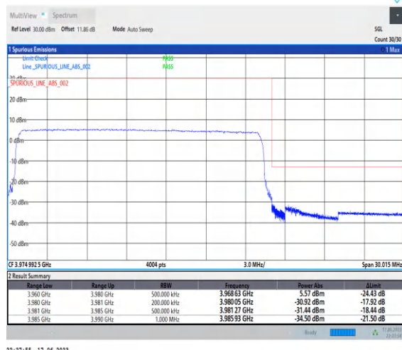
1-N77-3700-3980-PC3-30-20-H-6-CP-QPSK-Outer_Full-51@0-Ant2-1--PASS-see graph
