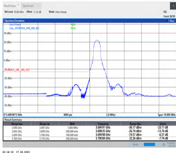
1-N77-3700-3980-PC3-30-10-L-1-DFT-PI2BPSK-Edge_1RB_Left-1@0-Ant2-1--PASS-see graph
