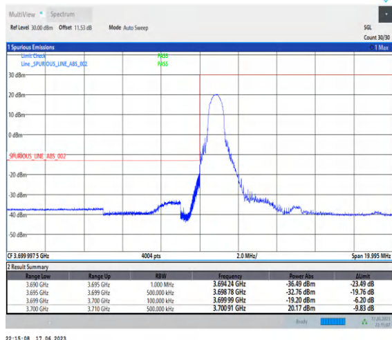
1-N77-3700-3980-PC3-30-10-L-4-CP-QPSK-Edge_1RB_Left-1@0-Ant2-1--PASS-see graph
