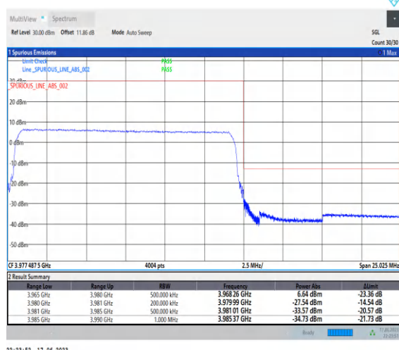
1-N77-3700-3980-PC3-30-15-H-6-CP-QPSK-Outer_Full-38@0-Ant2-1--PASS-see graph
