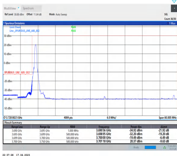
1-N77-3700-3980-PC3-30-50-L-4-CP-QPSK-Edge_1RB_Left-1@0-Ant2-1--PASS-see graph
