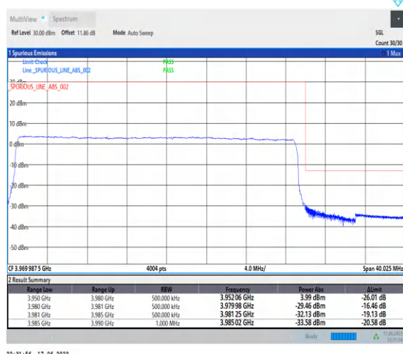
1-N77-3700-3980-PC3-30-30-H-6-CP-QPSK-Outer_Full-78@0-Ant2-1-PASS-see graph
