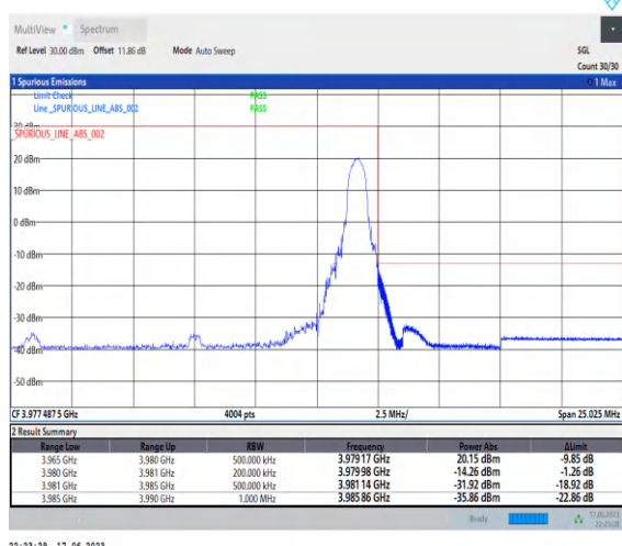
1-N77-3700-3980-PC3-30-15-H-5-CP-QPSK-Edge_1RB_Right-1@37-Ant2-1--PASS-see graph
