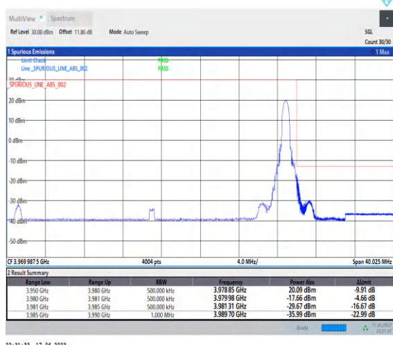
1-N77-3700-3980-PC3-30-30-H-5-CP-QPSK-Edge_1RB_Right-1@77-Ant2-1-PASS-see graph
