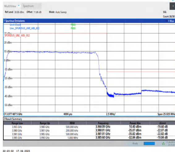
1-N77-3700-3980-PC3-30-15-H-3-DFT-PI2BPSK-Outer_Full-36@0-Ant2-1--PASS-see graph
