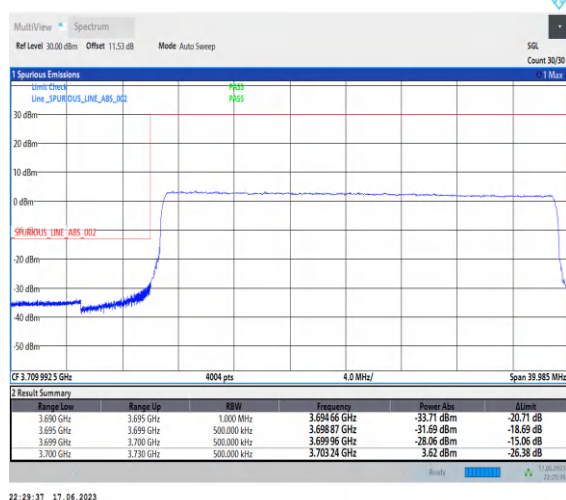
1-N77-3700-3980-PC3-30-30-L-6-CP-QPSK-Outer_Full-78@0-Ant2-1--PASS-see graph
