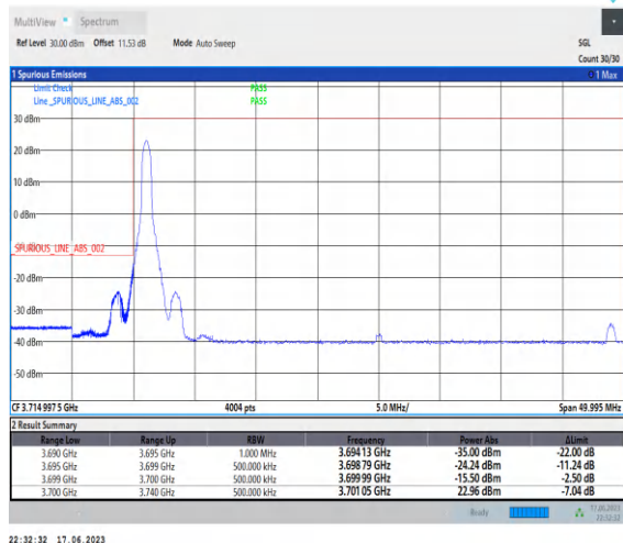
1-N77-3700-3980-PC3-30-40-L-1-DFT-PI2BPSK-Edge_1RB_Left-1@0-Ant2-1--PASS-see graph
