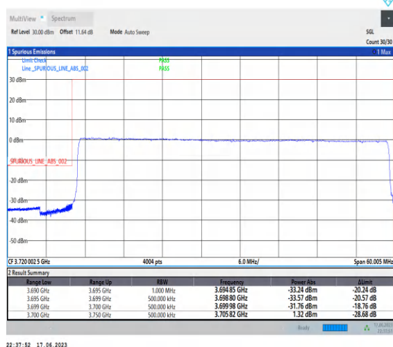
1-N77-3700-3980-PC3-30-50-L-6-CP-QPSK-Outer_Full-133@0-Ant2-1--PASS-see graph
