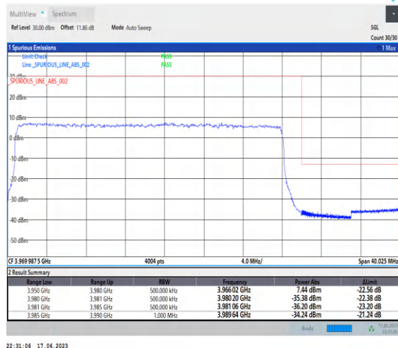
1-N77-3700-3980-PC3-30-30-H-3-DFT-PI2BPSK-Outer_Full-75@0-Ant2-1-PASS-see graph
