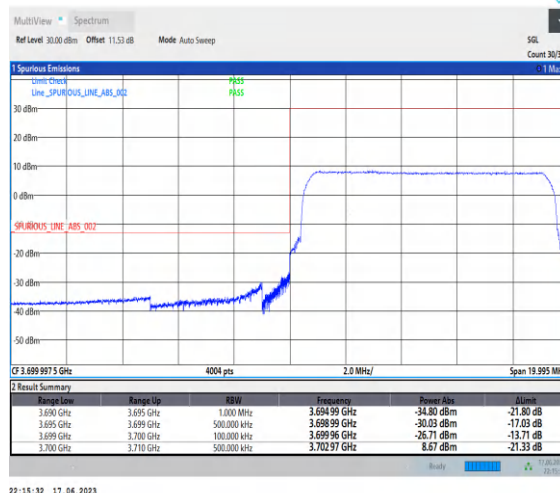
1-N77-3700-3980-PC3-30-10-L-6-CP-QPSK-Outer_Full-24@0-Ant2-1--PASS-see graph
