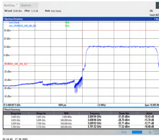
1-N77-3700-3980-PC3-30-10-L-3-DFT-PI2BPSK-Outer_Full-24@0-Ant2-1--PASS-see graph
