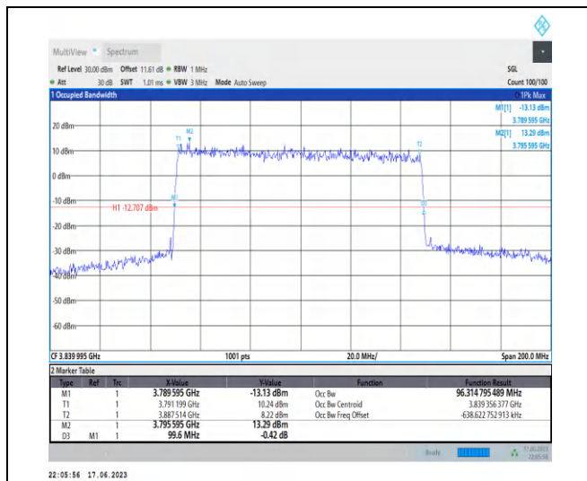
1-N77-3700-3980-PC3-30-100-M-2-DFT-QPSK-Out er_Full-270@0-Ant2-96.315-99.600-≤100-PASS
