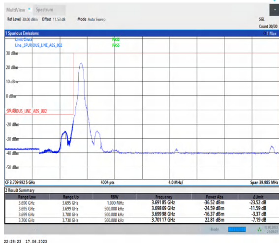
1-N77-3700-3980-PC3-30-30-L-1-DFT-PI2BPSK-Edge_1RB_Left-1@0-Ant2-1--PASS-see graph
