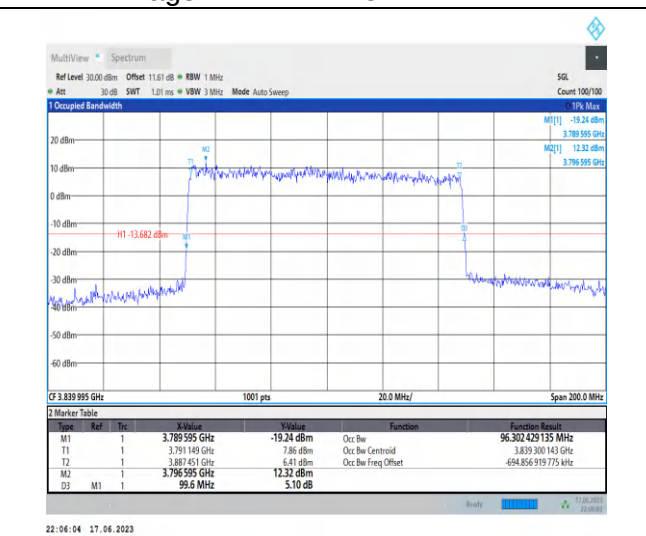
1-N77-3700-3980-PC3-30-100-M-3-DFT-16QAM-Out er_Full-270@0-Ant2-96.302-99.600-≤100-PASS
