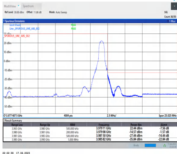
1-N77-3700-3980-PC3-30-15-H-2-DFT-PI2BPSK-Edge_1RB_Right-1@37-Ant2-1--PASS-see graph
