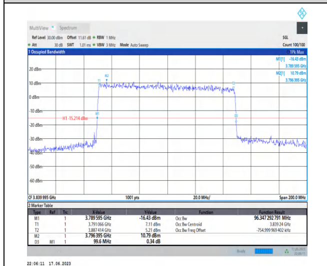
1-N77-3700-3980-PC3-30-100-M-4-DFT-64QAM-Out er_Full-270@0-Ant2-96.347-99.600-≤100-PASS
