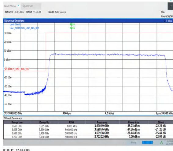
1-N77-3700-3980-PC3-30-30-L-3-DFT-PI2BPSK-Outer_Full-75@0-Ant2-1--PASS-see graph
