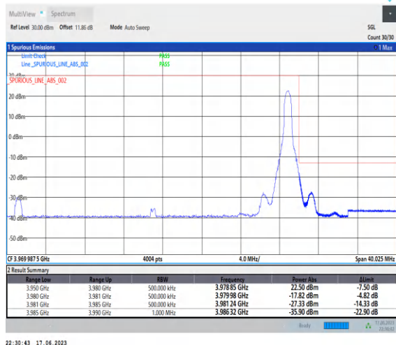
1-N77-3700-3980-PC3-30-30-H-2-DFT-PI2BPSK-Edge_1RB_Right-1@77-Ant2-1-PASS-see graph
