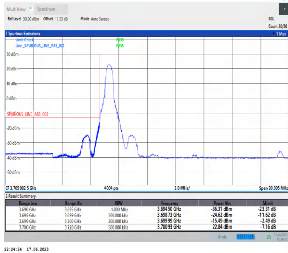
1-N77-3700-3980-PC3-30-20-L-1-DFT-PI2BPSK-Edge_1RB_Left-1@0-Ant2-1--PASS-see graph
