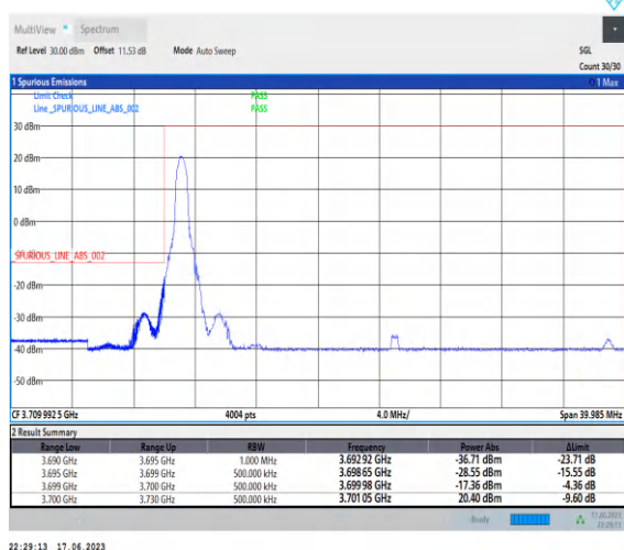
1-N77-3700-3980-PC3-30-30-L-4-CP-QPSK-Edge_1RB_Left-1@0-Ant2-1--PASS-see graph
