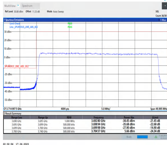
1-N77-3700-3980-PC3-30-40-L-3-DFT-PI2BPSK-Outer_Full-100@0-Ant2-1--PASS-see graph
