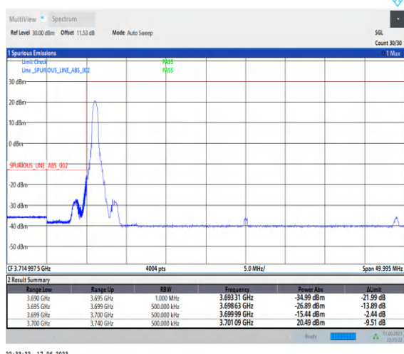
1-N77-3700-3980-PC3-30-40-L-4-CP-QPSK-Edge_1RB_Left-1@0-Ant2-1--PASS-see graph
