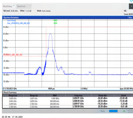
1-N77-3700-3980-PC3-30-20-L-4-CP-QPSK-Edge_1RB_Left-1@0-Ant2-1--PASS-see graph
