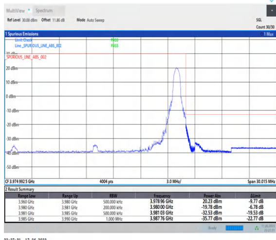
1-N77-3700-3980-PC3-30-20-H-5-CP-QPSK-Edge_1RB_Right-1@50-Ant2-1--PASS-see graph
