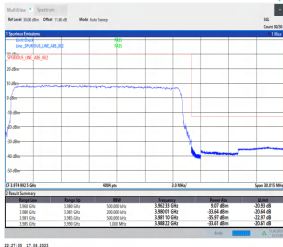
1-N77-3700-3980-PC3-30-20-H-3-DFT-PI2BPSK-Outer_Full-50@0-Ant2-1--PASS-see graph
