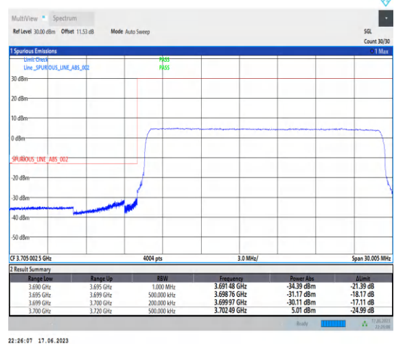
1-N77-3700-3980-PC3-30-20-L-6-CP-QPSK-Outer_Full-51@0-Ant2-1--PASS-see graph
