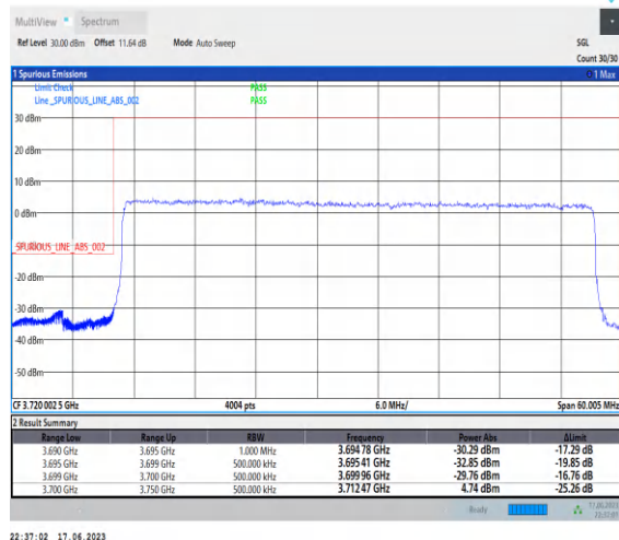
1-N77-3700-3980-PC3-30-50-L-3-DFT-PI2BPSK-Outer_Full-128@0-Ant2-1--PASS-see graph
