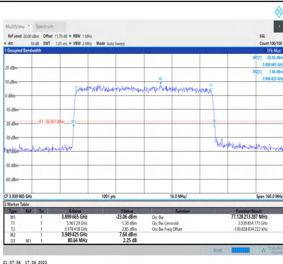
1-N77-3700-3980-PC3-30-80-H-9-CP-256QAM-Outer_Full-217@0-Ant2-77.128-80.640-≤80-PASS
