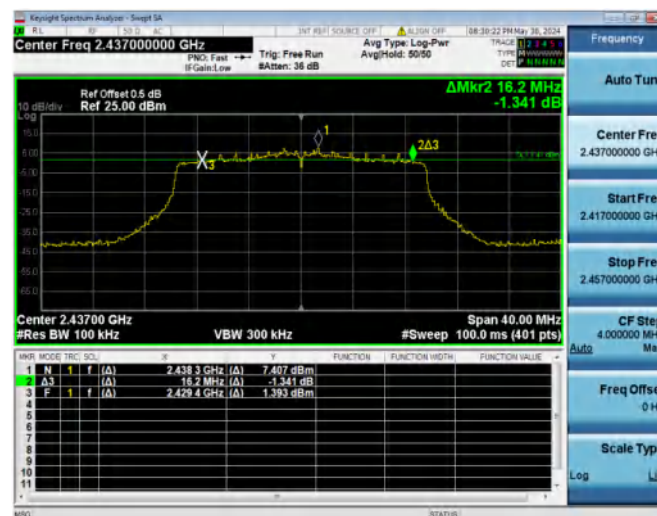
802.11ax-20 MHz(SU) MIDDLE CHANNEL
