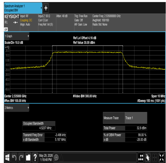
Band7-5MHz-64QAM-20775-25RB#0-PASS
