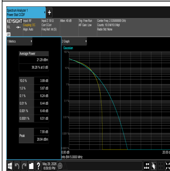
Band7-5MHz-64QAM-21100-1RB#0-PASS
