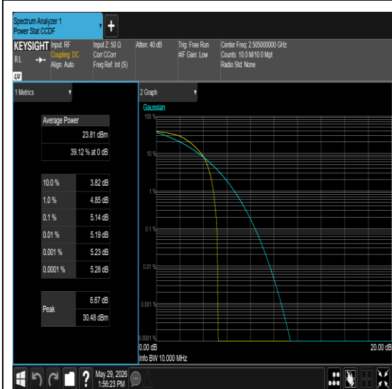
Band7-10MHz-QPSK-20800-1RB#0-PASS
