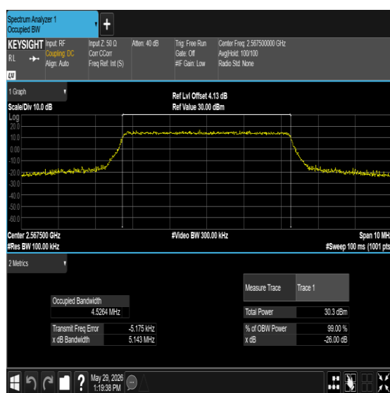
Band7-5MHz-16QAM-21425-25RB#0-PASS
