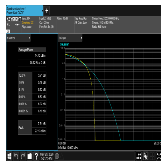
Band7-15MHz-QPSK-21100-1RB#0-PASS
