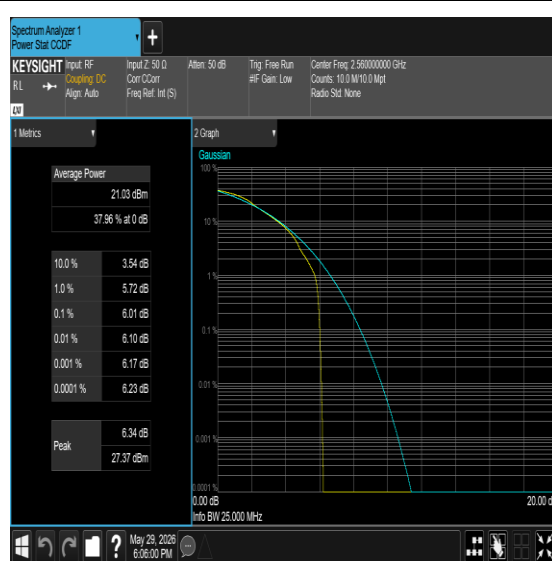
Band7-20MHz-QPSK-21350-1RB#0-PASS
