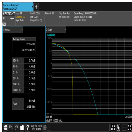
Band7-10MHz-QPSK-21400-1RB#0-PASS
