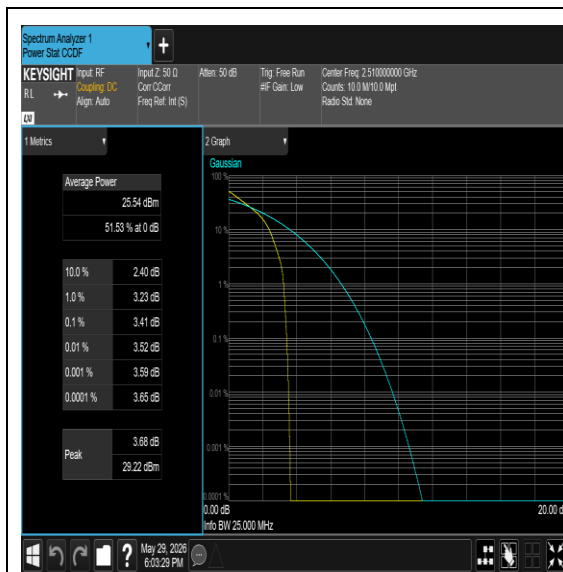
Band7-20MHz-QPSK-21100-1RB#0-PASS
