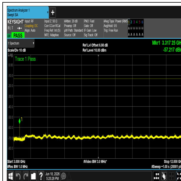
NTNV-n71-PC3-15-15-M-DFT-QPSK-Edge_1RB_Left- 30-1000-PASS
