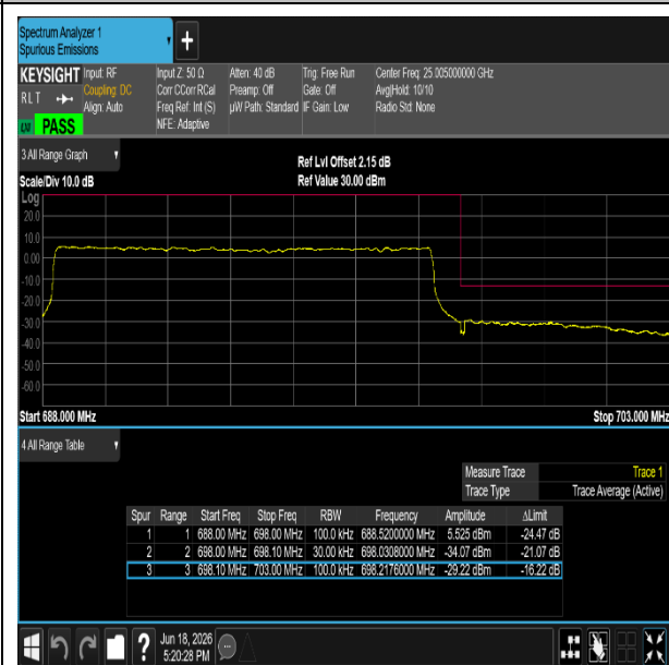
NTNV-n71-PC3-15-15-L-DFT-QPSK-Outer_Full-PASS
