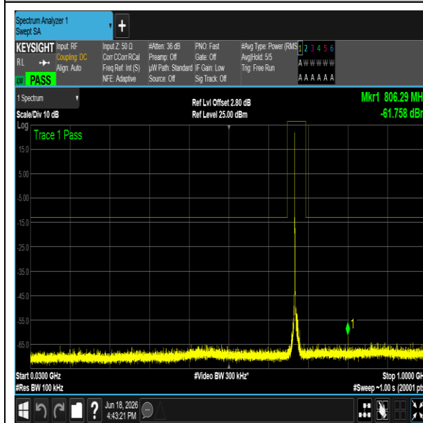
NTNV-n71-PC3-15-10-M-DFT-QPSK-Edge_1RB_Left- 3000-12000-PASS
