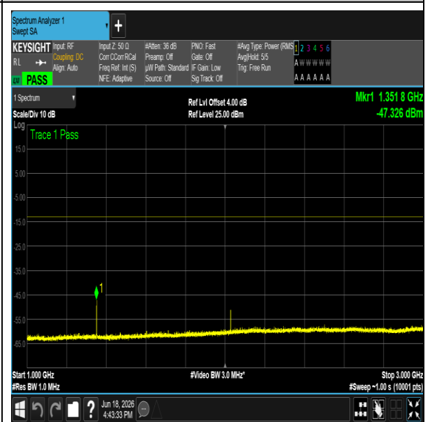
NTNV-n71-PC3-15-10-M-DFT-QPSK-Edge_1RB_Left- 12000-20000-PASS
