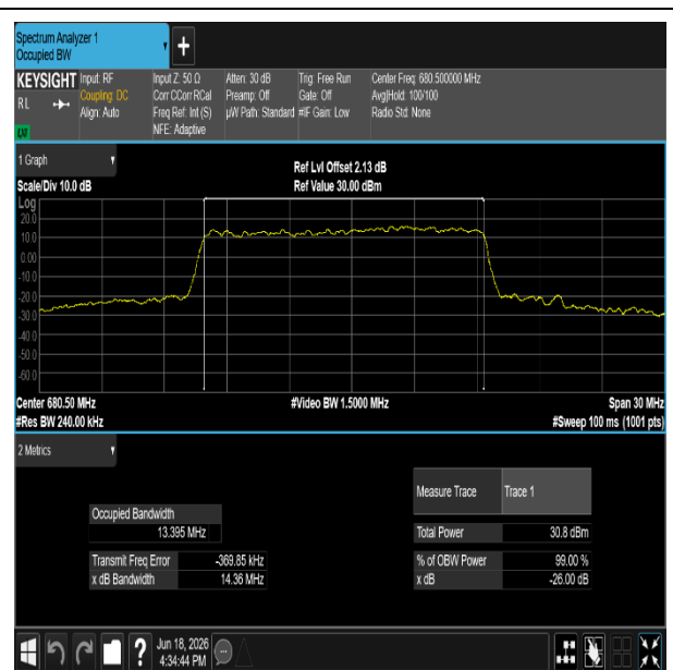
NTNV-n71-PC3-15-20-M-DFT-BPSK-Outer_Full-Ant1-PASS
