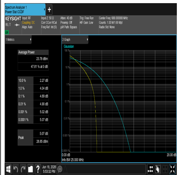
NTNV-n71-PC3-15-20-H-DFT-QPSK-Outer_Full-PASS
