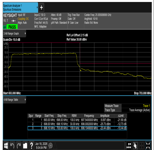
NTNV-n71-PC3-15-10-L-DFT-QPSK-Outer_Full-PASS
