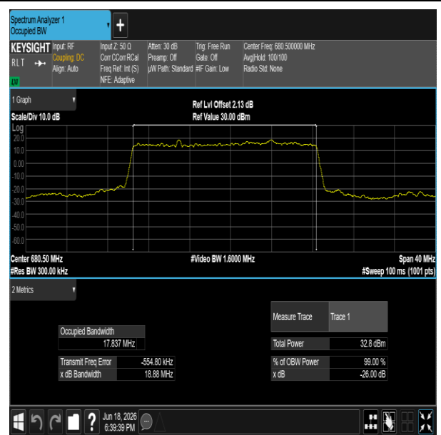
NTNV-n71-PC3-15-20-M-DFT-16QAM-Outer_Full-Ant1-PASS
