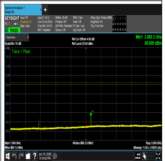
NTNV-n71-PC3-15-10-H-DFT-QPSK-Edge_1RB_Left- 12000-20000-PASS
