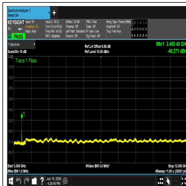
NTNV-n71-PC3-15-15-H-DFT-QPSK-Edge_1RB_Left- 30-1000-PASS
