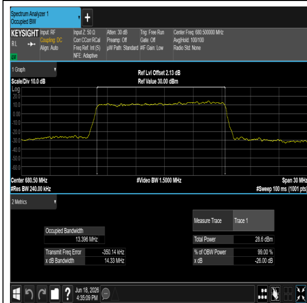
NTNV-n71-PC3-15-20-M-DFT-QPSK-Outer_Full-Ant1-PASS
