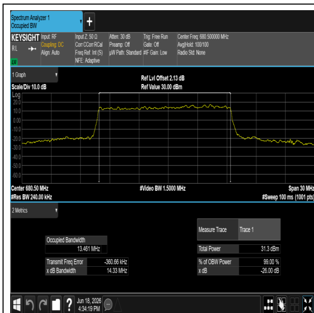
NTNV-n71-PC3-15-15-M-DFT-256QAM-Outer_Full-Ant1-PASS
