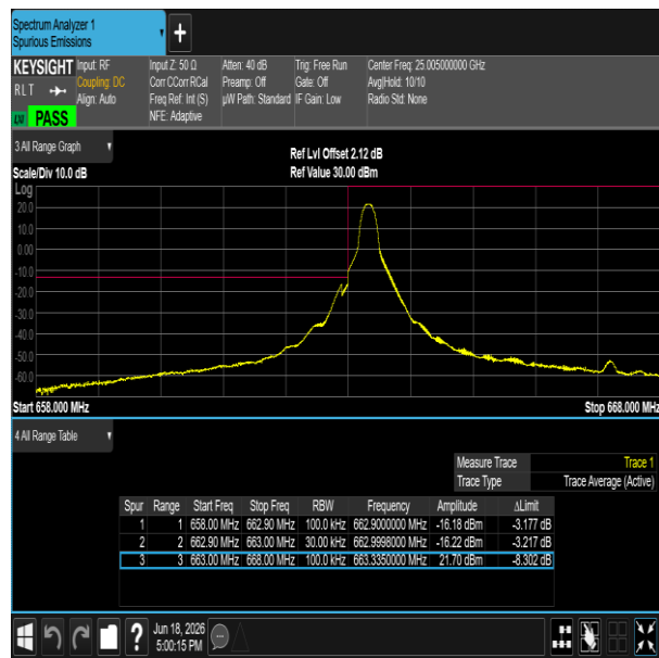
NTNV-n71-PC3-15-5-H-DFT-QPSK-Edge_1RB_Right-PASS
