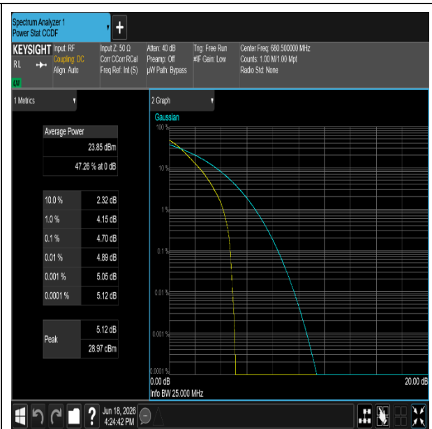
NTNV-n71-PC3-15-20-H-DFT-QPSK-Outer_Full-PASS
