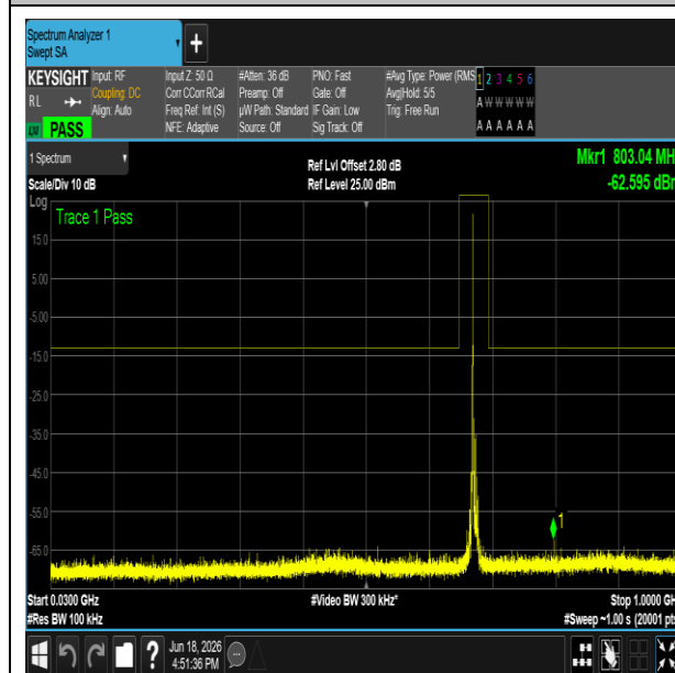
NTNV-n71-PC3-15-5-M-DFT-QPSK-Edge_1RB_Left- 3000-12000-PASS
