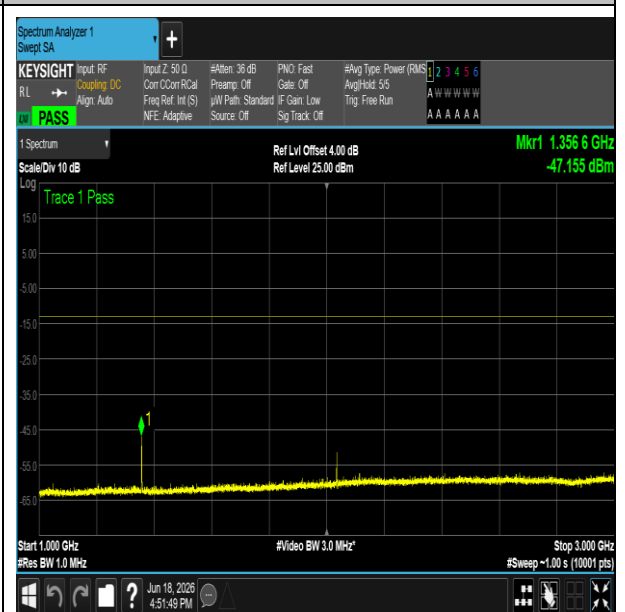
NTNV-n71-PC3-15-5-M-DFT-QPSK-Edge_1RB_Left- 12000-20000-PASS
