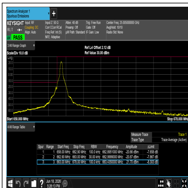
NTNV-n71-PC3-15-15-H-DFT-QPSK-Edge_1RB_Right-PASS
