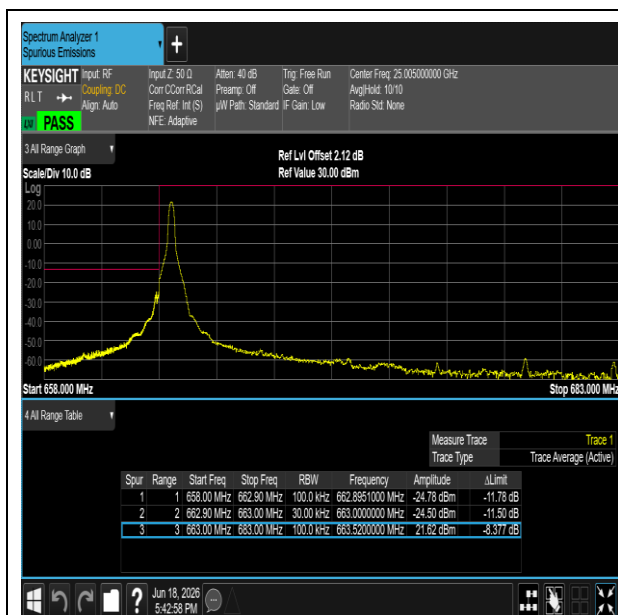
NTNV-n71-PC3-15-20-H-DFT-QPSK-Edge_1RB_Right-PASS
