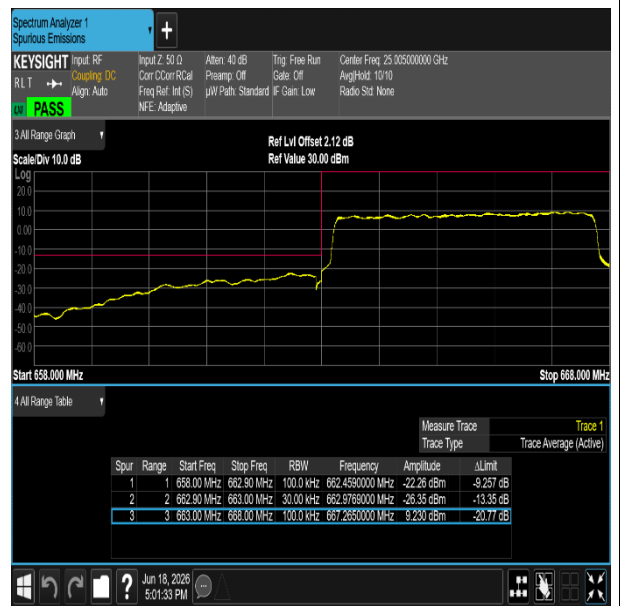
NTNV-n71-PC3-15-5-H-DFT-QPSK-Outer_Full-PASS
