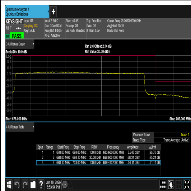
NTNV-n71-PC3-15-20-H-DFT-QPSK-Outer_Full-PASS
