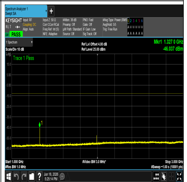
NTNV-n71-PC3-15-15-L-DFT-QPSK-Edge_1RB_Left- 12000-20000-PASS
