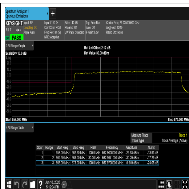
NTNV-n71-PC3-15-10-H-DFT-QPSK-Outer_Full-PASS
