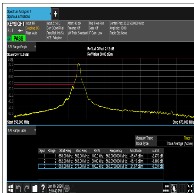
NTNV-n71-PC3-15-10-H-DFT-QPSK-Edge_1RB_Right-PASS
