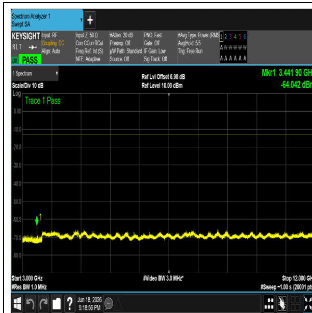
NTNV-n71-PC3-15-15-L-DFT-QPSK-Edge_1RB_Left- 30-1000-PASS
