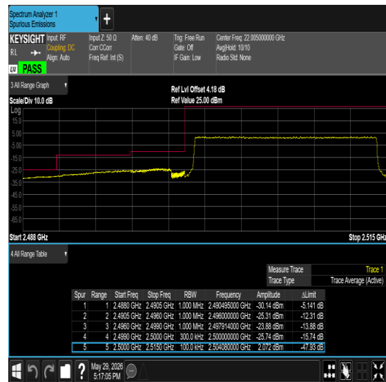
Band7-15MHz-16QAM-21375-75RB#0-PASS
