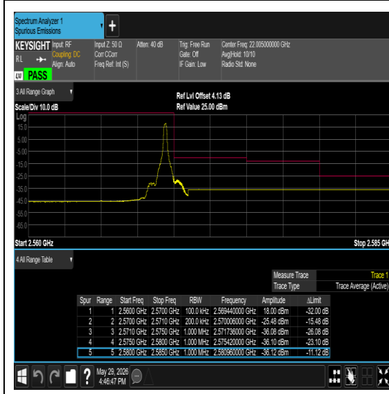
Band7-10MHz-64QAM-21400-1RB#49-PASS
