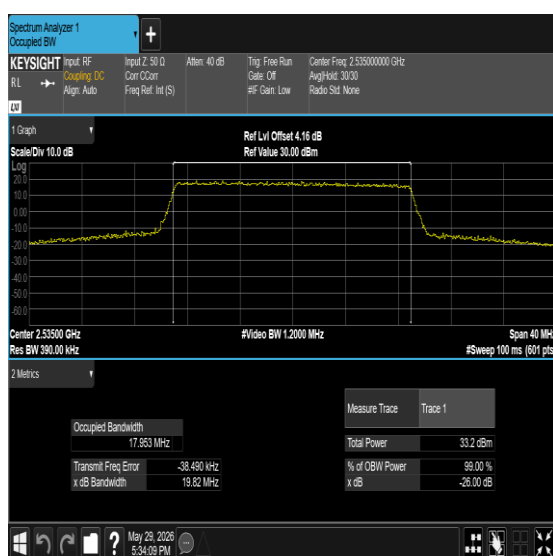
Band7-20MHz-QPSK-21100-100RB#0-PASS
