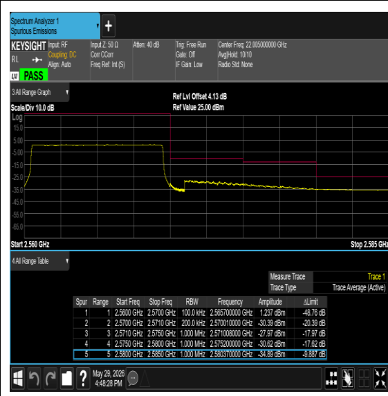
Band7-10MHz-64QAM-21400-50RB#0-PASS
