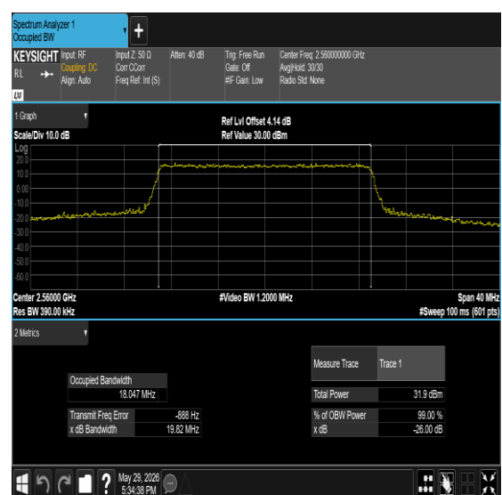
Band7-20MHz-QPSK-21350-100RB#0-PASS
