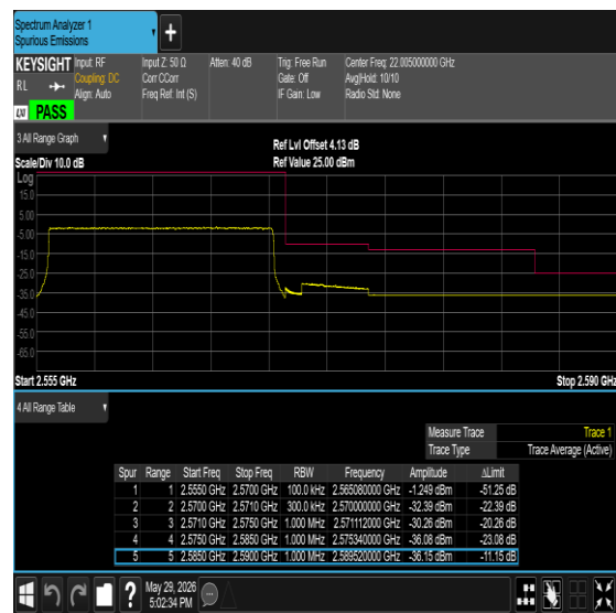
Band7-15MHz-16QAM-20825-75RB#0-PASS
