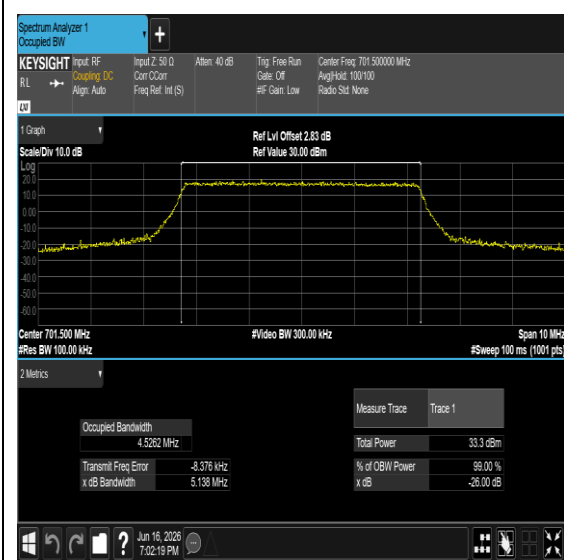
Band12-5MHz-QPSK-23035-25RB#0-PASS
