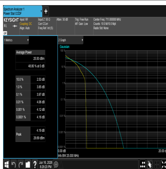
Band12-10MHz-QPSK-23130-1RB#0-PASS
