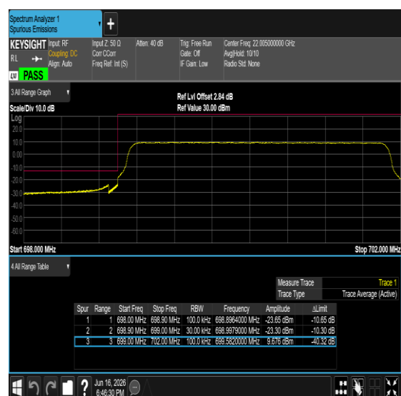
Band12-3MHz-64QAM-23165-15RB#0-PASS
