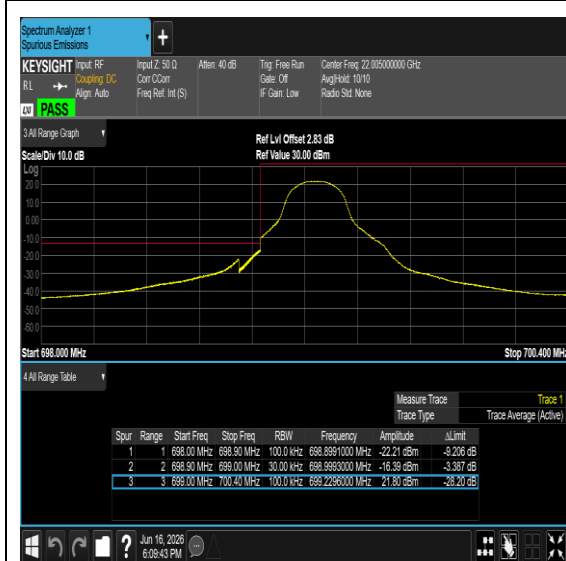
Band12-1.4MHz-16QAM-23017-1RB#0-PASS
