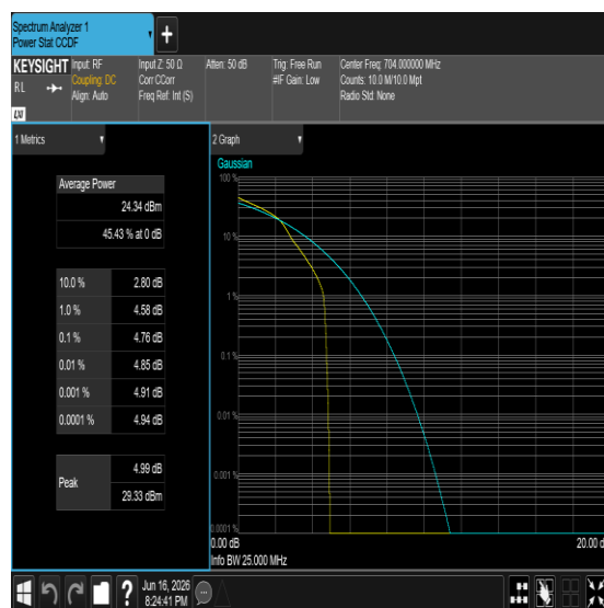
Band12-10MHz-16QAM-23095-1RB#0-PASS
