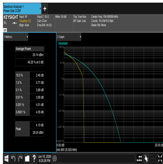
Band12-10MHz-64QAM-23095-1RB#0-PASS
