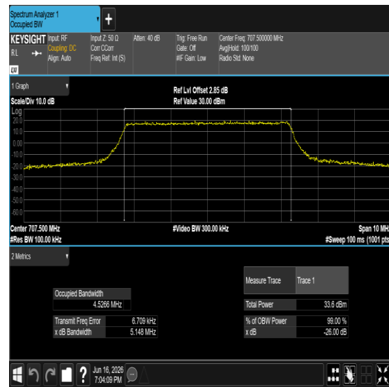
Band12-5MHz-16QAM-23035-25RB#0-PASS
