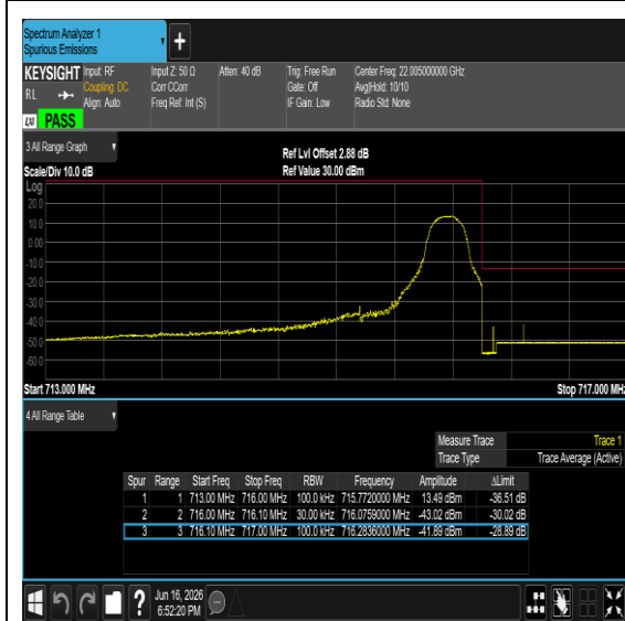
Band12-3MHz-64QAM-23165-1RB#14-PASS
