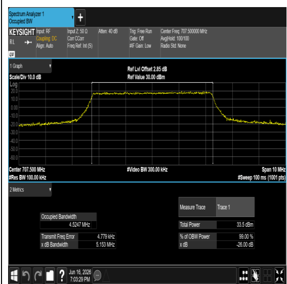
Band12-5MHz-QPSK-23095-25RB#0-PASS
