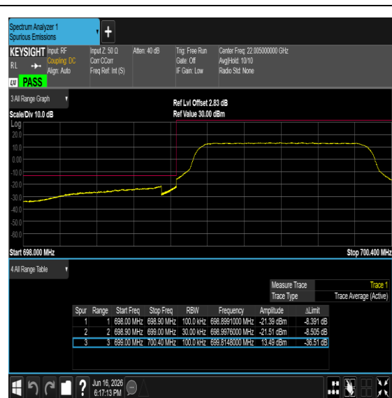
Band12-1.4MHz-64QAM-23173-6RB#0-PASS
