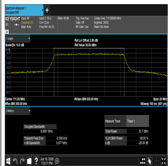
Band12-10MHz-QPSK-23130-50RB#0-PASS
