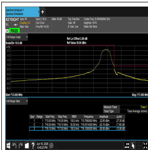
Band12-3MHz-64QAM-23025-1RB#0-PASS
