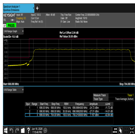
Band12-5MHz-64QAM-23035-25RB#0-PASS
