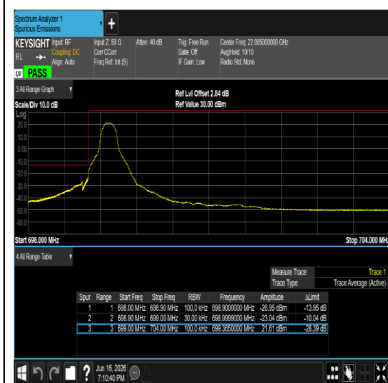
Band12-5MHz-64QAM-23035-1RB#0-PASS
