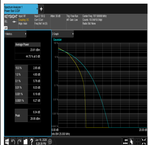
Band12-10MHz-16QAM-23095-50RB#0-PASS
