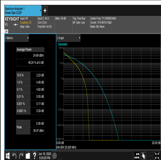
Band12-10MHz-QPSK-23130-50RB#0-PASS
