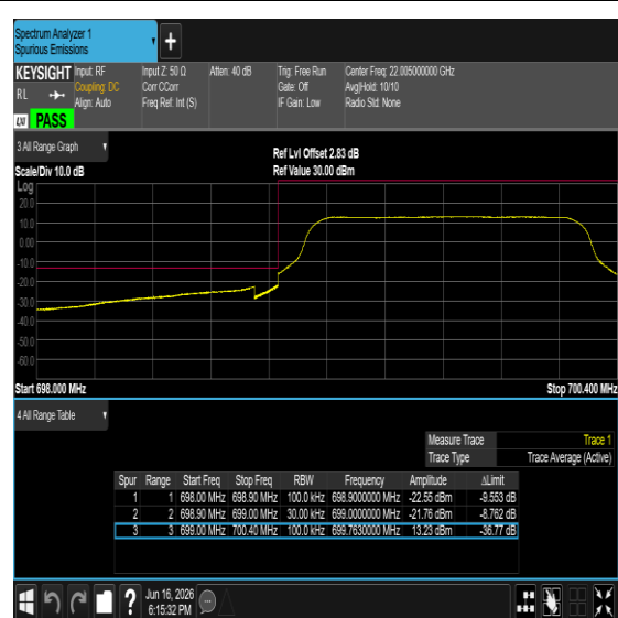
Band12-1.4MHz-16QAM-23017-6RB#0-PASS
