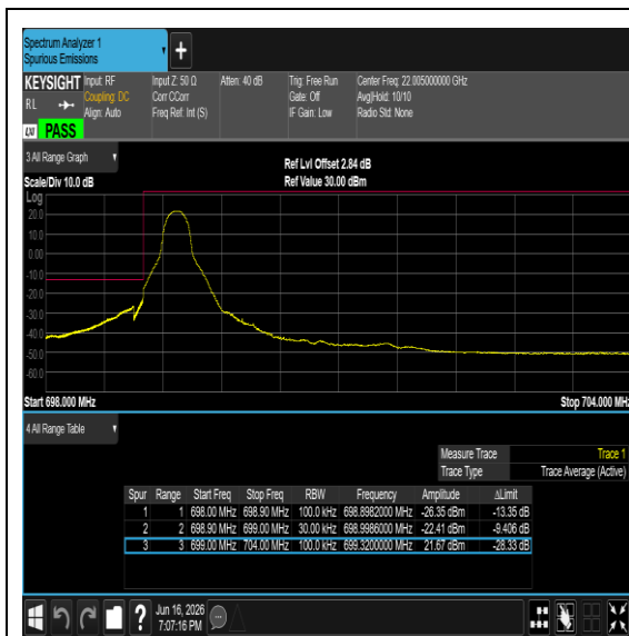
Band12-5MHz-QPSK-23155-1RB#24-PASS
