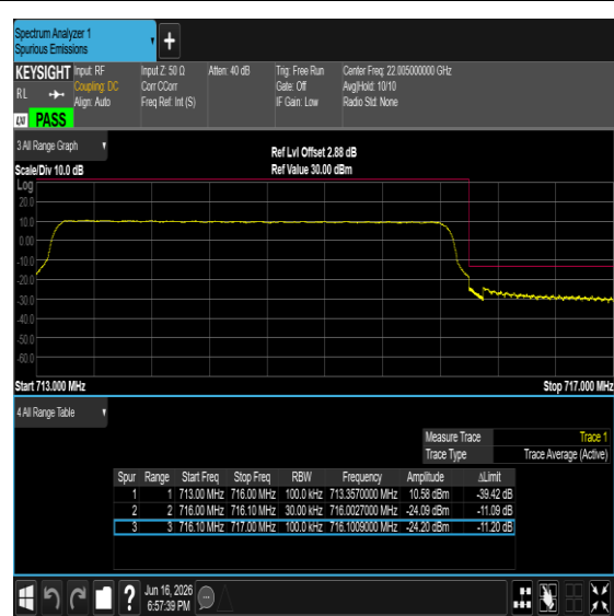
Band12-3MHz-64QAM-23165-15RB#0-PASS
