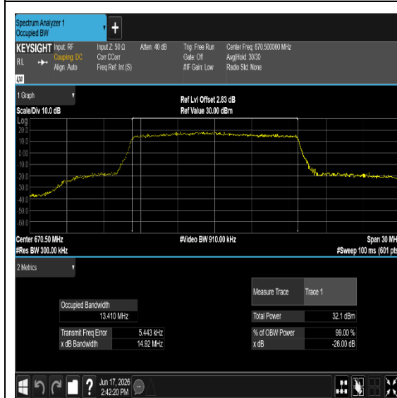
Band71-15MHz-QPSK-133197-75RB#0-PASS
