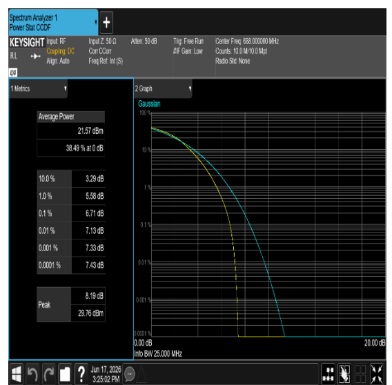
Band71-20MHz-QPSK-133372-100RB#0-PASS
