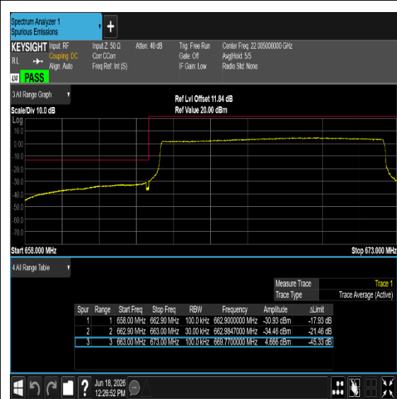
Band71-10MHz-QPSK-133172-50RB#0-PASS
