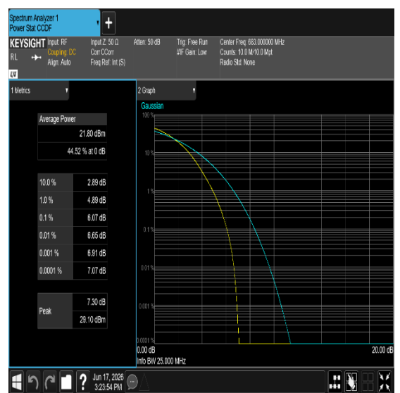
Band71-20MHz-16QAM-133322-100RB#0-PASS
