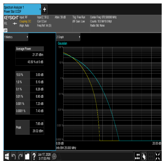
Band71-15MHz-16QAM-133197-75RB#0-PASS
