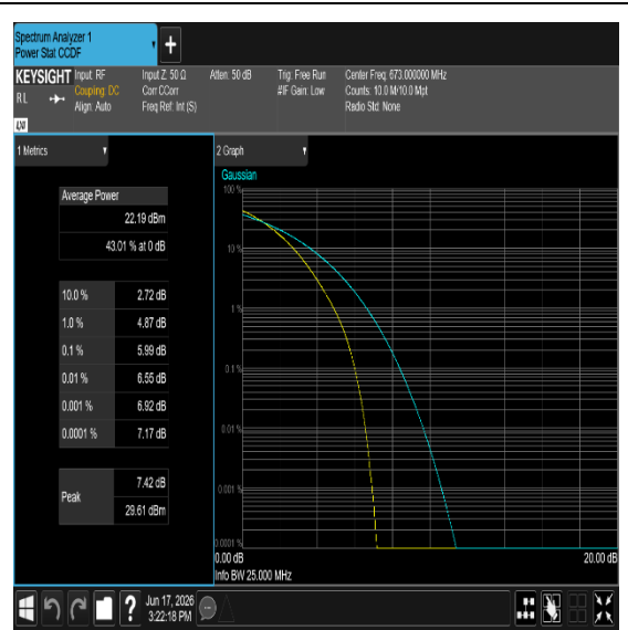
Band71-20MHz-QPSK-133322-100RB#0-PASS
