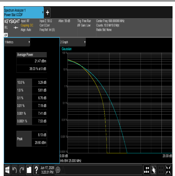
Band71-20MHz-16QAM-133222-100RB#0-PASS
