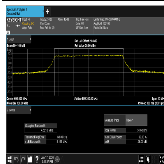
Band71-5MHz-16QAM-133447-25RB#0-PASS
