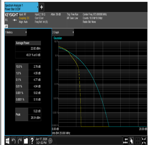
Band71-20MHz-16QAM-133322-1RB#0-PASS
