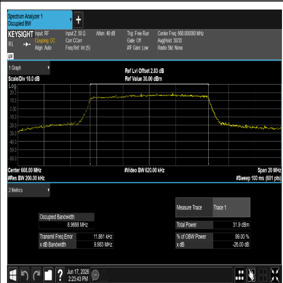
Band71-10MHz-QPSK-133172-50RB#0-PASS
