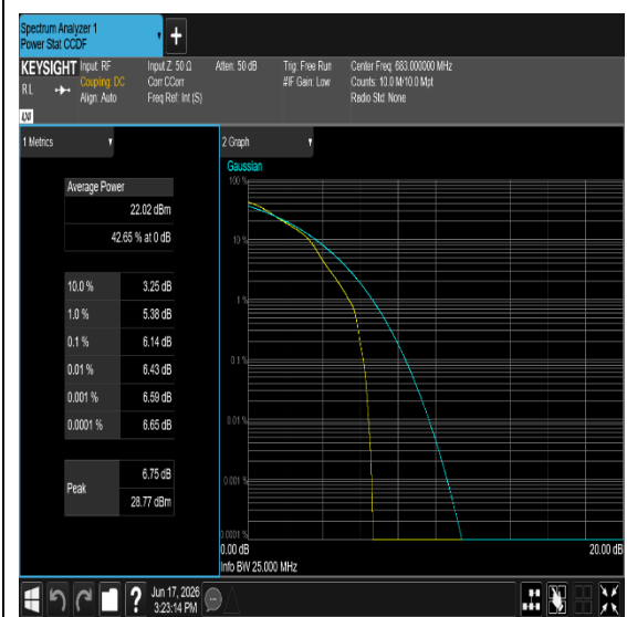
Band71-20MHz-16QAM-133322-1RB#0-PASS
