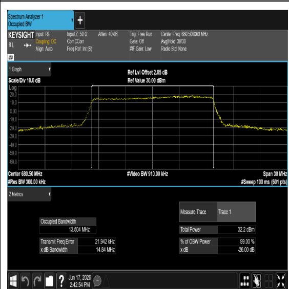
Band71-15MHz-QPSK-133297-75RB#0-PASS
