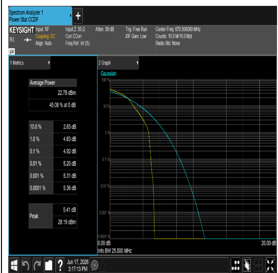
Band71-15MHz-16QAM-133197-1RB#0-PASS
