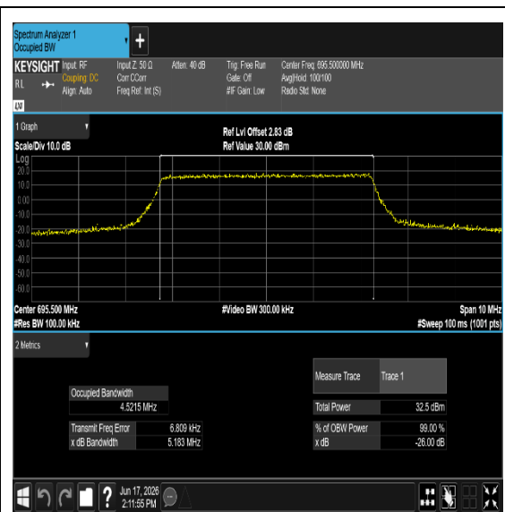
Band71-5MHz-16QAM-133297-25RB#0-PASS
