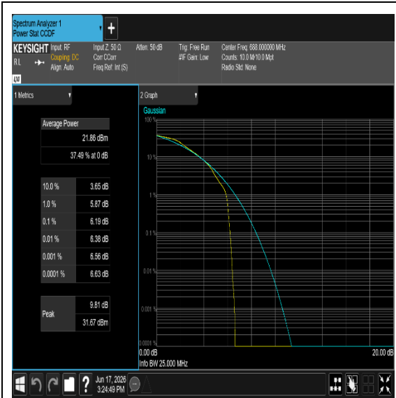
Band71-20MHz-16QAM-133222-1RB#0-PASS
