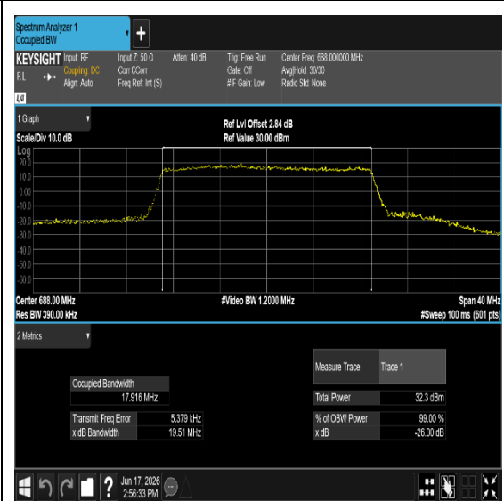
Band71-20MHz-QPSK-133372-100RB#0-PASS
