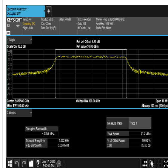
Band41-5MHz-16QAM-41565-25RB#0-PASS
