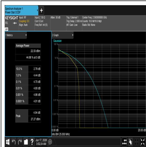
Band41-15MHz-64QAM-41515-1RB#0-PASS
