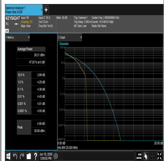
Band41-10MHz-64QAM-41540-1RB#0-PASS
