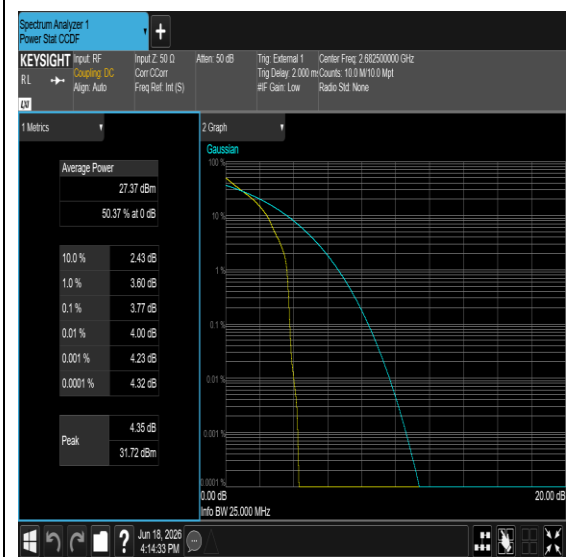
Band41-15MHz-16QAM-39725-1RB#0-PASS
