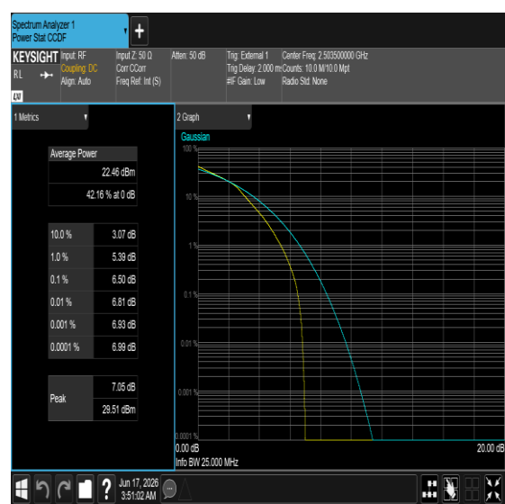
Band41-15MHz-16QAM-39725-75RB#0-PASS
