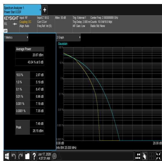
Band41-20MHz-16QAM-40620-100RB#0-PASS
