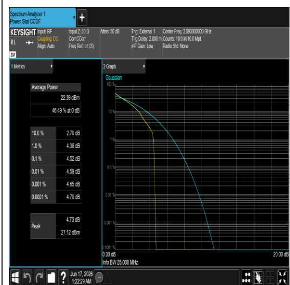
Band41-5MHz-64QAM-40620-1RB#0-PASS
