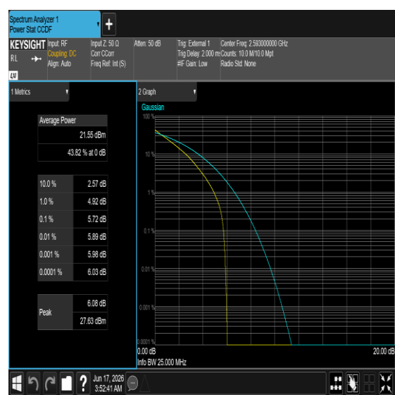
Band41-15MHz-QPSK-40620-75RB#0-PASS
