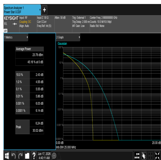
Band41-20MHz-QPSK-41490-100RB#0-PASS
