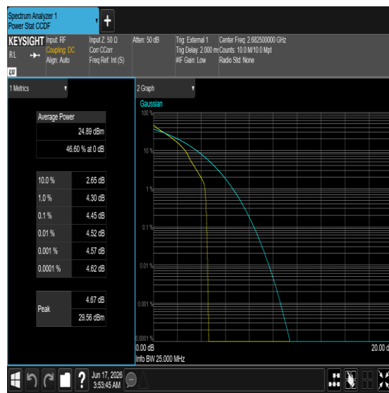
Band41-15MHz-64QAM-39725-1RB#0-PASS
