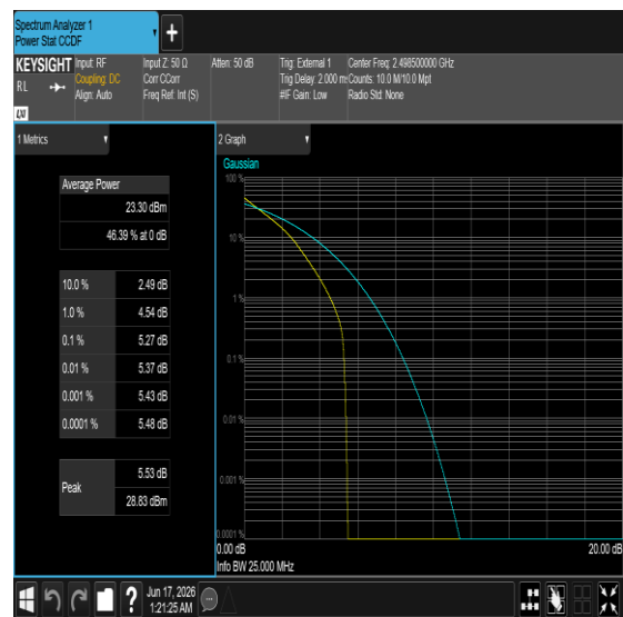
Band41-5MHz-64QAM-40620-25RB#0-PASS
