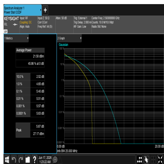
Band41-5MHz-64QAM-40620-25RB#0-PASS
