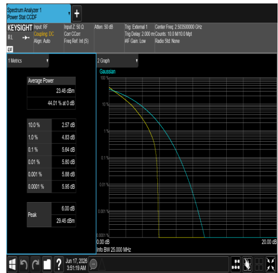
Band41-15MHz-64QAM-40620-75RB#0-PASS
