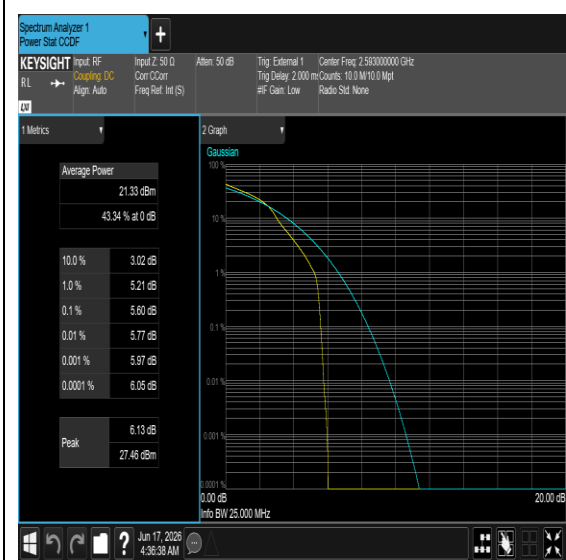
Band41-20MHz-16QAM-40620-1RB#0-PASS
