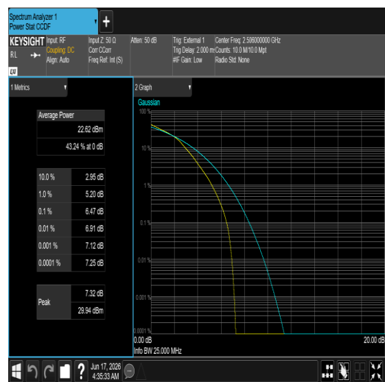
Band41-20MHz-16QAM-40620-100RB#0-PASS
