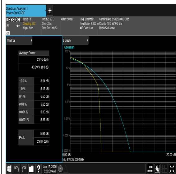
Band41-15MHz-16QAM-39725-1RB#0-PASS
