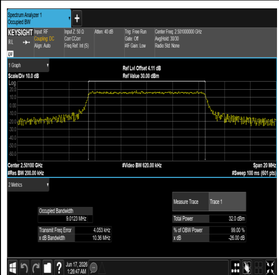
Band41-10MHz-QPSK-39700-50RB#0-PASS
