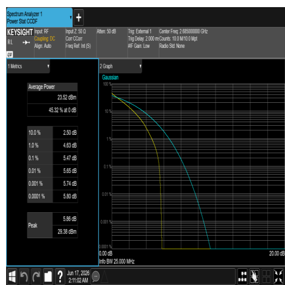
Band41-10MHz-64QAM-41540-50RB#0-PASS
