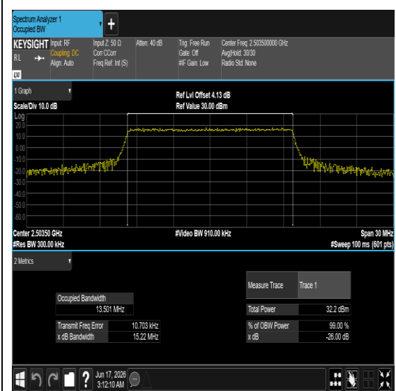
Band41-15MHz-QPSK-39725-75RB#0-PASS
