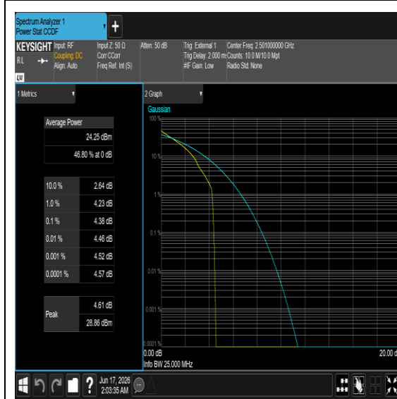
Band41-10MHz-QPSK-39700-1RB#0-PASS
