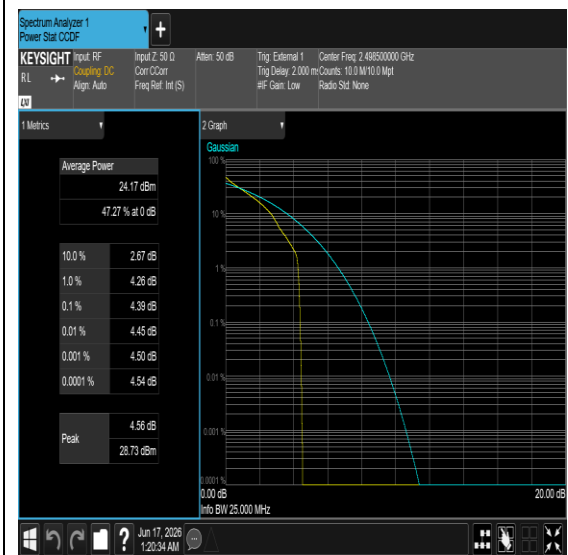
Band41-5MHz-64QAM-40620-1RB#0-PASS
