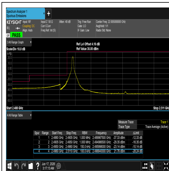
Band41-15MHz-QPSK-41515-1RB#74-PASS
