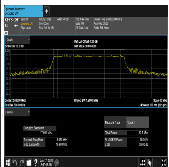
Band41-20MHz-QPSK-41490-100RB#0-PASS
