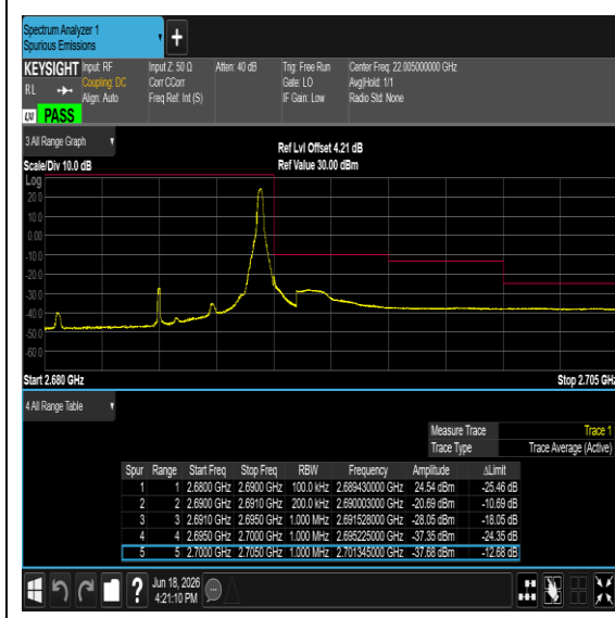
Band41-10MHz-64QAM-41540-1RB#49-PASS
