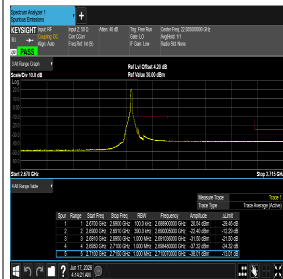
Band41-20MHz-16QAM-41490-1RB#99-PASS
