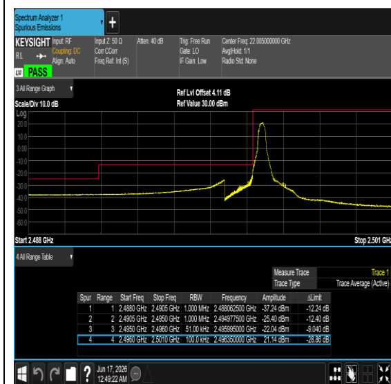
Band41-5MHz-16QAM-39675-1RB#0-PASS
