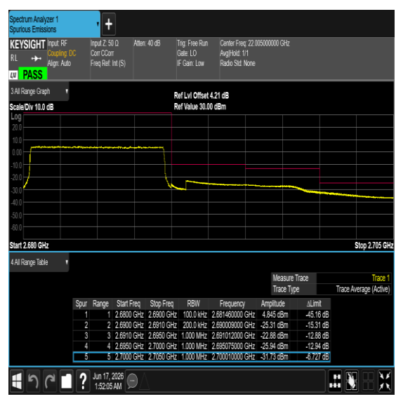
Band41-10MHz-64QAM-41540-50RB#0-PASS
