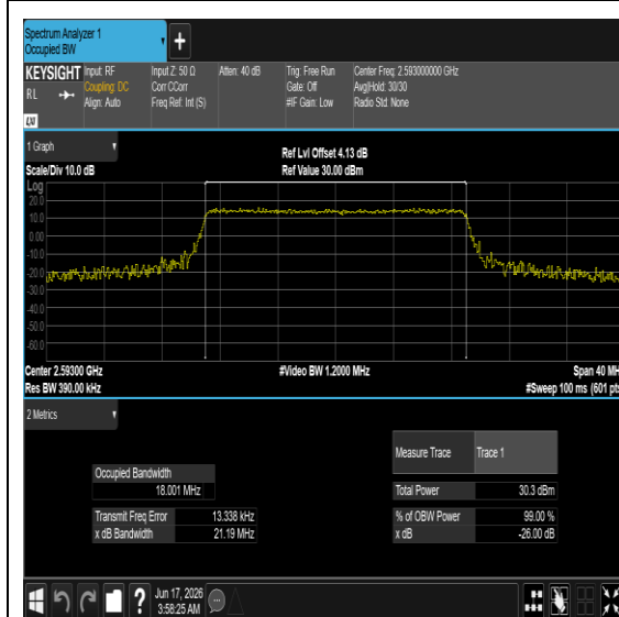
Band41-20MHz-QPSK-40620-100RB#0-PASS
