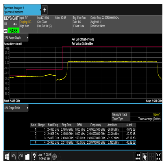
Band41-15MHz-64QAM-39725-75RB#0-PASS
