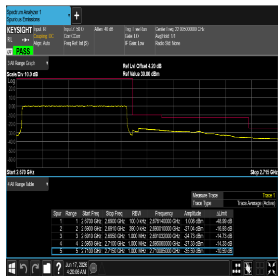
Band41-20MHz-16QAM-41490-100RB#0-PASS
