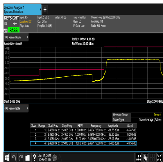
Band41-5MHz-16QAM-39675-25RB#0-PASS
