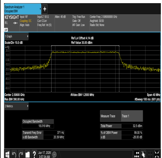
Band41-20MHz-QPSK-41490-100RB#0-PASS
