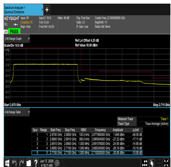
Band41-20MHz-QPSK-41490-100RB#0-PASS
