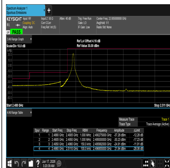
Band41-15MHz-64QAM-39725-1RB#0-PASS
