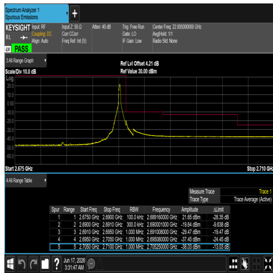
Band41-15MHz-16QAM-39725-1RB#0-PASS
