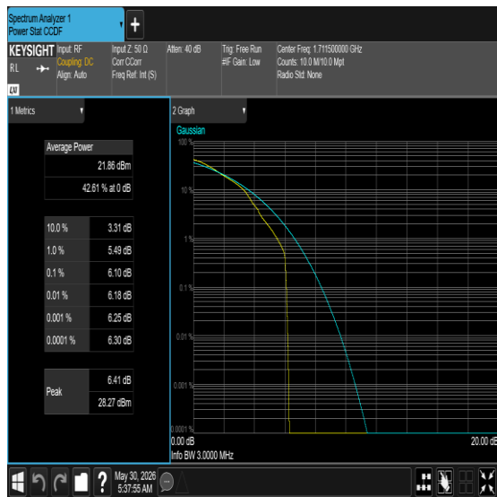
Band66-3MHz-16QAM-132322-1RB#0-PASS
