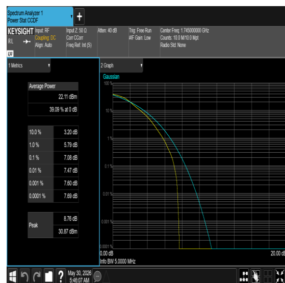
Band66-5MHz-QPSK-132322-25RB#0-PASS
