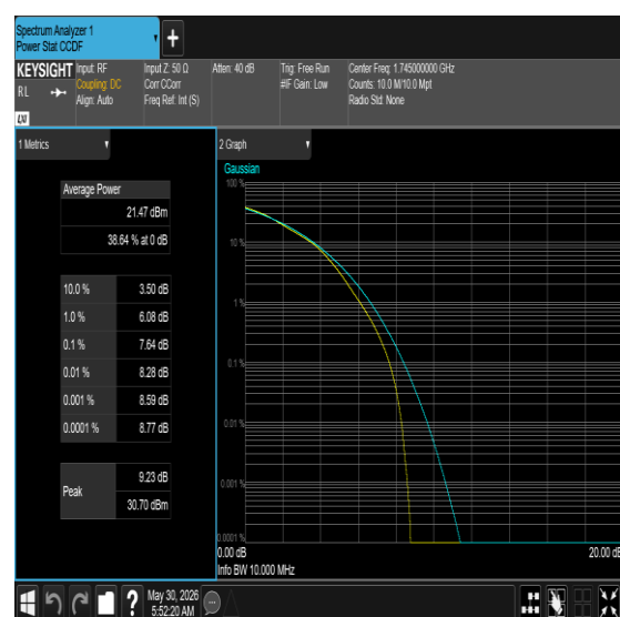
Band66-10MHz-16QAM-132322-50RB#0-PASS
