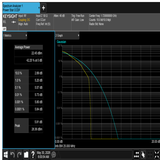
Band66-20MHz-QPSK-132322-1RB#0-PASS
