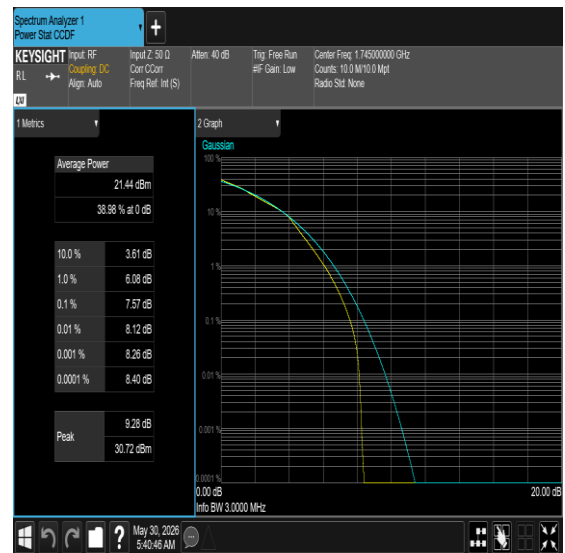
Band66-3MHz-16QAM-132657-15RB#0-PASS
