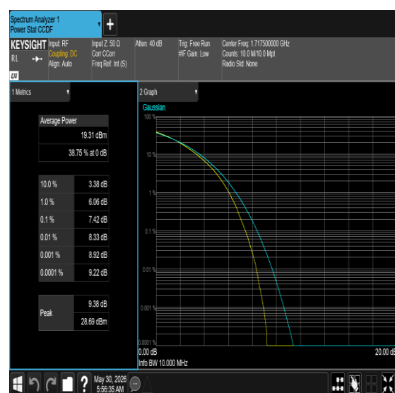
Band66-15MHz-64QAM-132047-75RB#0-PASS
