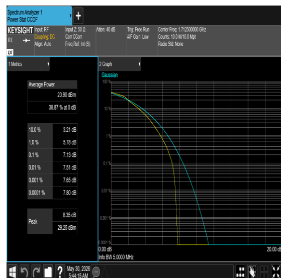
Band66-5MHz-QPSK-132322-25RB#0-PASS
