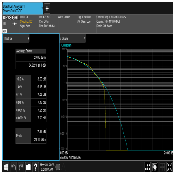
Band66-1.4MHz-16QAM-132322-1RB#0-PASS
