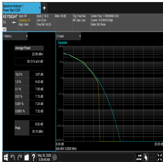
Band66-3MHz-16QAM-132657-1RB#0-PASS
