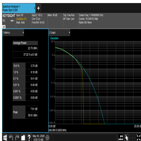
Band66-5MHz-QPSK-132322-1RB#0-PASS
