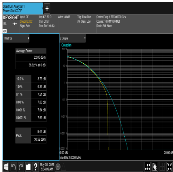
Band66-1.4MHz-16QAM-131979-1RB#0-PASS
