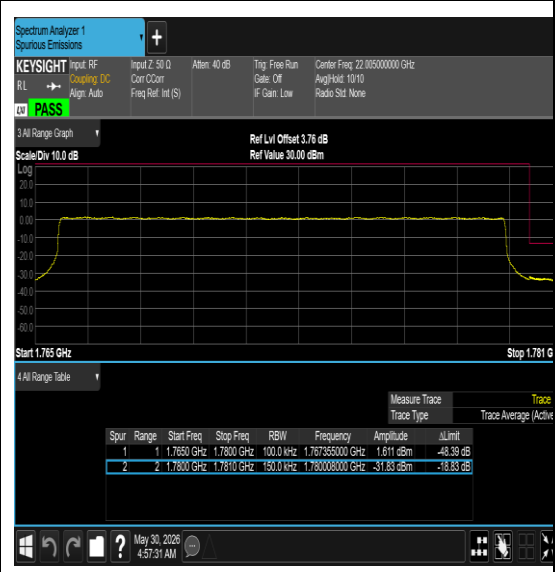
Band66-15MHz-16QAM-132597-75RB#0-PASS
