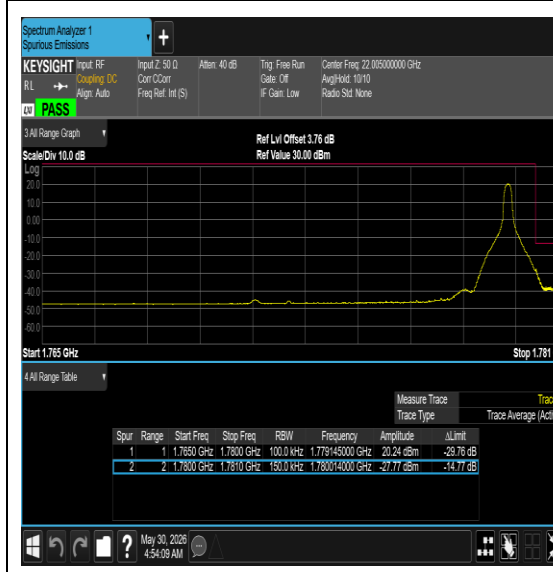
Band66-15MHz-16QAM-132597-1RB#74-PASS
