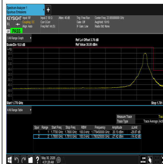
Band66-15MHz-QPSK-132047-1RB#0-PASS
