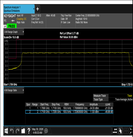
Band66-15MHz-QPSK-132047-75RB#0-PASS
