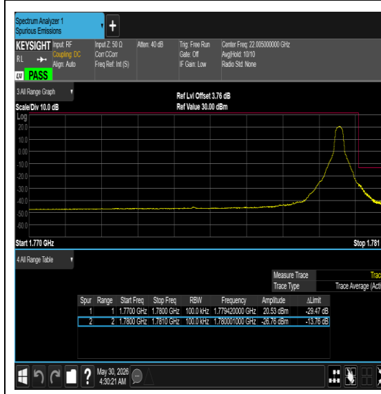
Band66-10MHz-QPSK-132622-1RB#49-PASS
