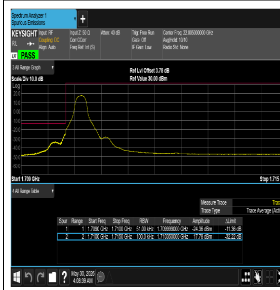
Band66-5MHz-64QAM-131997-1RB#0-PASS
