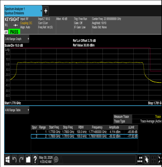
Band66-10MHz-QPSK-132622-50RB#0-PASS
