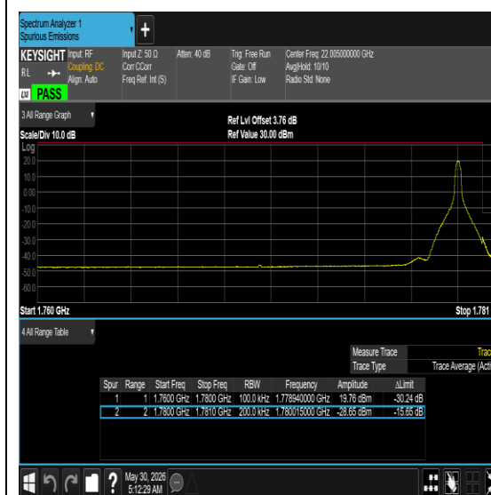
Band66-20MHz-16QAM-132072-1RB#0-PASS
