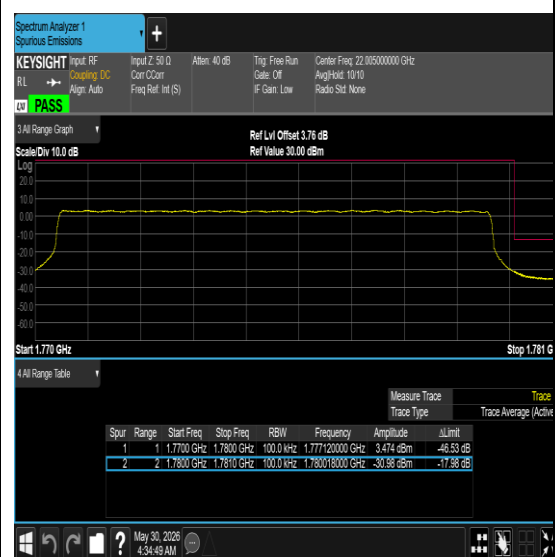
Band66-15MHz-QPSK-132047-75RB#0-PASS
