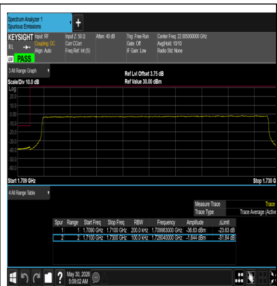
Band66-20MHz-64QAM-132572-100RB#0-PASS
