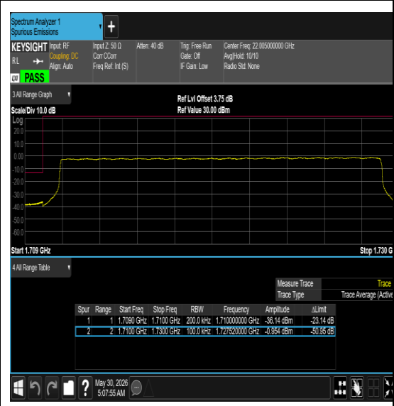
Band66-20MHz-16QAM-132072-100RB#0-PASS
