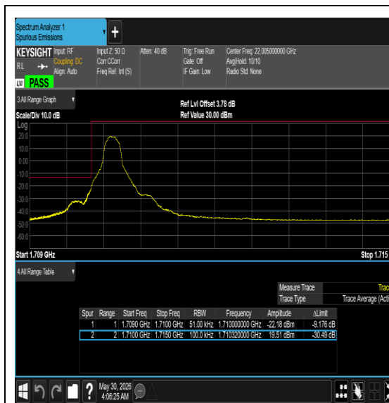
Band66-5MHz-QPSK-132647-1RB#24-PASS
