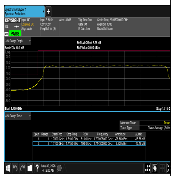
Band66-5MHz-64QAM-131997-25RB#0-PASS
