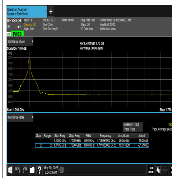
Band66-20MHz-16QAM-132072-1RB#0-PASS
