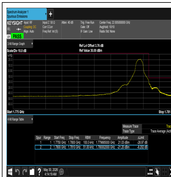
Band66-10MHz-QPSK-132022-1RB#0-PASS
