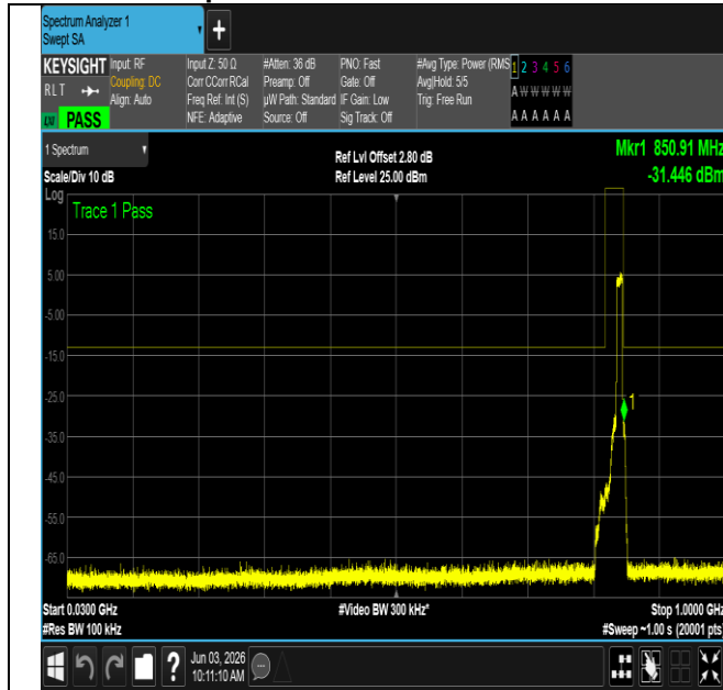
NTNV-n26(824-849)-PC3-15-10-H-DFT-QPSK- Edge 1RB Left-3000-12000-PASS
