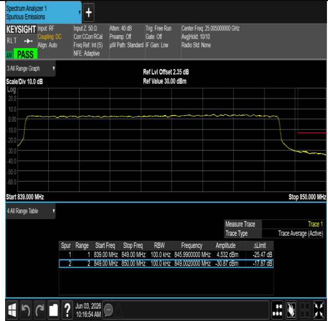
NTNV-n26(824-849)-PC3-15-15-L-DFT-QPSK-Outer_Full-PASS
