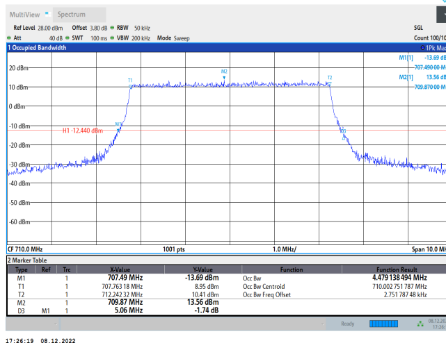
Band17-5MHz-QPSK-23790-25RB#0
