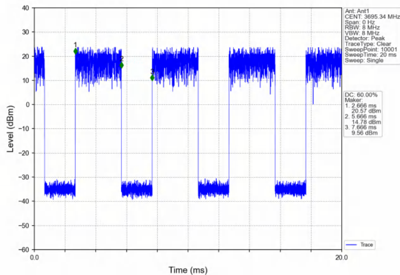
Band48_5MHz_16QAM_HCH_3697.5MHz_RB_1_0_NTNV
