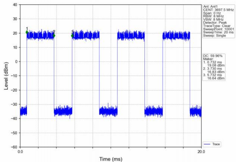
Band48_5MHz_256QAM_HCH_3697.5MHz_RB_25_0_NTNV
