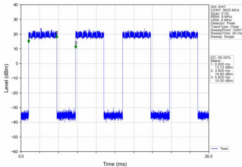
Band48_10MHz_64QAM_MCH_3625MHz_RB_50_0_NTNV
