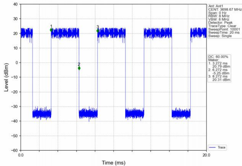
Band48_5MHz_16QAM_HCH_3697.5MHz_RB_25_0_NTNV
