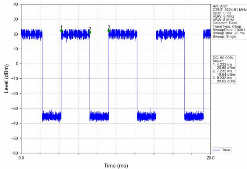
Band48_5MHz_16QAM_MCH_3625MHz_RB_12_13_NTNV
