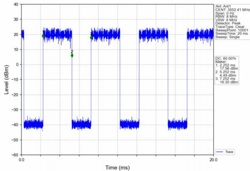
Band48_5MHz_64QAM_LCH_3552.5MHz_RB_12_13_NTNV
