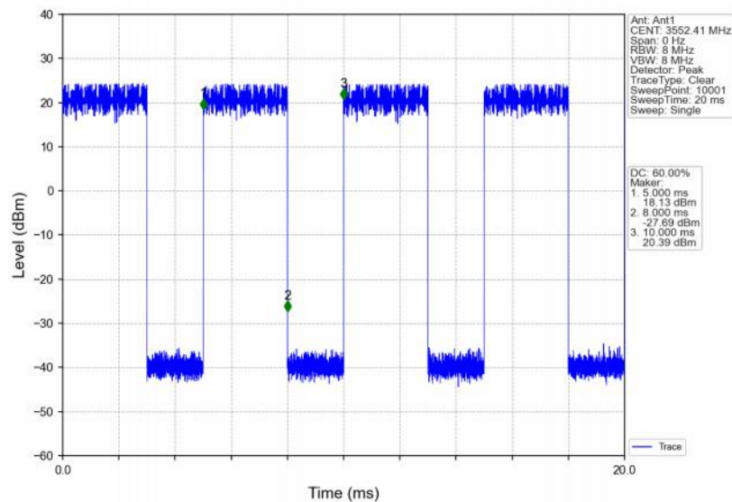
Band48_5MHz_16QAM_LCH_3552.5MHz_RB_12_6_NTNV
