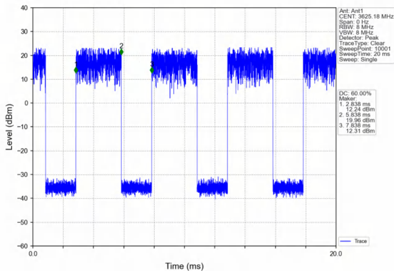
Band48_5MHz_16QAM_MCH_3625MHz_RB_1_13_NTNV
