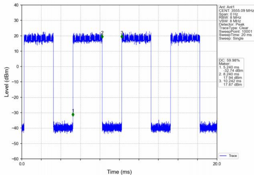
Band48_10MHz_256QAM_LCH_3555MHz_RB_25_13_NTNV
