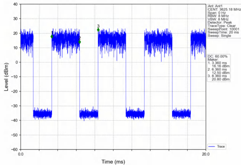
Band48_5MHz_64QAM_MCH_3625MHz_RB_1_24_NTNV
