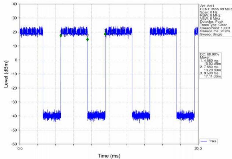
Band48_10MHz_64QAM_LCH_3555MHz_RB_25_25_NTNV
