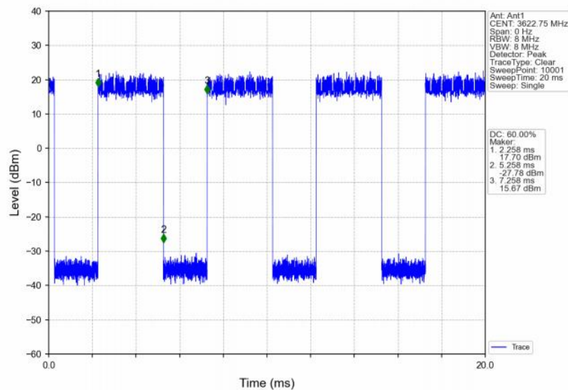
Band48_10MHz_256QAM_MCH_3625MHz_RB_25_0_NTNV
