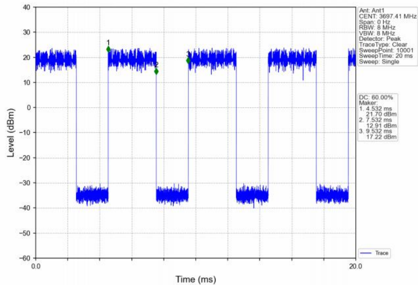
Band48_5MHz_64QAM_HCH_3697.5MHz_RB_12_13_NTNV
