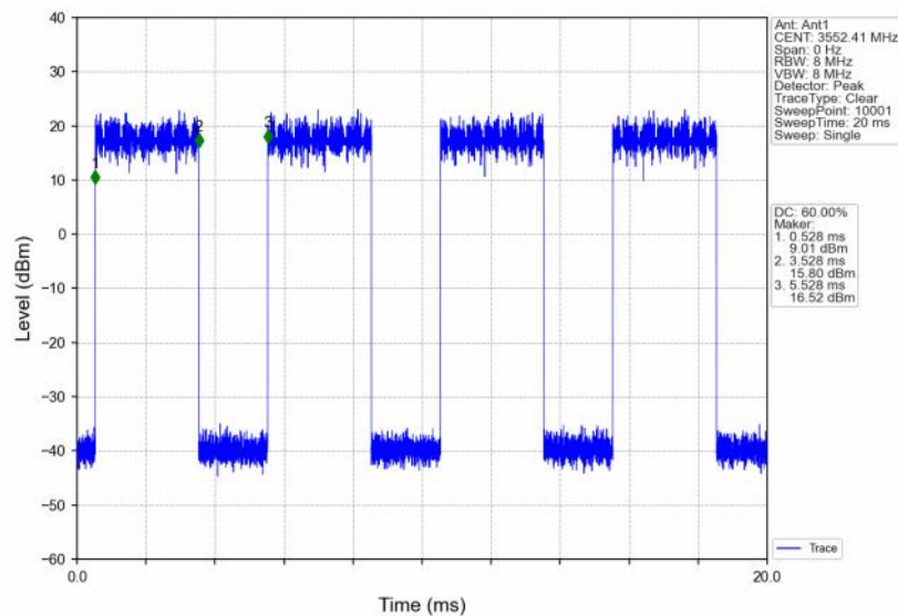
Band48_5MHz_256QAM_LCH_3552.5MHz_RB_12_6_NTNV
