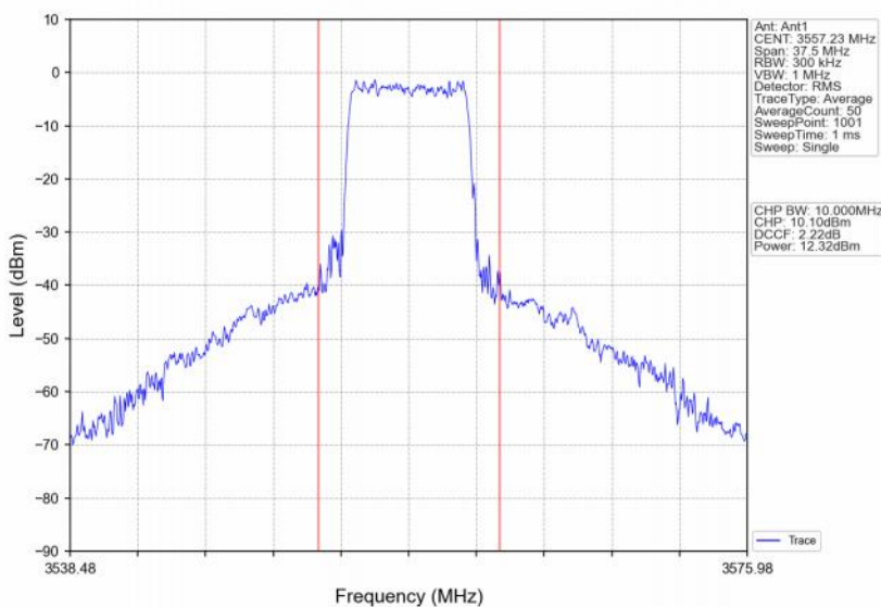
Band48_15MHz_256QAM_LCH_3557.5MHz_RB_36_18_NTNV
