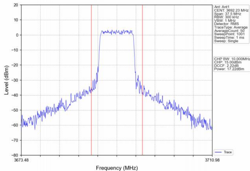
Band48_15MHz_16QAM_HCH_3692.5MHz_RB_36_18_NTNV
