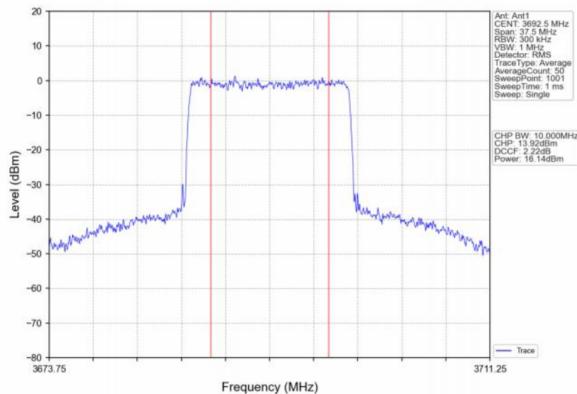
Band48_15MHz_16QAM_HCH_3692.5MHz_RB_75_0_NTNV
