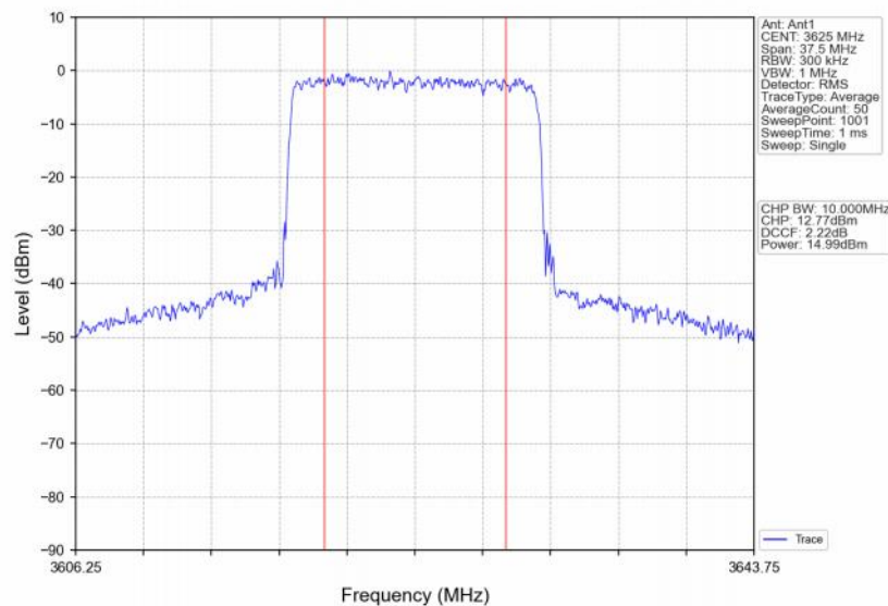
Band48_15MHz_64QAM_MCH_3625MHz_RB_75_0_NTNV
