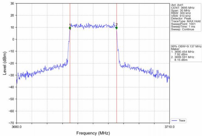
Band48_10MHz_16QAM_HCH_3695MHz_RB_50_0_NTNV
