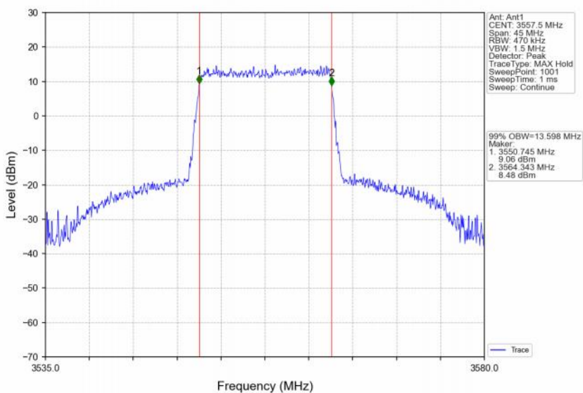
Band48_15MHz_256QAM_LCH_3557.5MHz_RB_75_0_NTNV
