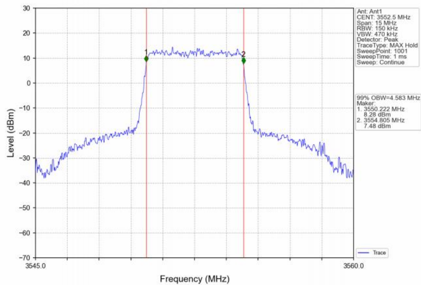
Band48_5MHz_256QAM_LCH_3552.5MHz_RB_25_0_NTNV
