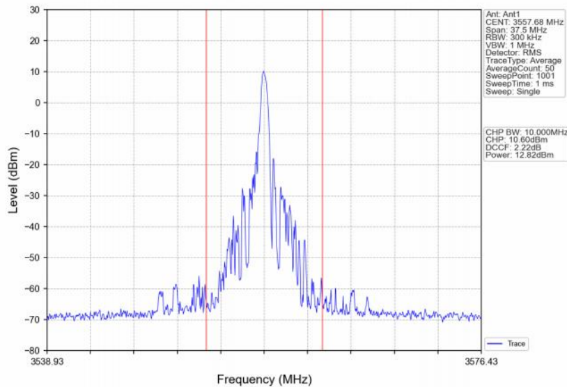
Band48_15MHz_256QAM_LCH_3557.5MHz_RB_1_74_NTNV
