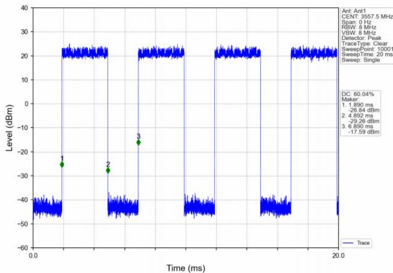
Band48_15MHz_256QAM_LCH_3557.5MHz_RB_75_0_NTNV
