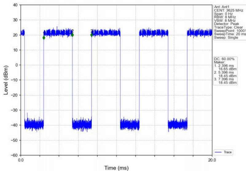
Band48_20MHz_64QAM_MCH_3625MHz_RB_100_0_NTNV
