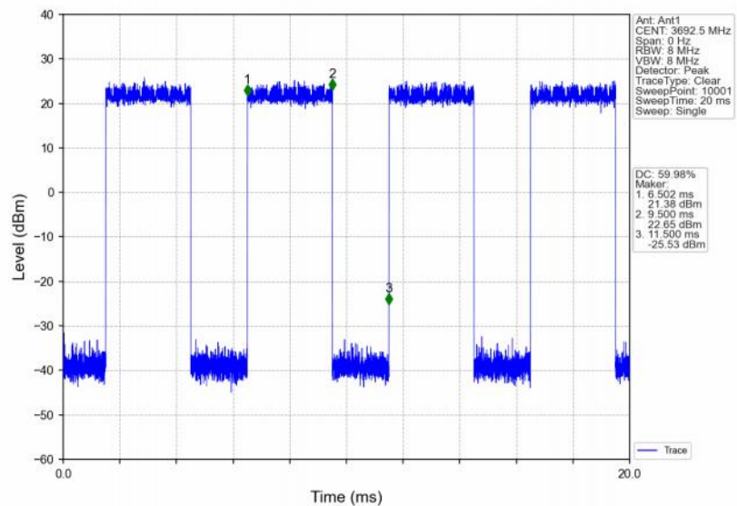
Band48_15MHz_256QAM_HCH_3692.5MHz_RB_75_0_NTNV
