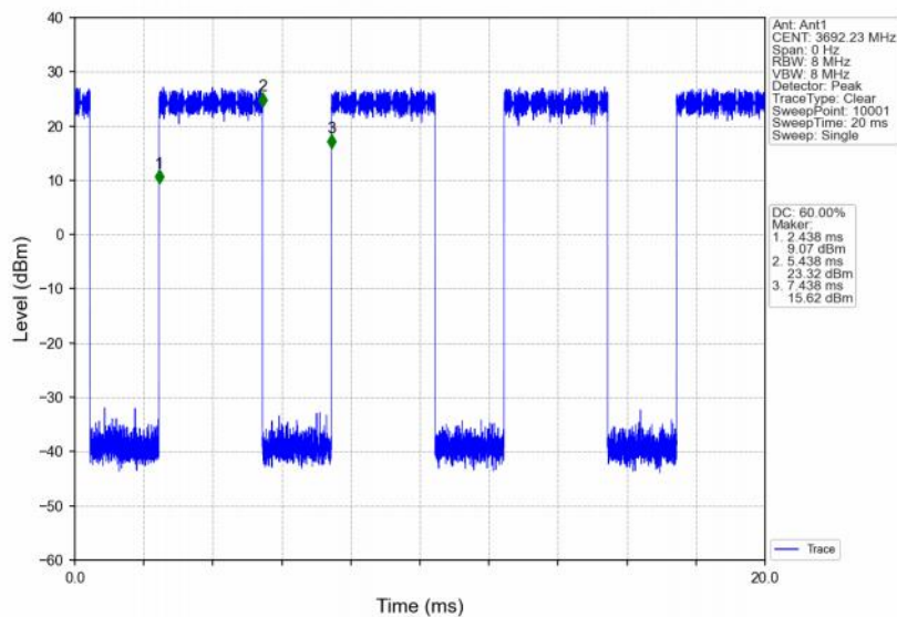
Band48_15MHz_16QAM_HCH_3692.5MHz_RB_36_18_NTNV
