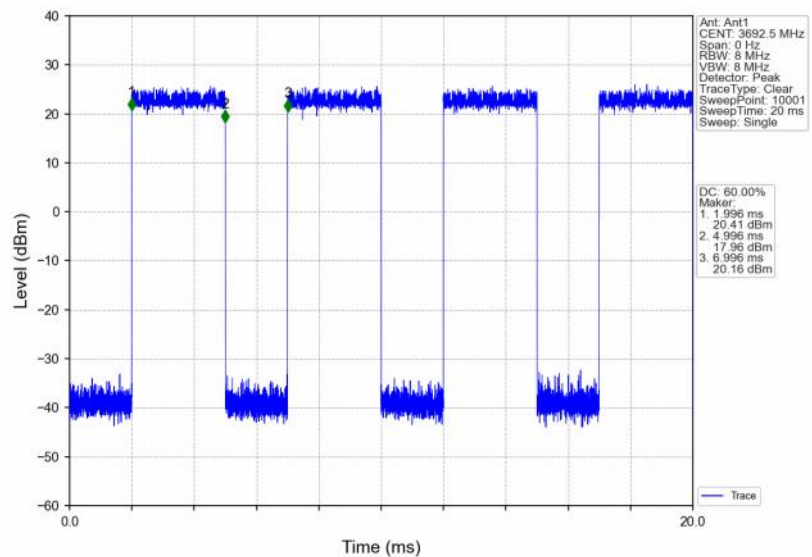
Band48_15MHz_16QAM_HCH_3692.5MHz_RB_75_0_NTNV
