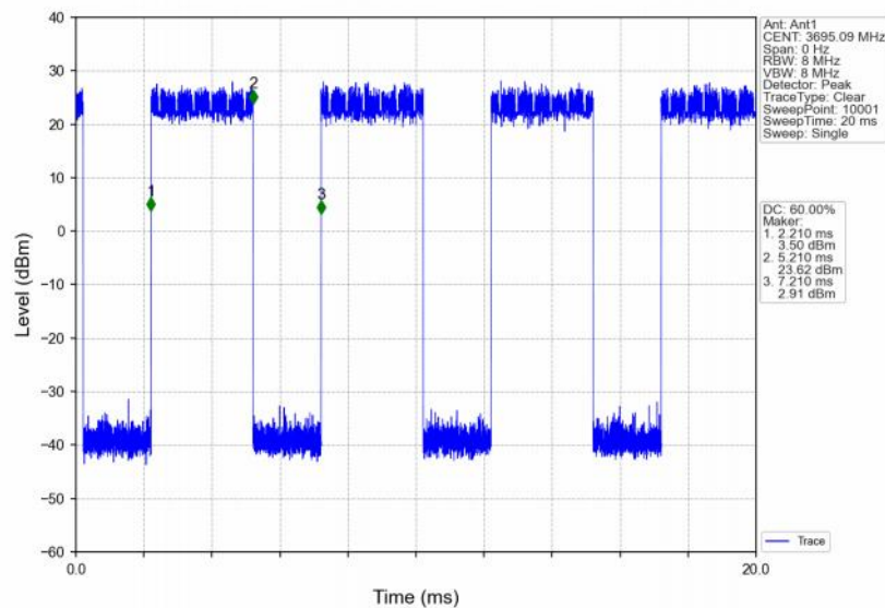
Band48_10MHz_256QAM_HCH_3695MHz_RB_25_13_NTNV
