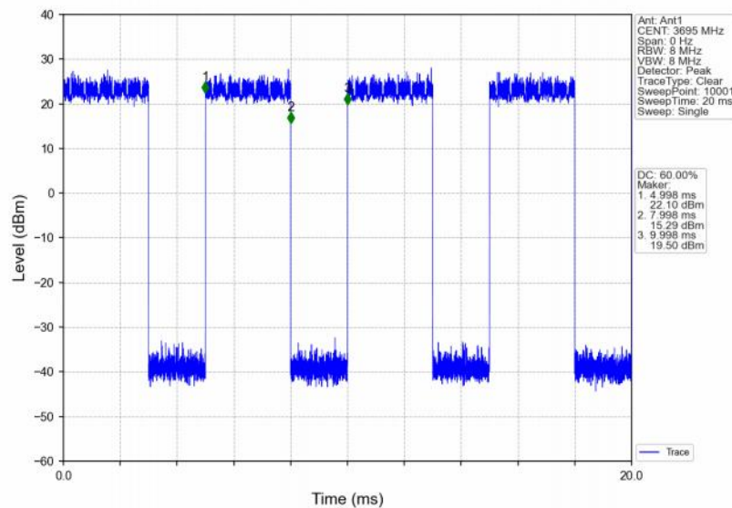
Band48_10MHz_256QAM_HCH_3695MHz_RB_50_0_NTNV
