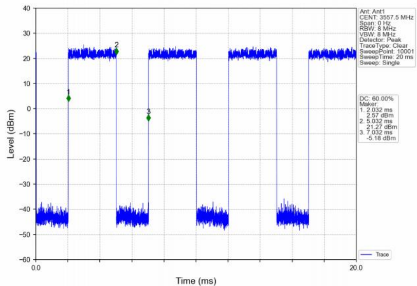
Band48_15MHz_16QAM_LCH_3557.5MHz_RB_75_0_NTNV
