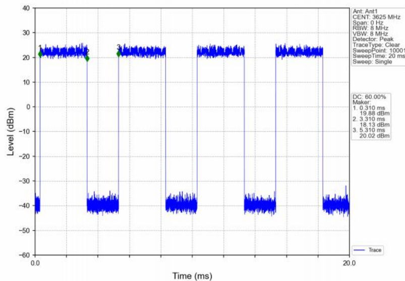
Band48_15MHz_64QAM_MCH_3625MHz_RB_75_0_NTNV
